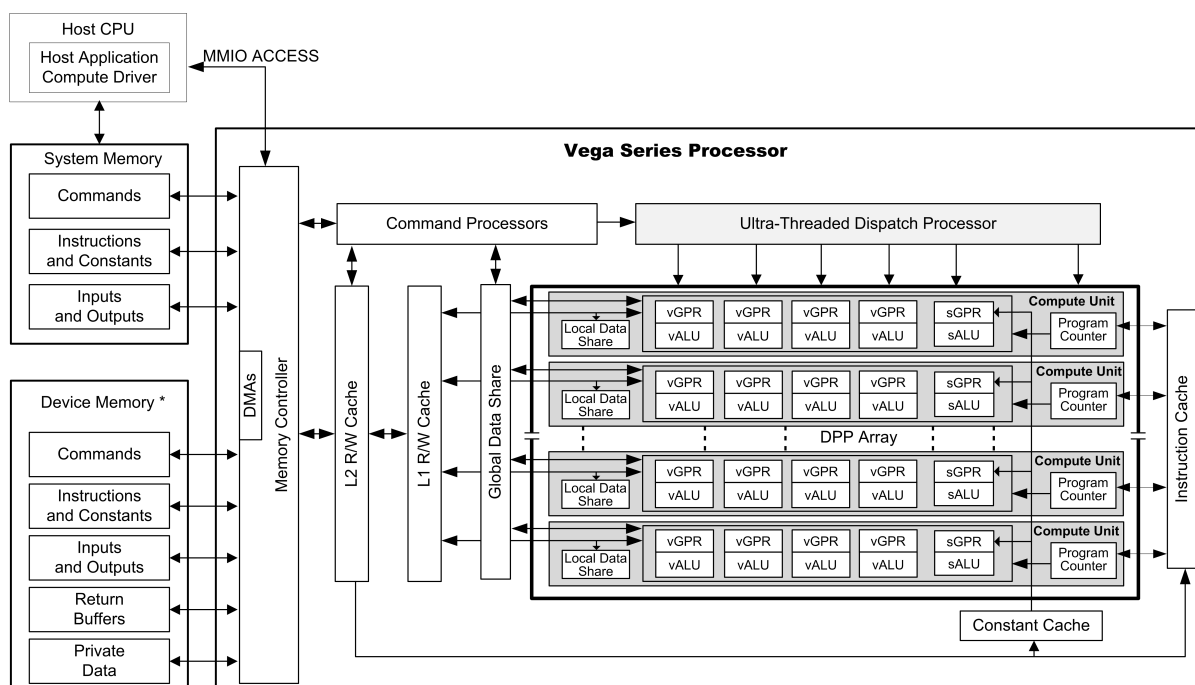
Figure 1. AMD GCN Vega Generation Series Block Diagram
