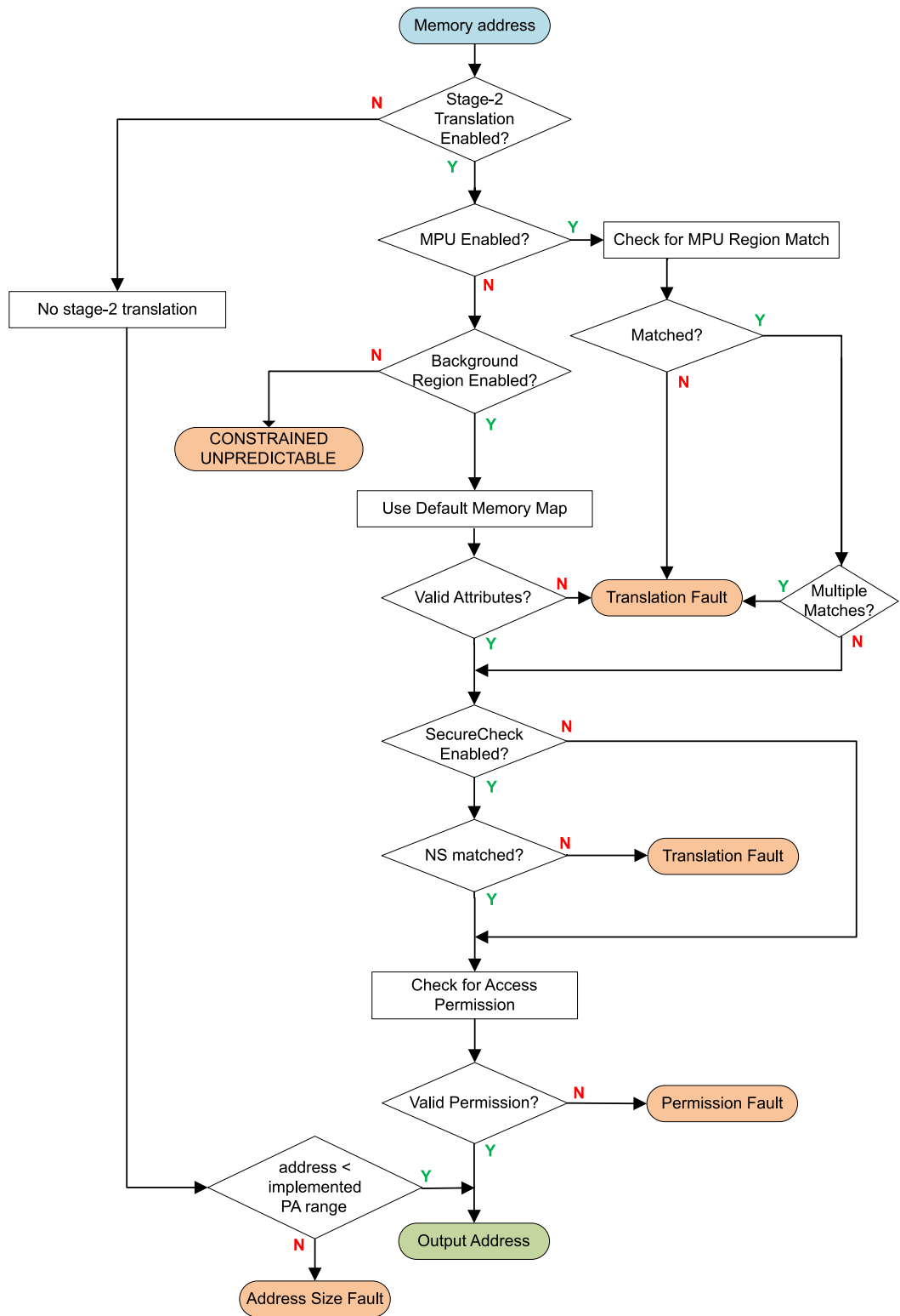
Figure D6-3 MPU fault check sequence for the stage 2 Secure EL1&0 translation
