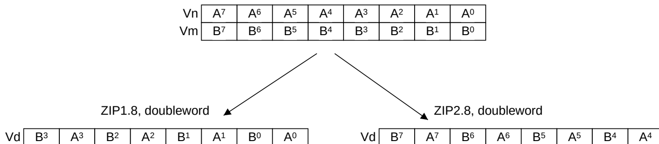
Figure C7-10 ZIP1 and ZIP2 with the arrangement specifier 8B
