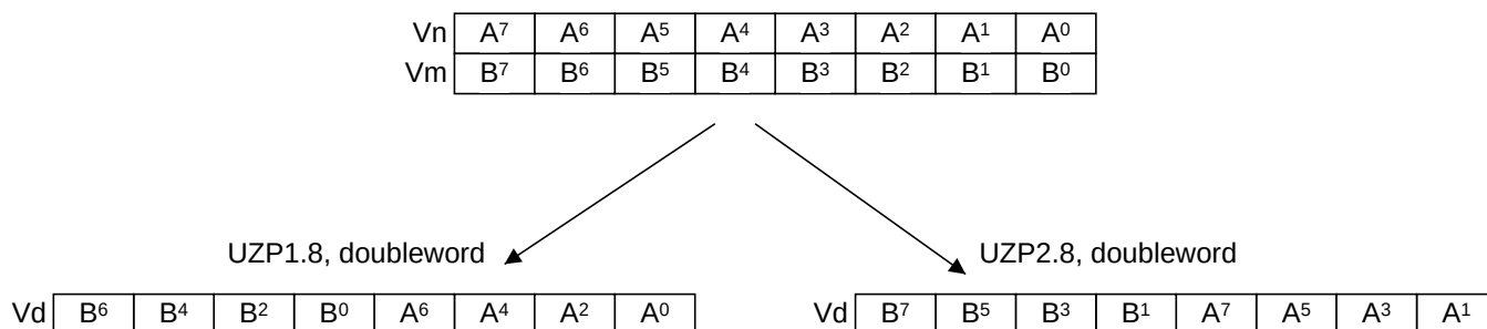
Figure C7-8 UZP1 and UZP2 with the arrangement specifier 8B
