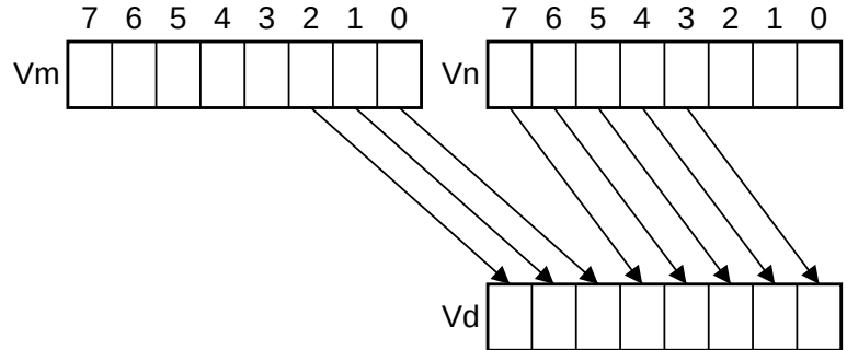
Figure C7-1 EXT doubleword operation for Q = 0 and imm4<2:0> = 3
