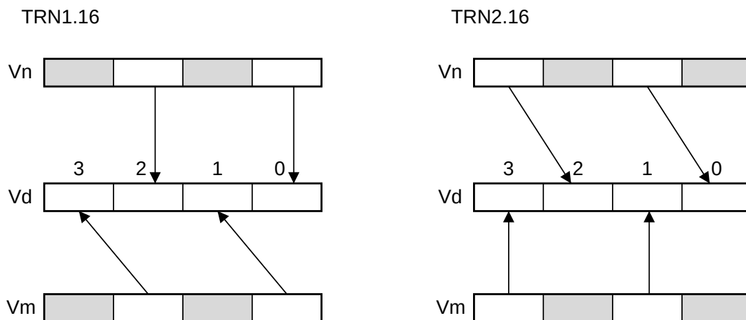
Figure C7-5 TRN1 and TRN2 halfword operations where Q = 0
