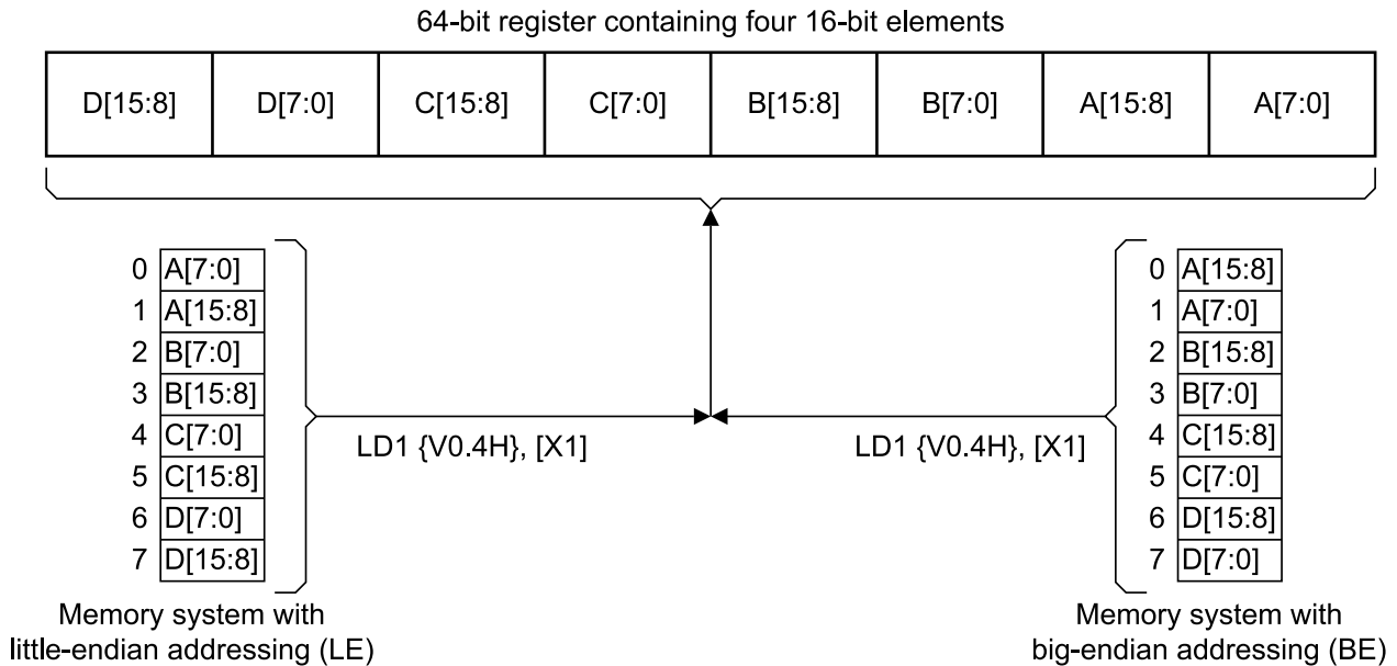
Figure B2-3 SIMD byte order example
