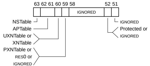
Figure D5-7 Stage 1 next-level attribute fields in a VMSAv8-64 Table descriptor
