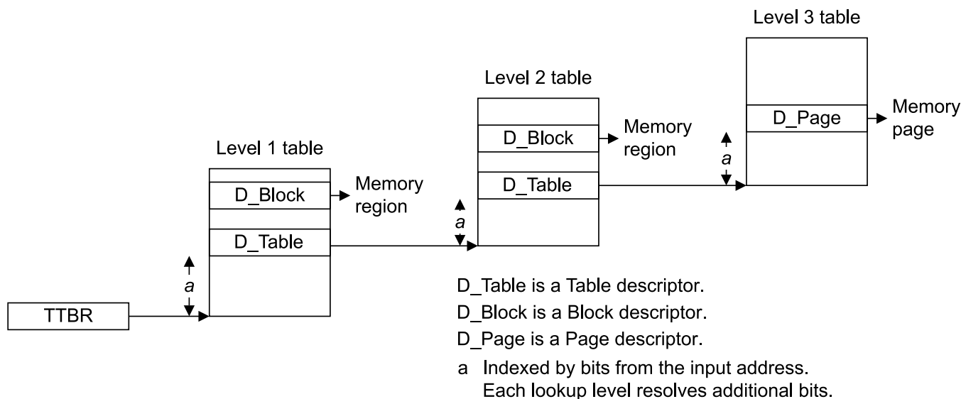
Figure D5-1 Generalized view of a single address translation stage
