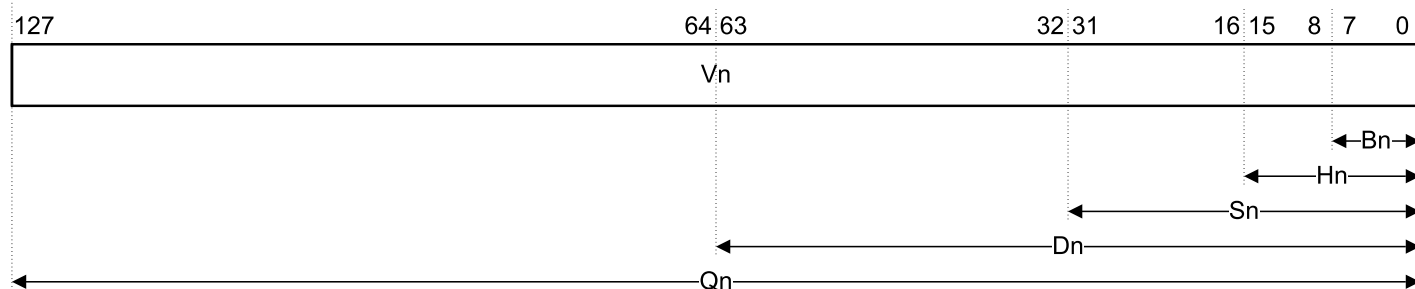
Figure B1-2 SIMD and floating-point register naming
