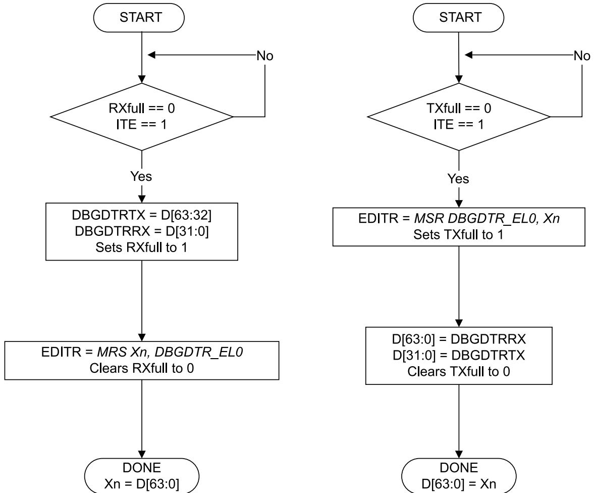
Figure E2-3 Reading and writing general-purpose registers, other than SP, in Debug state in AArch64 state
