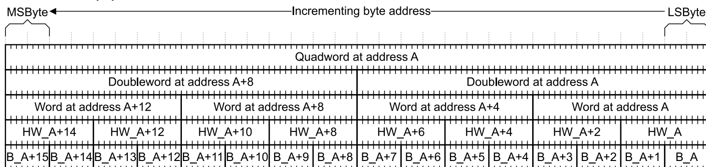
Figure B2-2 Endianness relationships
