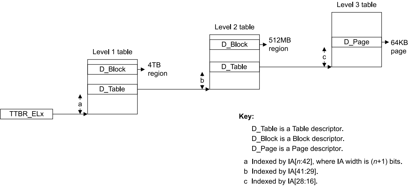
Figure D5-5 Generalized view of a stage 1 address translation using the 64KB granule
