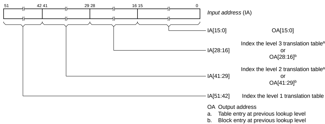
Figure D5-4 52-bit IA resolved using 64KB translation granule
