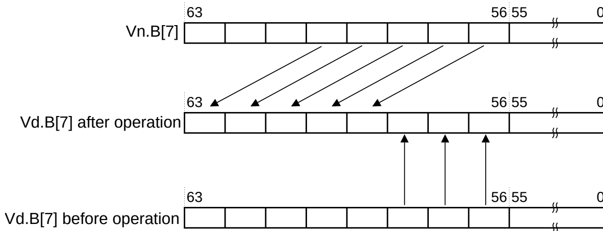
Figure C7-3 shift left by 3 for an 8-bit vector element
