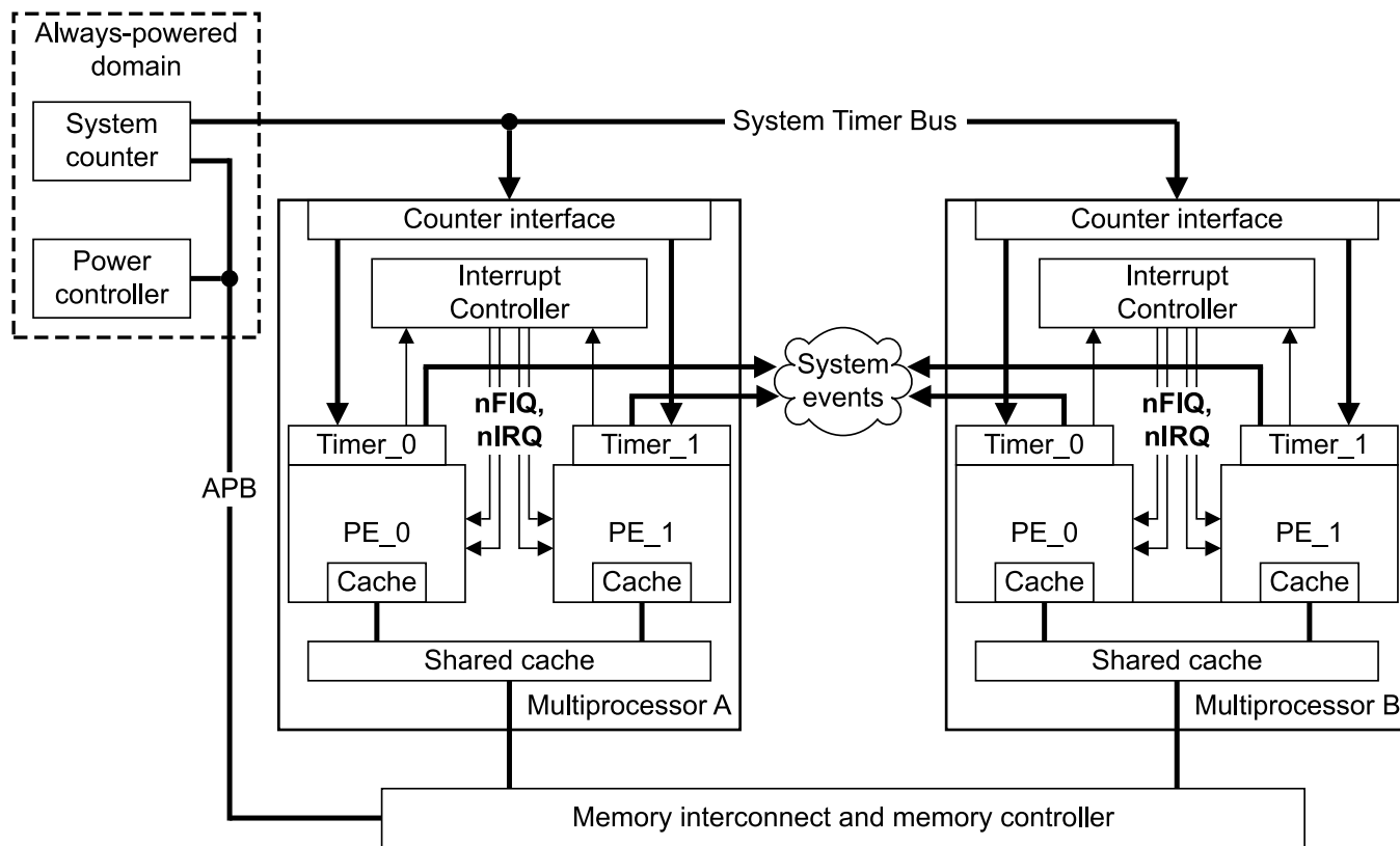
Figure D7-1 Generic Timer example
