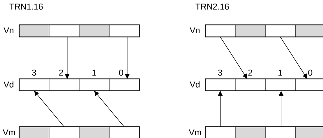
Figure C7-6 TRN1 and TRN2 halfword operations where Q = 0
