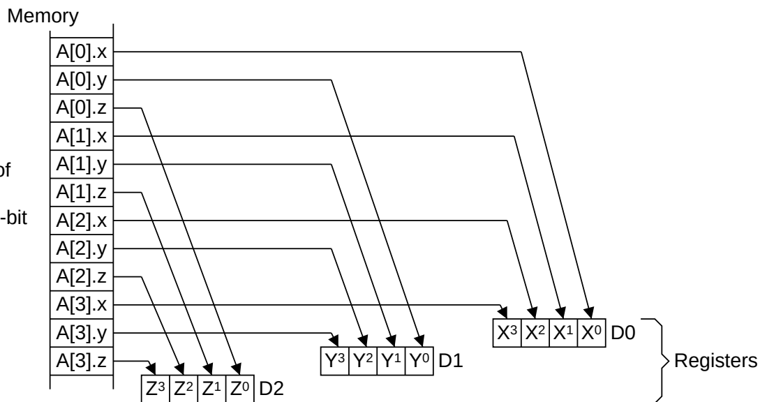
Figure C7-2 de-interleaving of an LD3.16 (multiple 3-element structures) instruction
