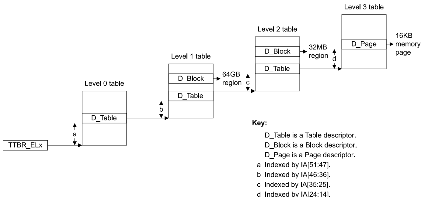
Figure D5-3 Generalized view of a stage 1 address translation using the 16KB granule
