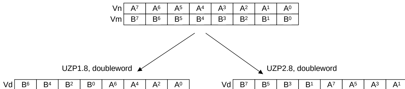
Figure C7-7 UZP1 and UZP2 with the arrangement specifier 8B
