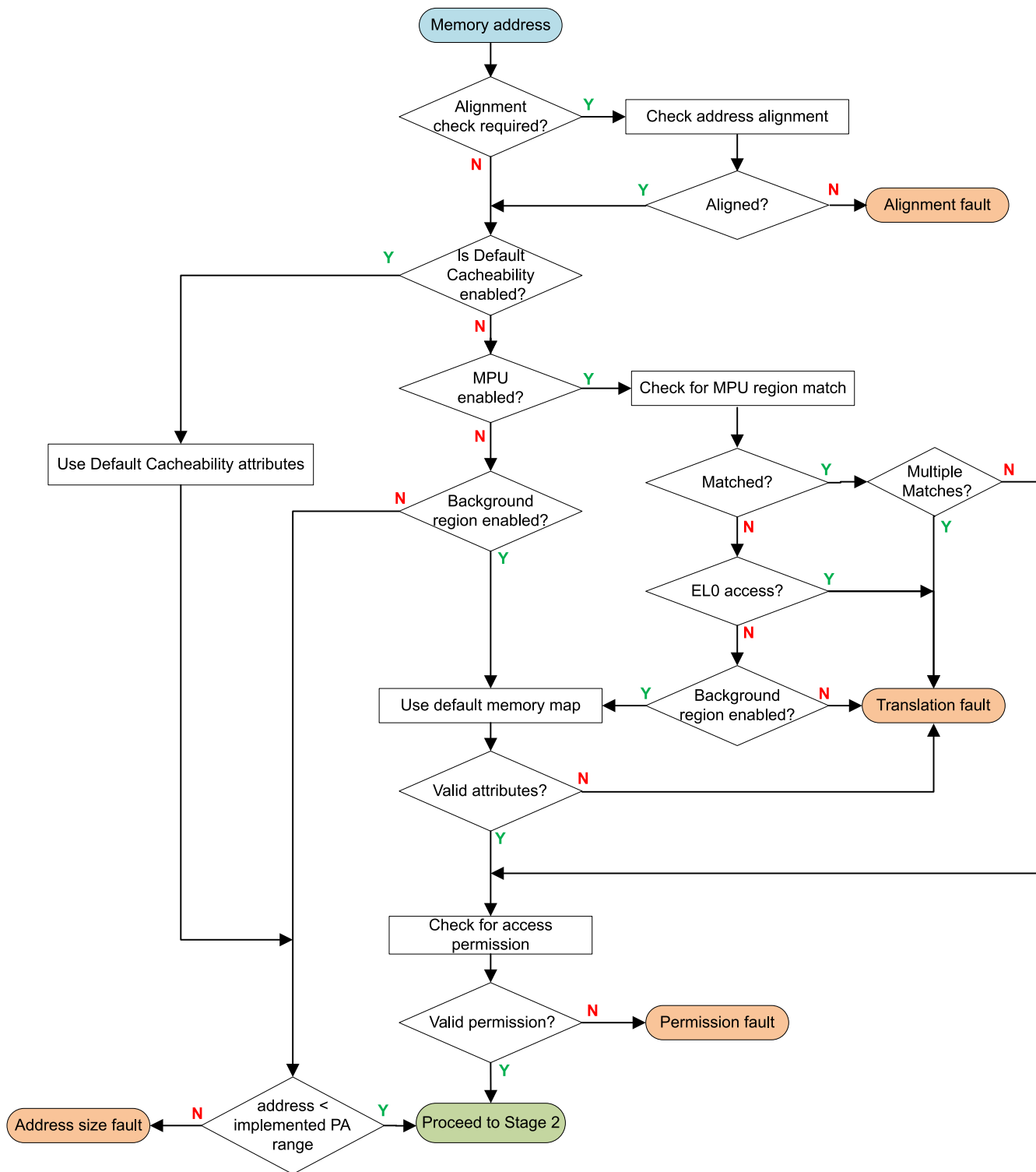
Figure D6-1 MPU fault check sequence for the stage 1 Secure EL1&0 translation
