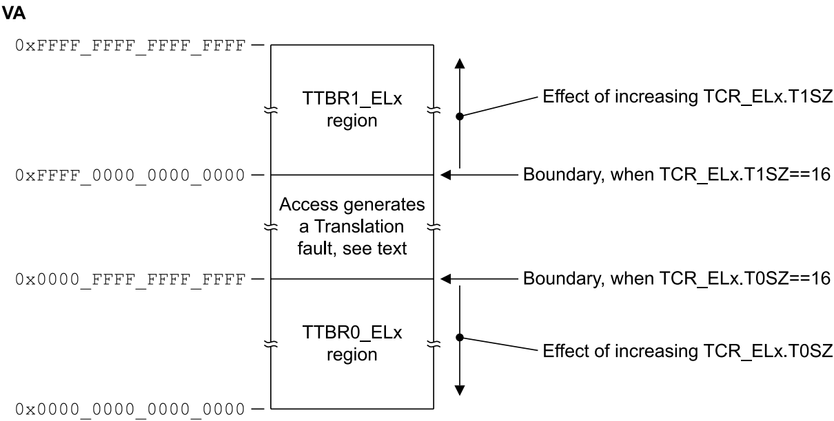
Figure D5-2 Example of a stage 1 translation that supports two VA ranges
