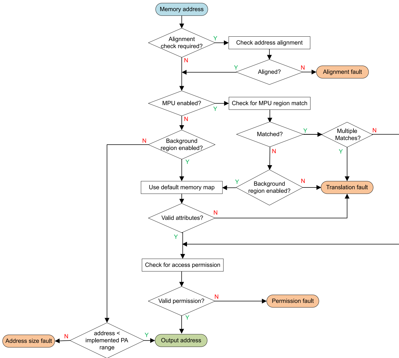
Figure D6-2 MPU fault check sequence for the stage 1 Secure EL2 translation
