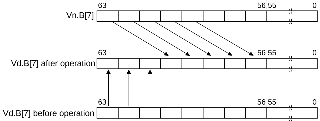
Figure C7-4 shift right by 3 for an 8-bit vector element
