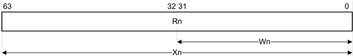
Figure B1-1 General-purpose register naming
