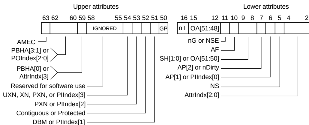
Figure D5-10 Stage 1 attribute fields in VMSAv8-64 Block and Page descriptors
