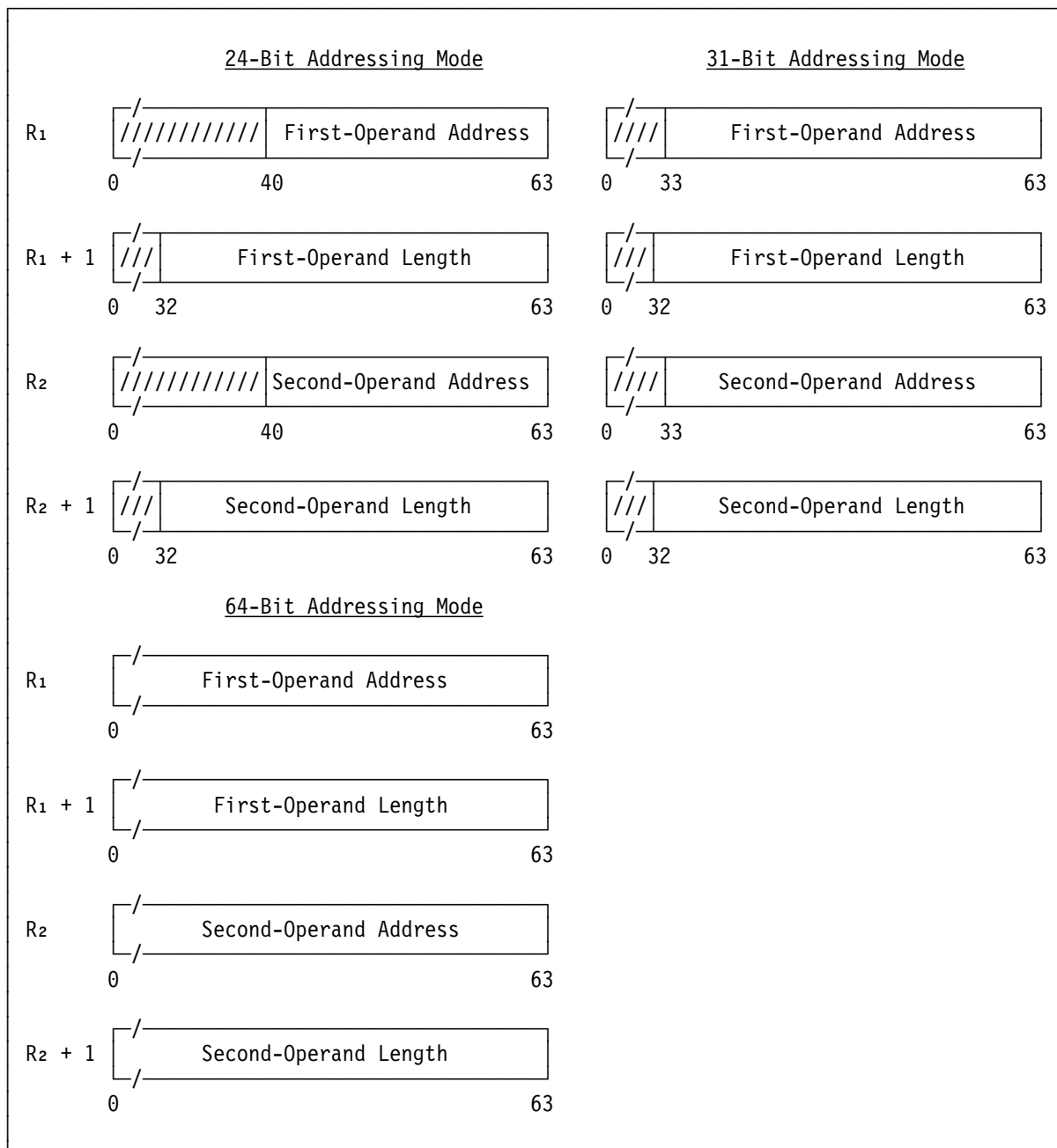
| Figure 7-70. Register Contents for CONVERT UTF-8 TO UTF-16
