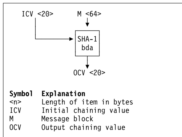
Figure 7-43. Symbol for SHA-1 Block Digest Algorithm
