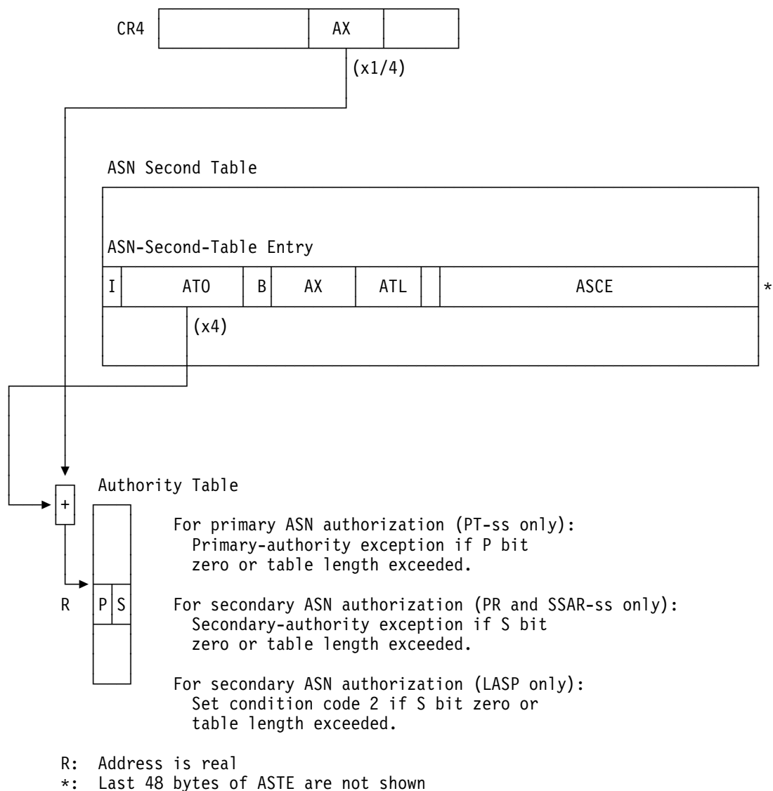
Figure 3-8. ASN Authorization
