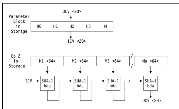
Figure 7-46. KIMD-SHA-1
