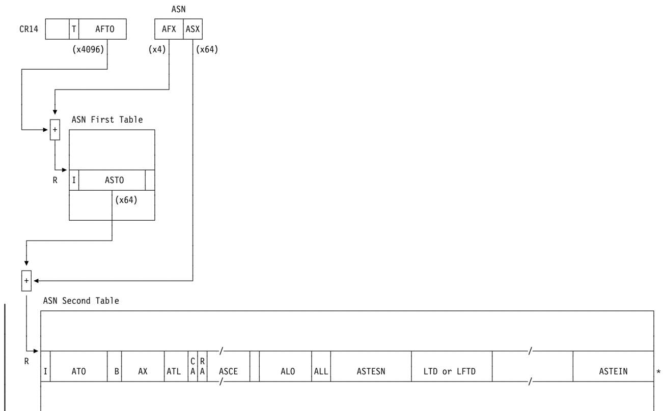
Figure 3-7. ASN Translation
