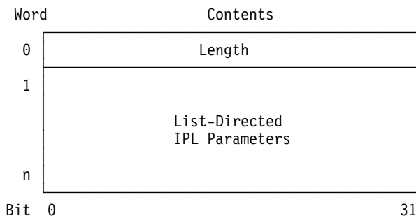
Figure 17-2. IPL-Parameter List
