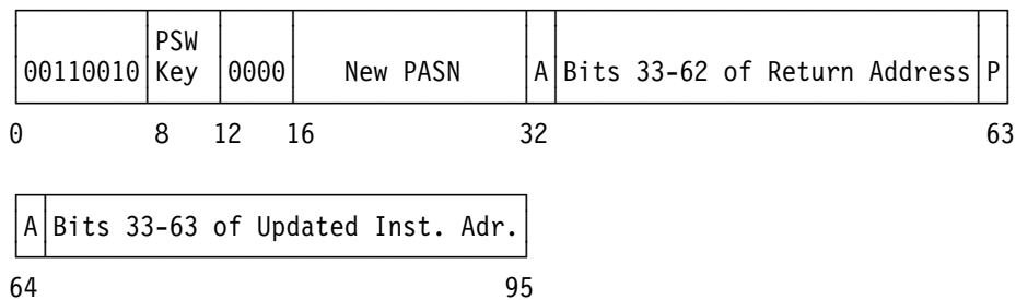
Figure 4-6 (Part 4 of 9). Trace Entries
