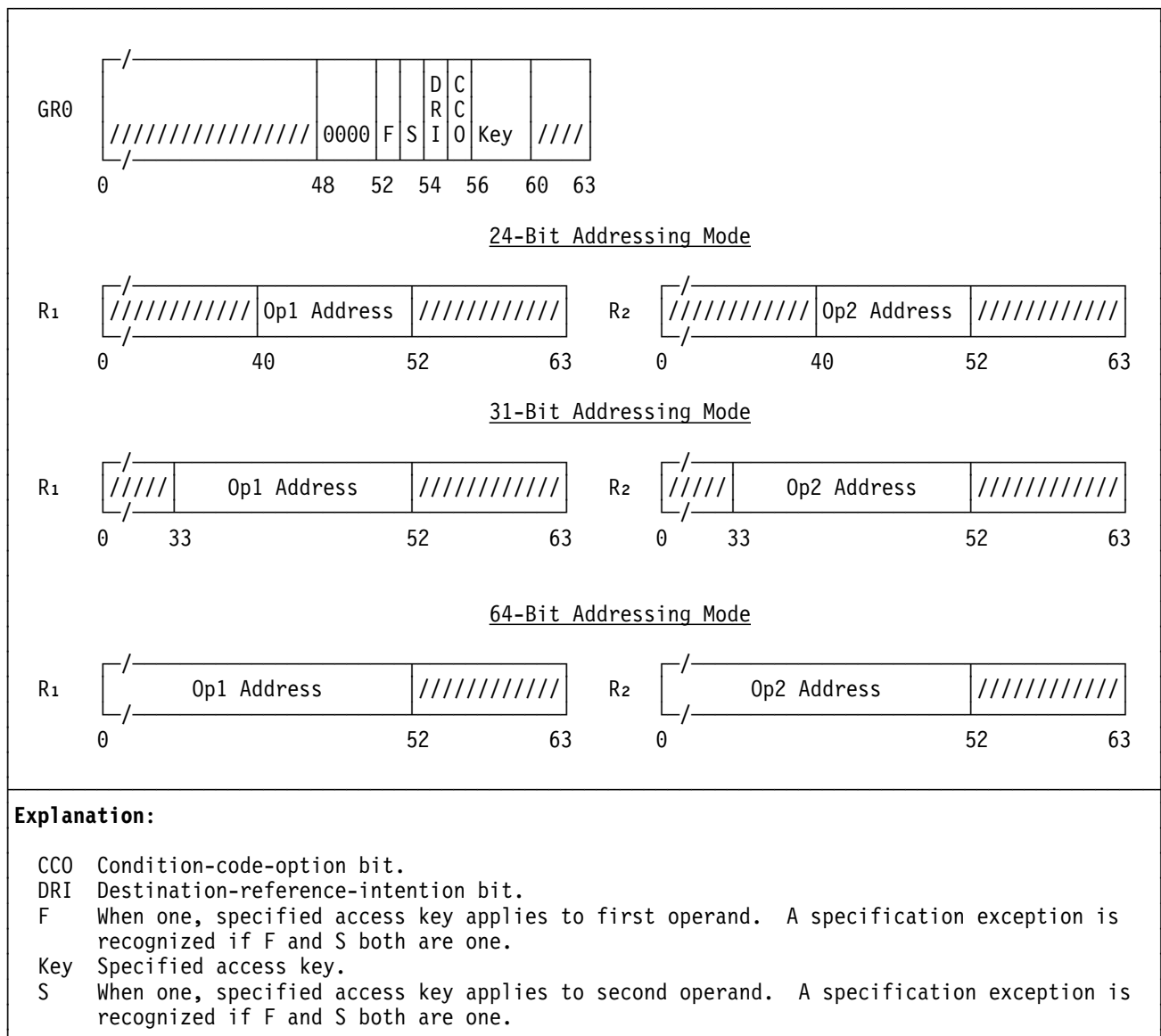
Figure 10-20. Register Contents for MOVE PAGE
