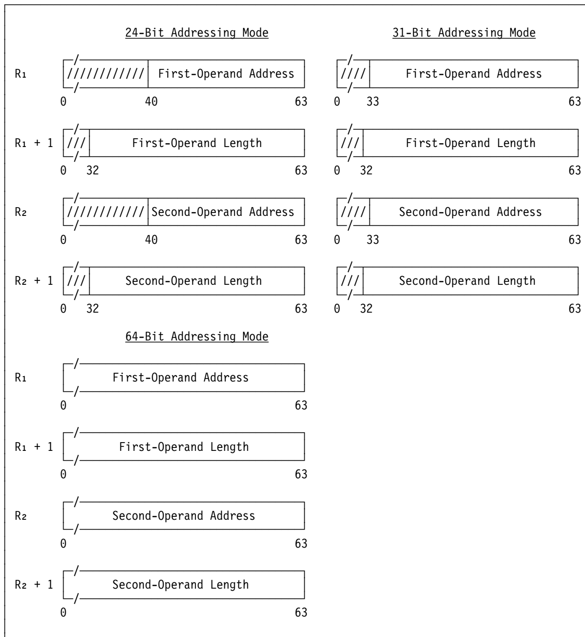
Figure 7-67. Register Contents for CONVERT UTF-16 TO UTF-8
