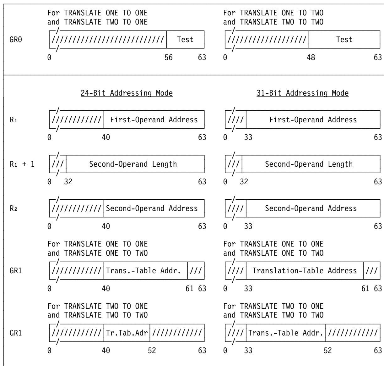
Figure 7-80 (Part 1 of 2). Register Contents for TRANSLATE ONE TO ONE, TRANSLATE ONE TO TWO, TRANSLATE TWO TO ONE, and TRANSLATE TWO TO TWO
