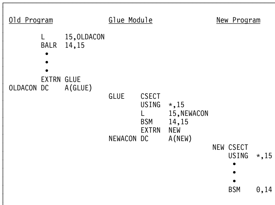
Figure 5-4. Glue Module for Linkage from the 24-Bit Mode to the 31-Bit Mode
