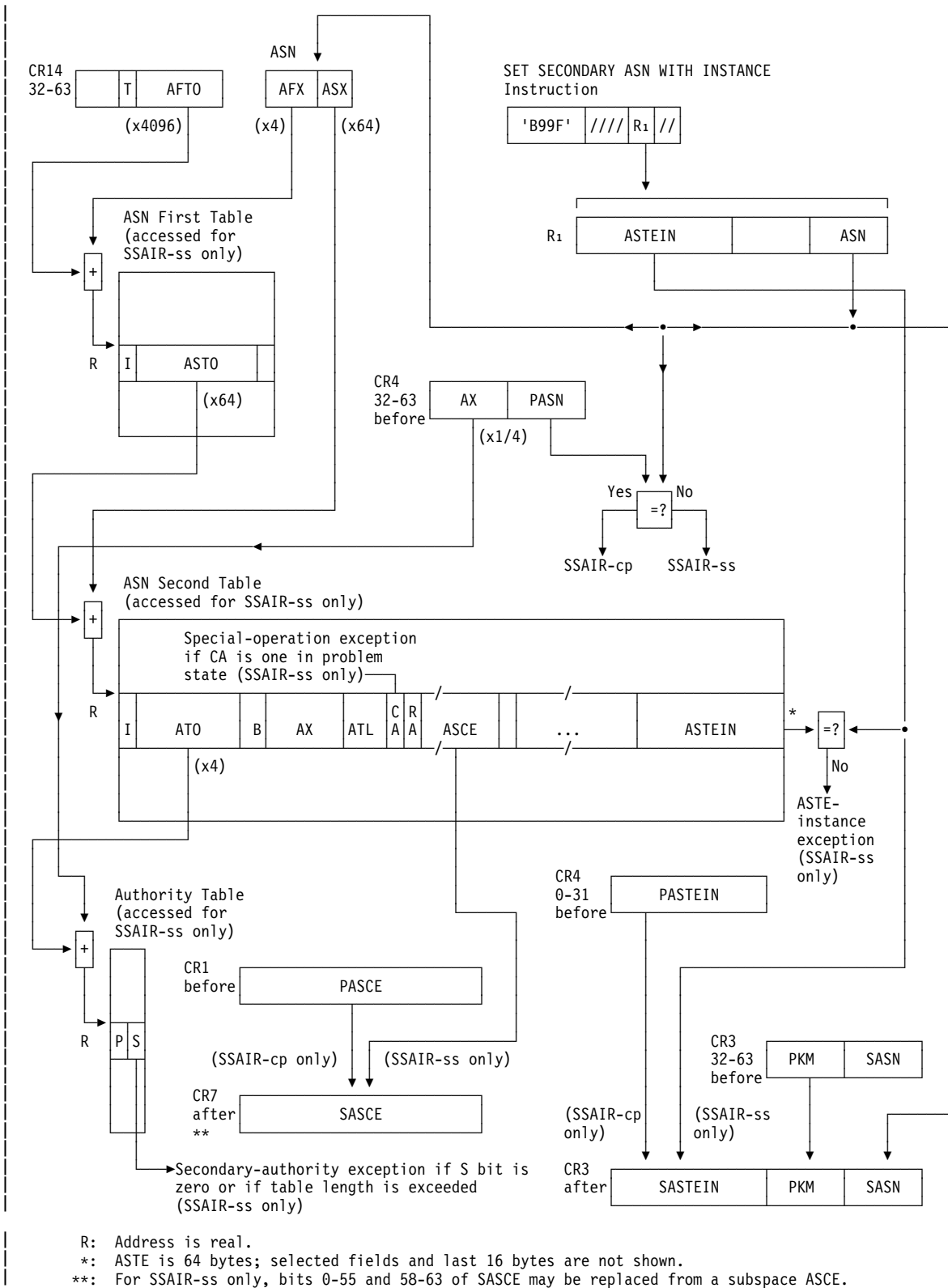
Figure 10-33. Execution of SET SECONDARY ASN WITH INSTANCE
