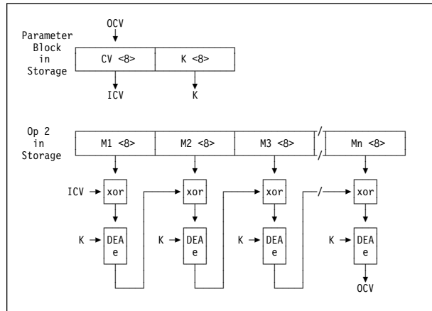
Figure 7-60. KMAC-DEA
