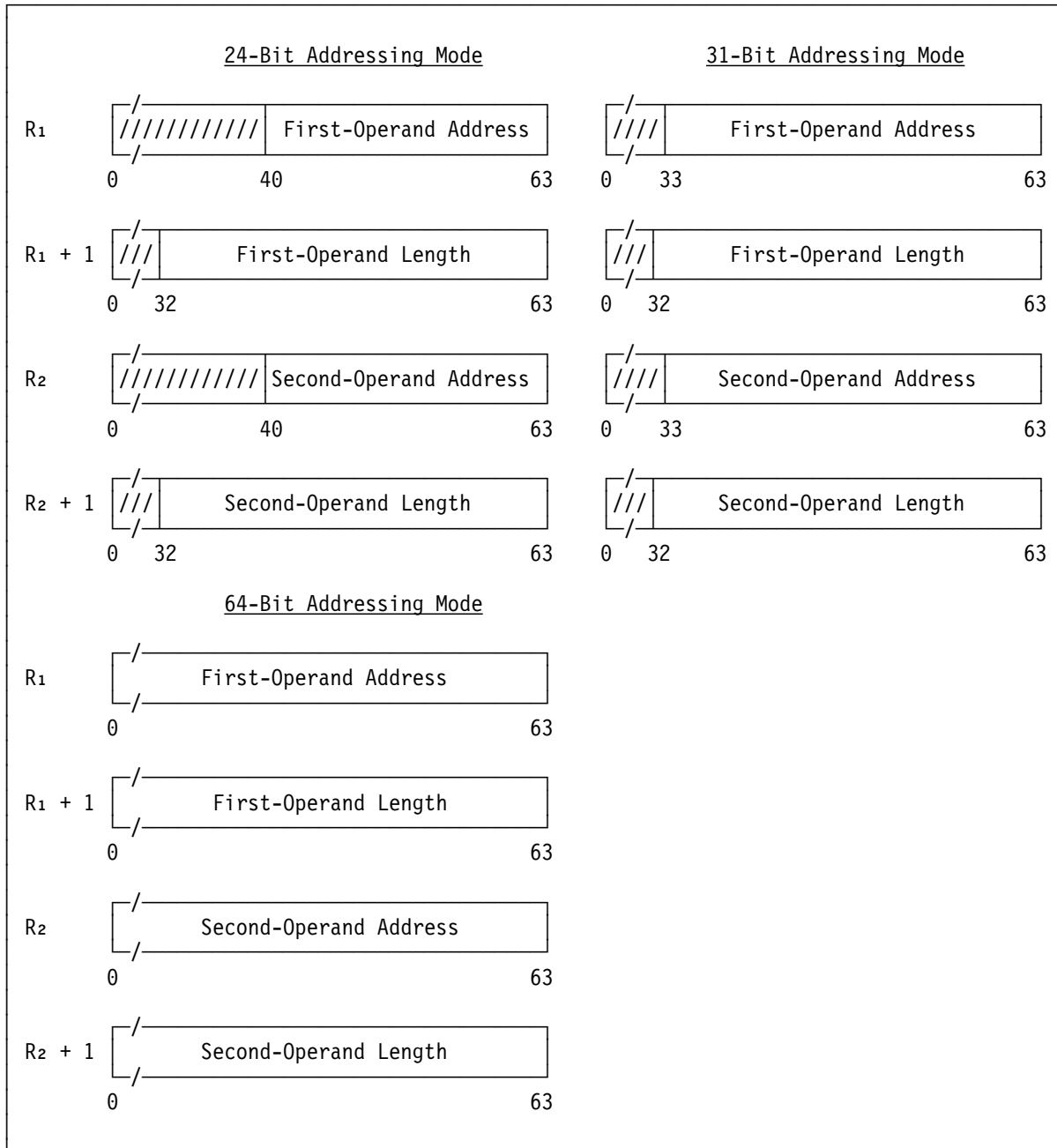
Figure 7-66. Register Contents for CONVERT UTF-16 TO UTF-32
