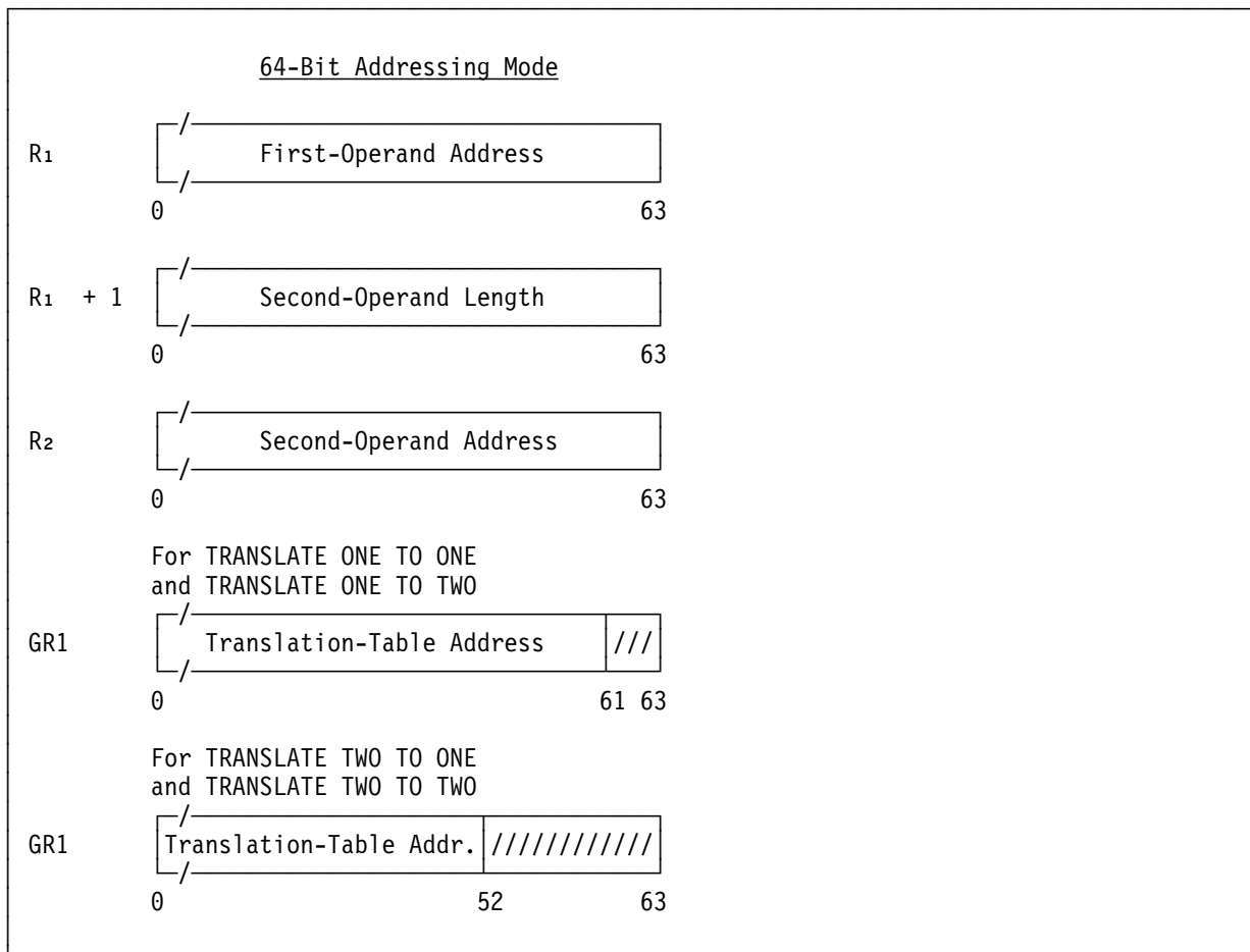
Figure 7-80 (Part 2 of 2). Register Contents for TRANSLATE ONE TO ONE, TRANSLATE ONE TO TWO, TRANSLATE TWO TO ONE, and TRANSLATE TWO TO TWO
