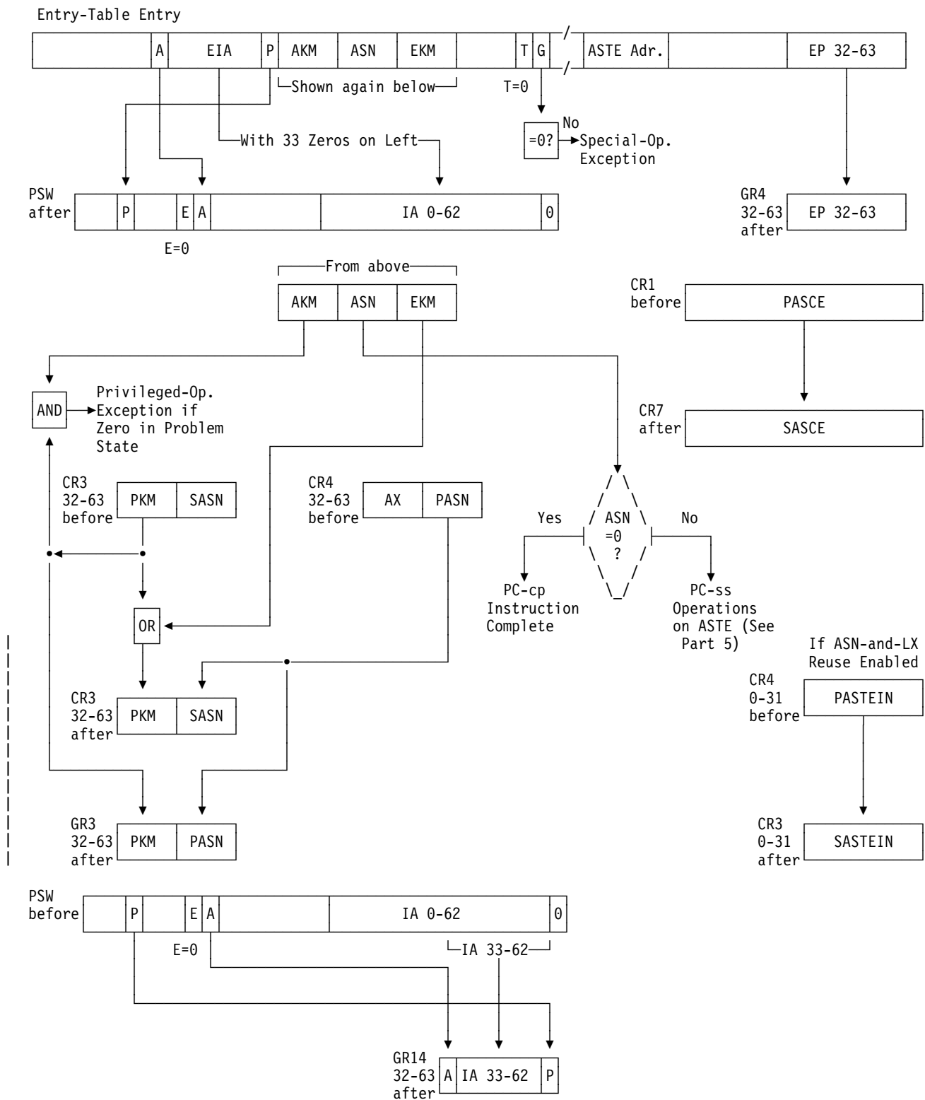
Figure 10-24 (Part 1 of 5). Execution of PROGRAM CALL
