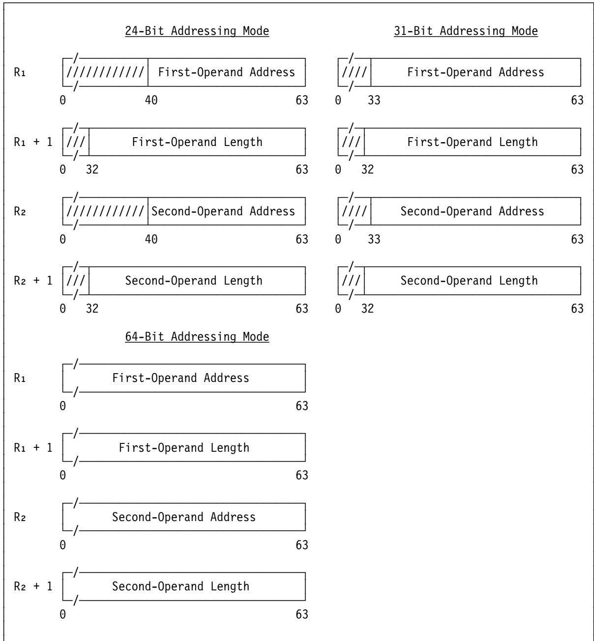
Figure 7-69. Register Contents for CONVERT UTF-32 TO UTF-8
