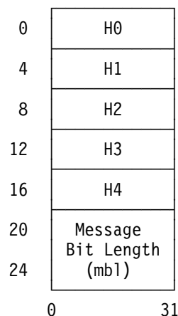
Figure 7-48. Parameter Block for KLMD-SHA-1
