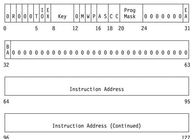
Figure 4-2. PSW Format
