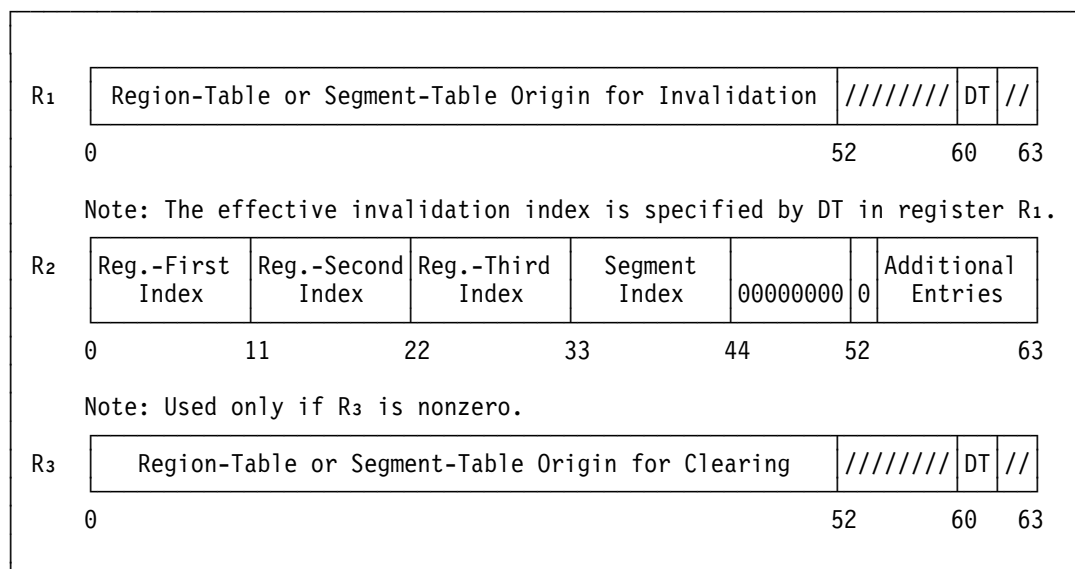
Figure 10-12. Register Contents for INVALIDATE DAT TABLE ENTRY Invalidation-and-Clearing Operation (Bit 52 of GR R 2 Is Zero)
