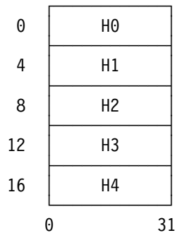
Figure 7-45. Parameter Block for KIMD-SHA-1
