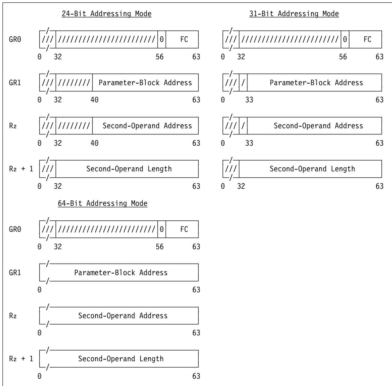
Figure 7-42. General Register Assignment for KIMD and KLMD
