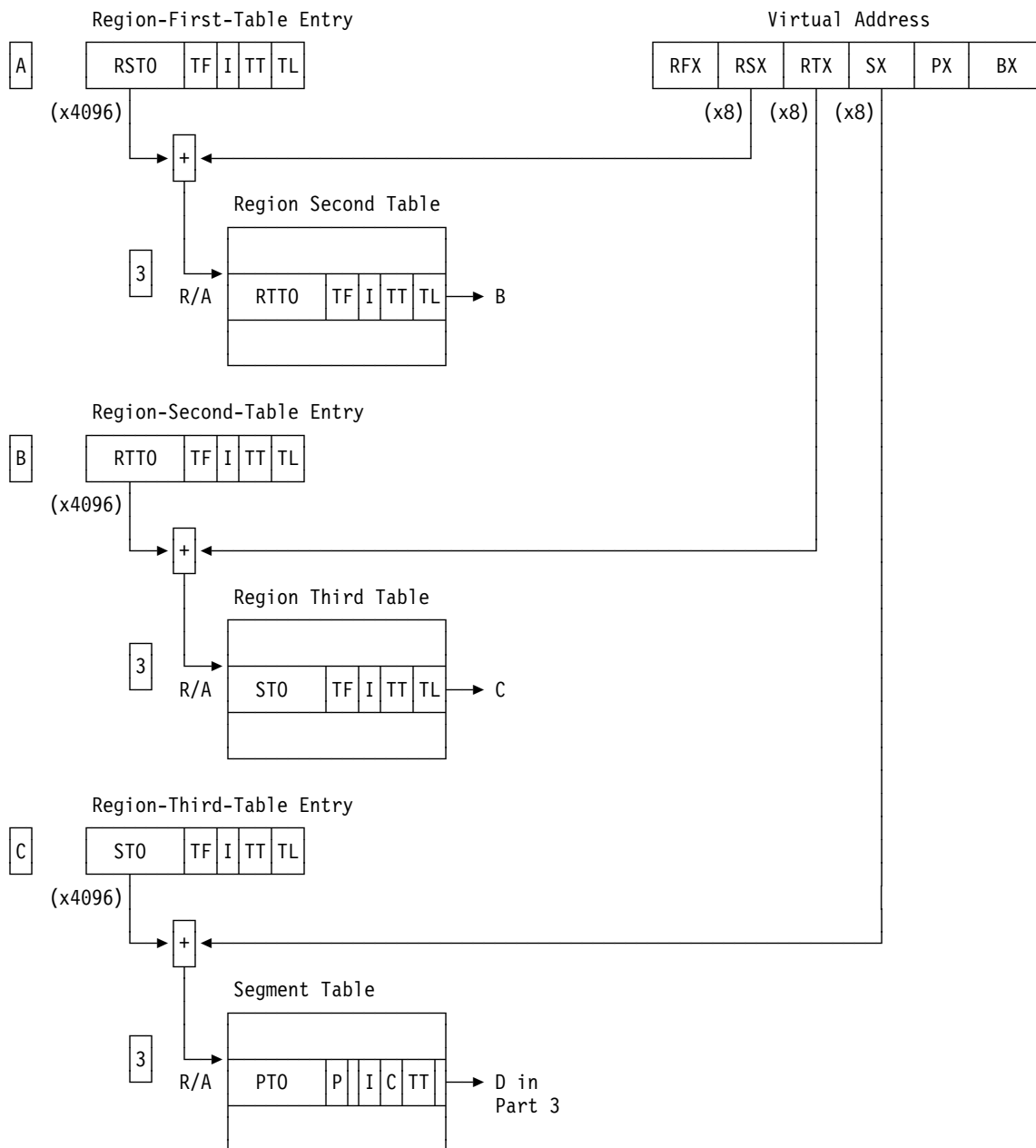
Figure 3-10 (Part 2 of 3). Translation Process
