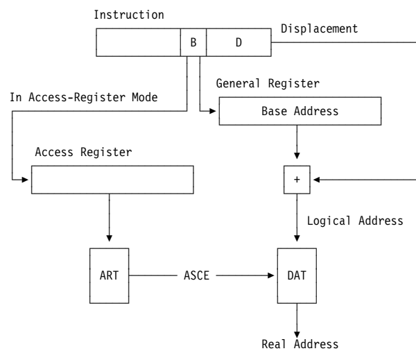
Figure 5-10. Use of Access Registers
