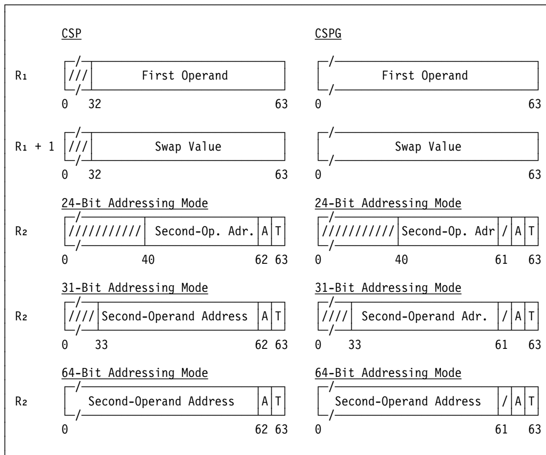
Figure 10-5. Register Contents for COMPARE AND SWAP AND PURGE
