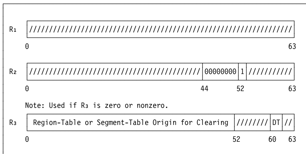
Figure 10-13. Register Contents for INVALIDATE DAT TABLE ENTRY Clearing-by-ASCE Operation (Bit 52 of GR R 2 Is One)
