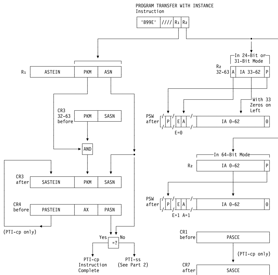
Figure 10-28 (Part 1 of 2). Execution of PROGRAM TRANSFER WITH INSTANCE
