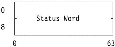
Figure 7-58. Parameter Block for KMAC-Query
