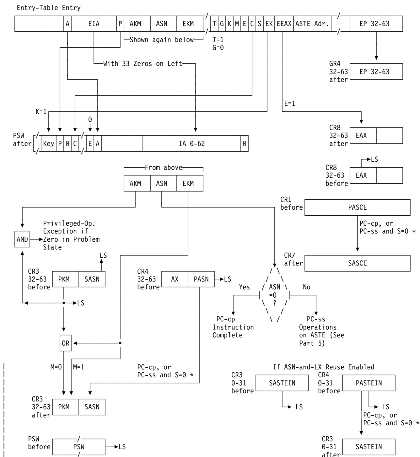
Figure 10-24 (Part 4 of 5). Execution of PROGRAM CALL
