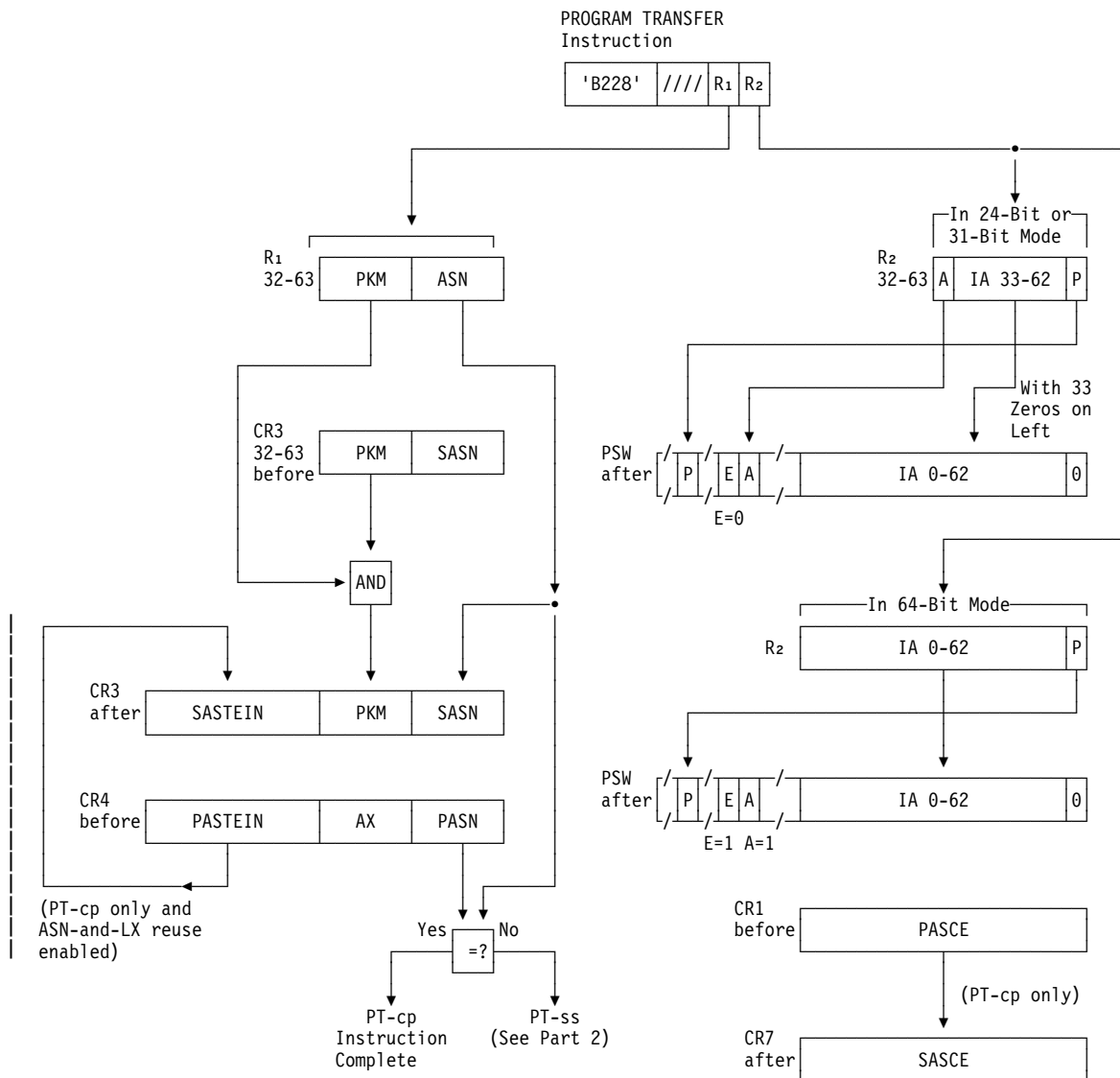
Figure 10-27 (Part 1 of 2). Execution of PROGRAM TRANSFER
