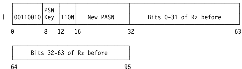
Figure 4-6 (Part 7 of 9). Trace Entries
