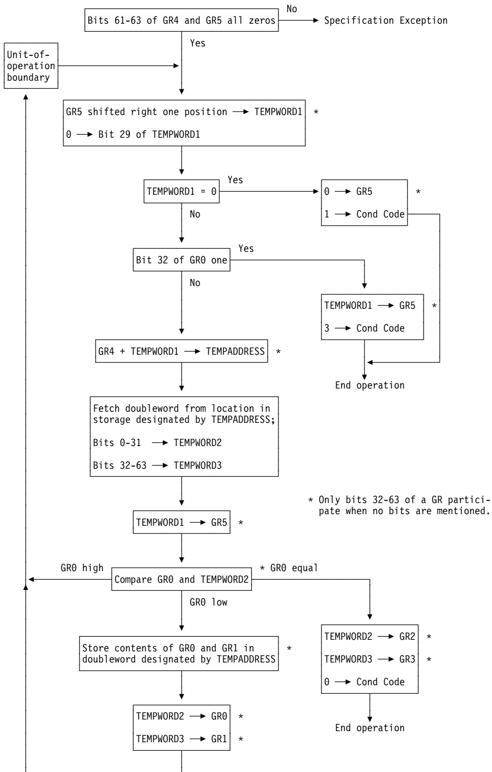
Figure 7-81. Execution of UPDATE TREE in the 24-Bit or 31-Bit Addressing Mode
