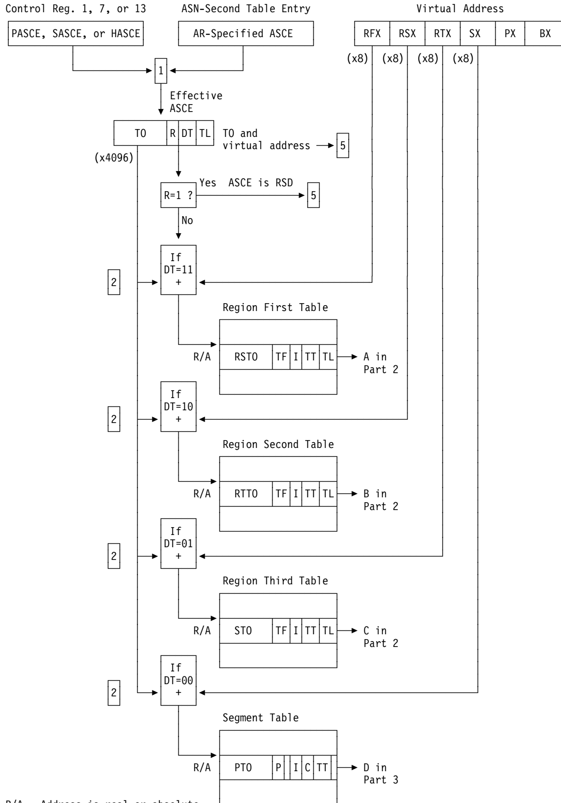
Figure 3-10 (Part 1 of 3). Translation Process
