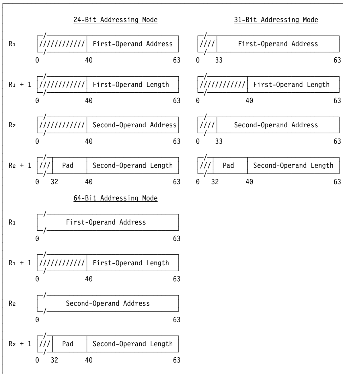
Figure 7-72. Register Contents for MOVE LONG
