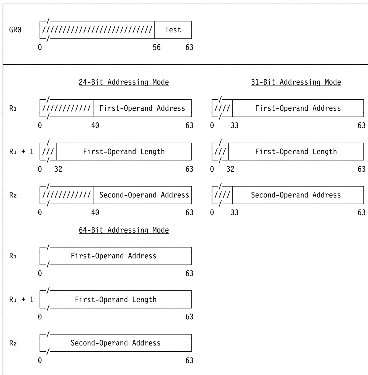
Figure 7-79. Register Contents for TRANSLATE EXTENDED
