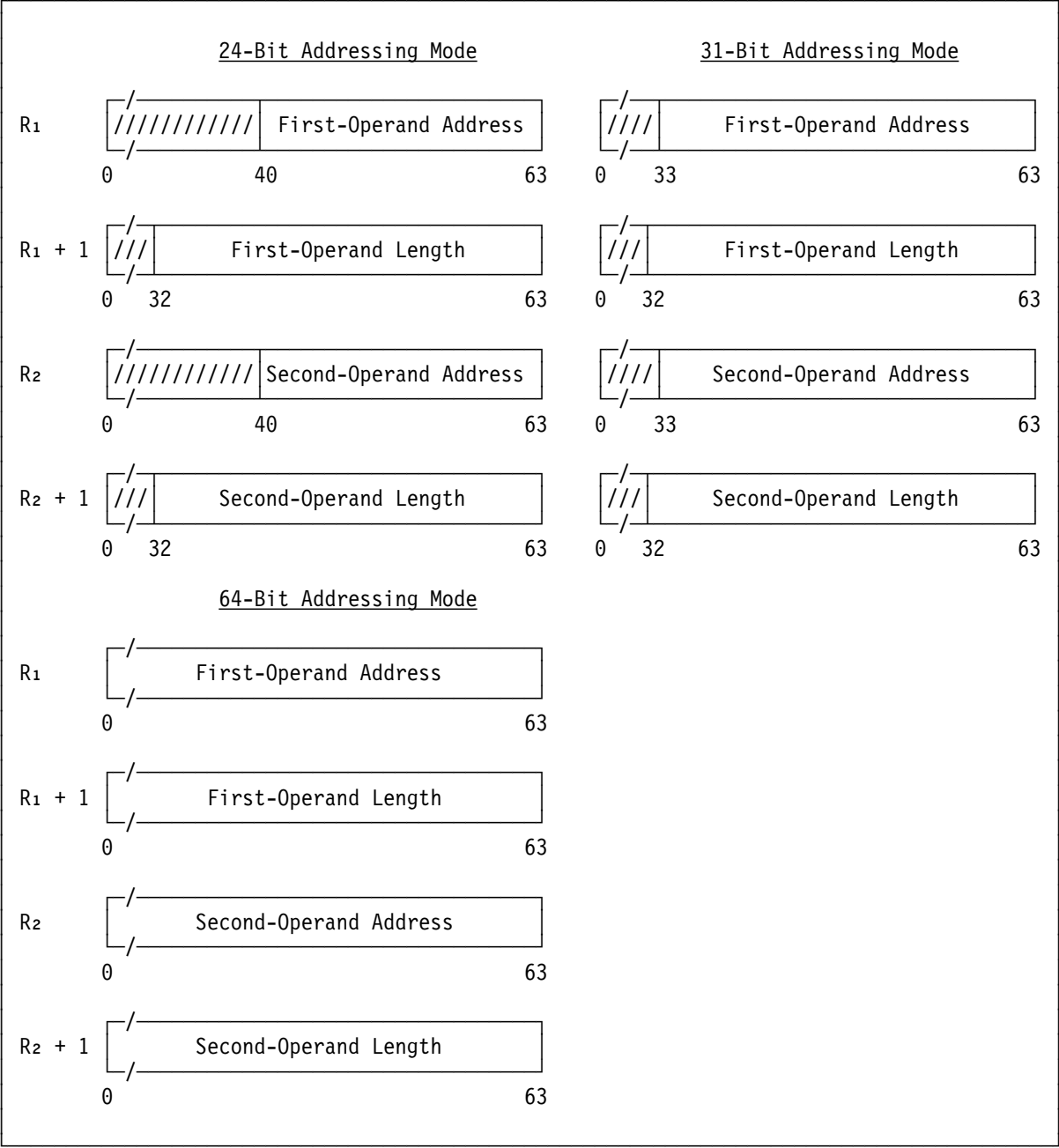
Figure 7-71. Register Contents for CONVERT UTF-8 TO UTF32
