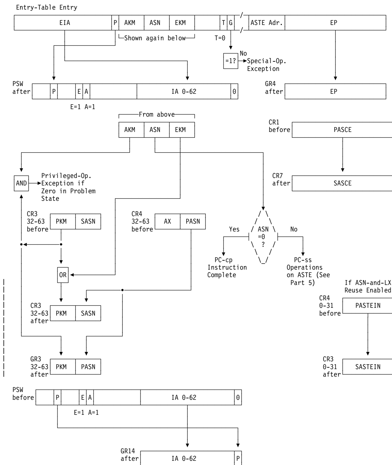
Figure 10-24 (Part 2 of 5). Execution of PROGRAM CALL
