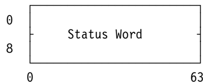
Figure 7-44. Parameter Block for KIMD-Query
