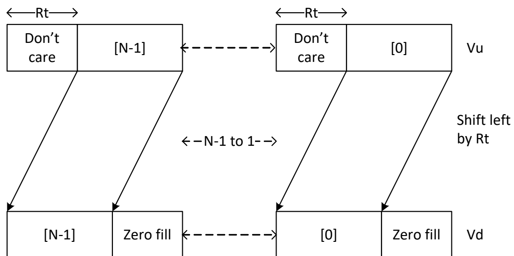
Figure 6-21 Shift left by R_t
