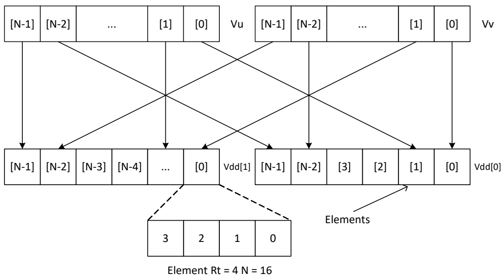
Figure 6-9 Vector shuffle and deal cross-lane operations
