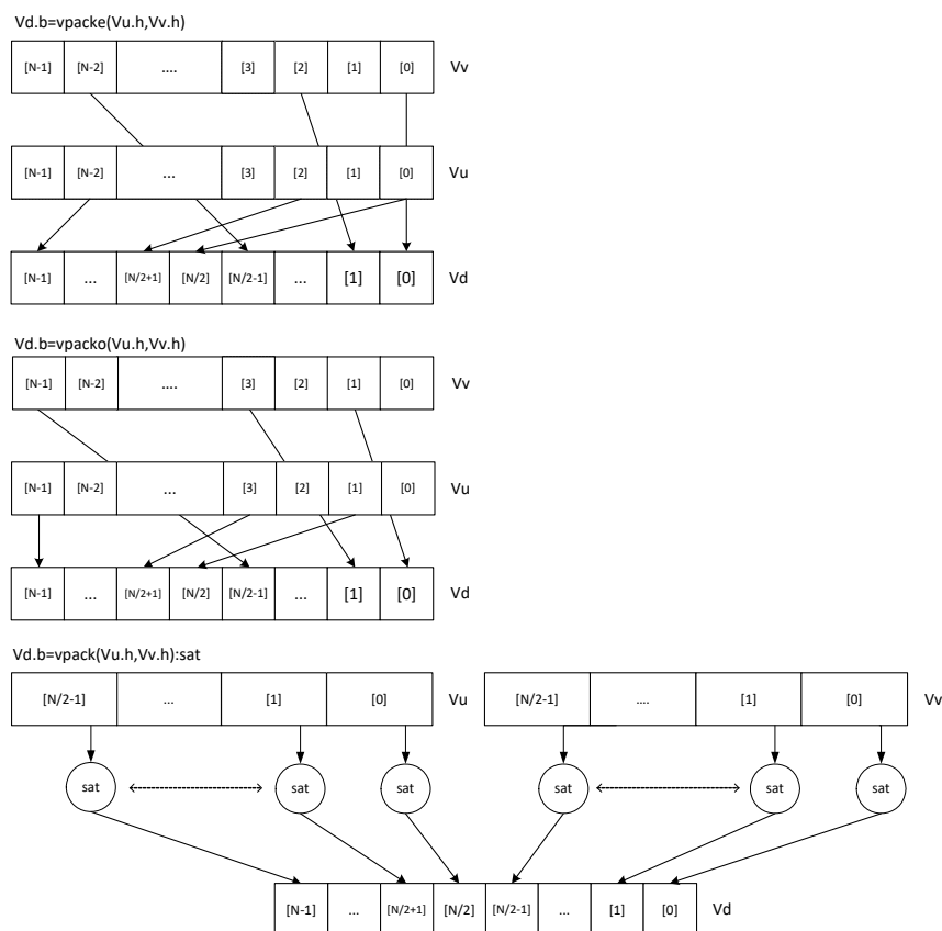
Figure 6-5 vpack operation
