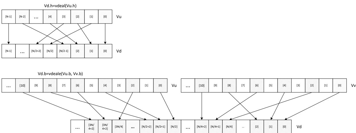
Figure 6-3 Vdeale operation
