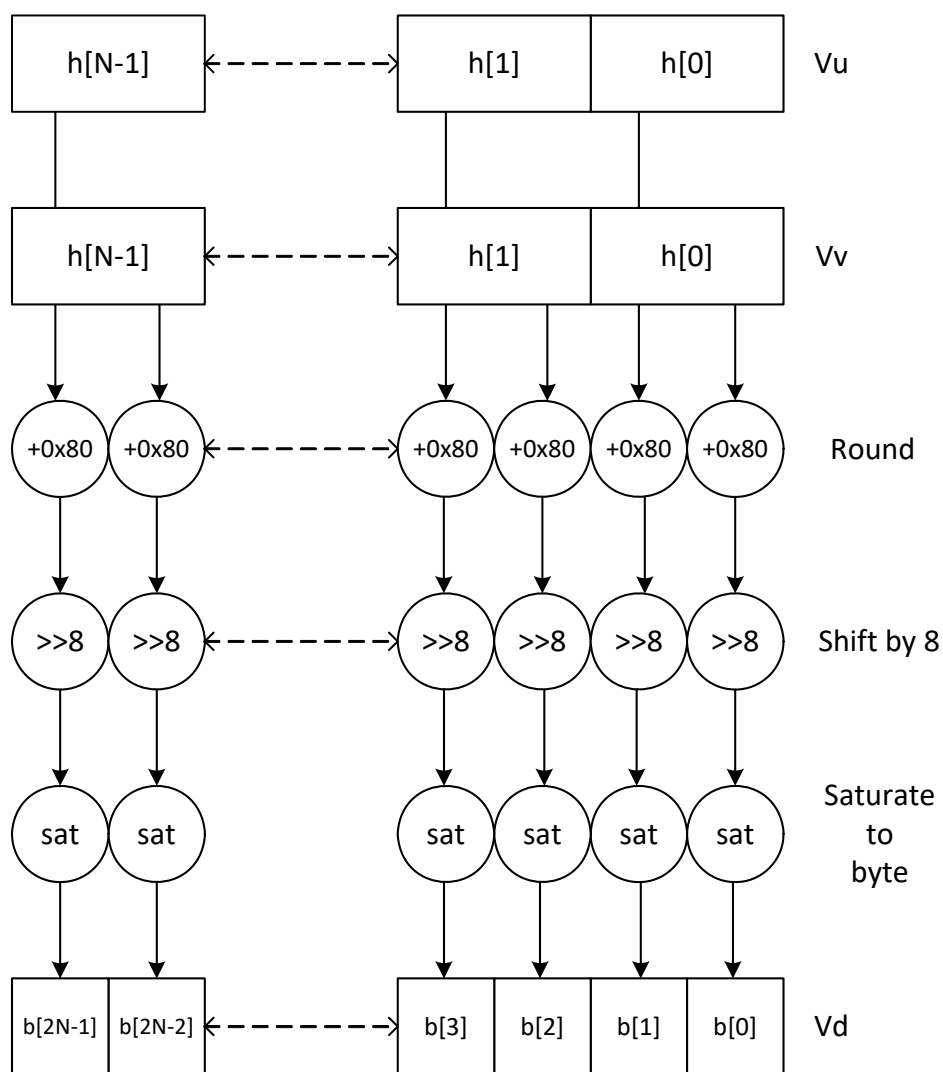
Figure 6-23 Vd.b = vround(Vu.h, Vv.h):sat
