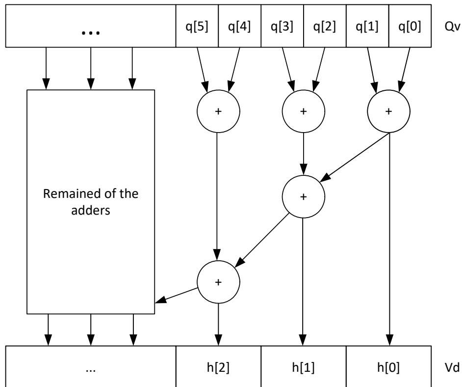
Figure 6-17 Vd32.h = \text{prefixsum}(qv4)
