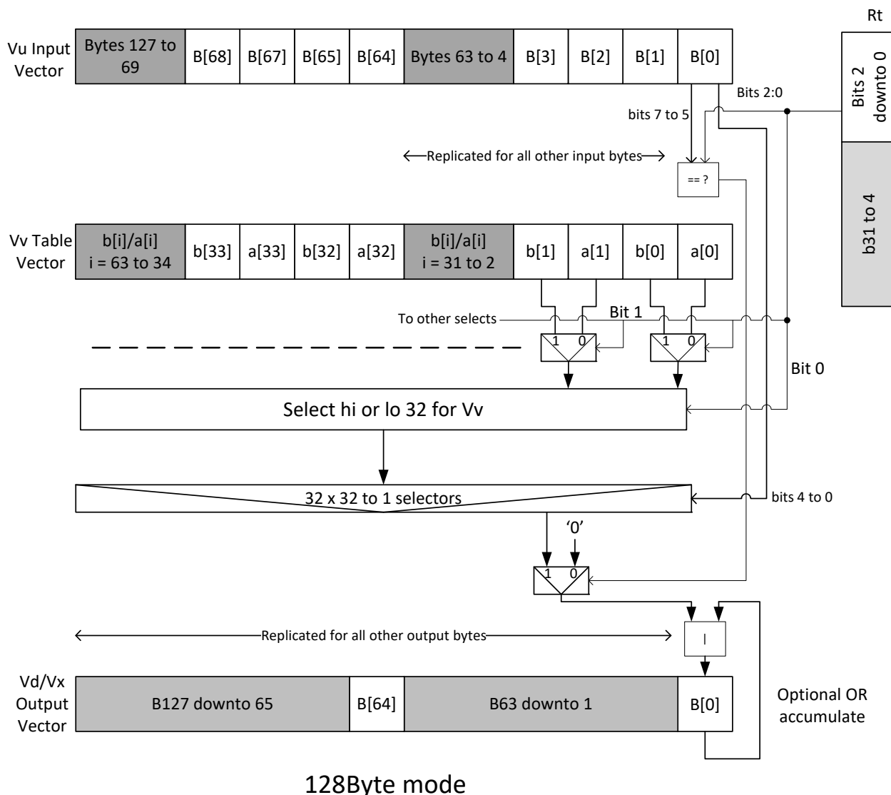
Figure 6-13 The vlut32 operation in 128 byte mode
