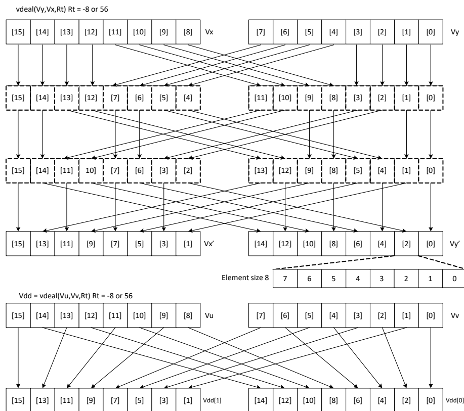
Figure 6-6 vdeal(Vy, Vx, Rt) \text{ Rt} = -8 \text{ or } 56
