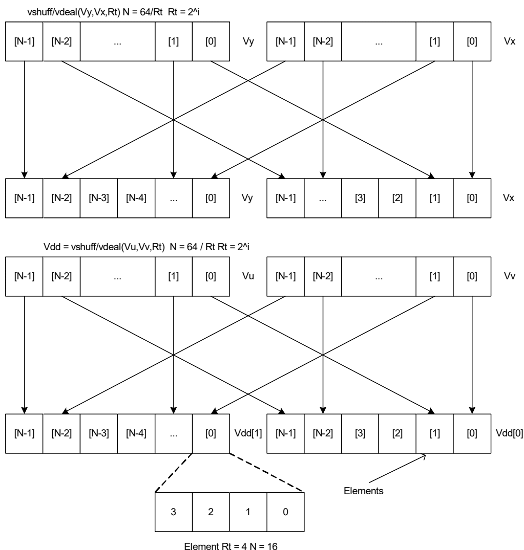
Figure 6-4 vshuff/vdeal ( Vy, Vx, Rt ) N = 64/Rt \quad Rt = 2^i
