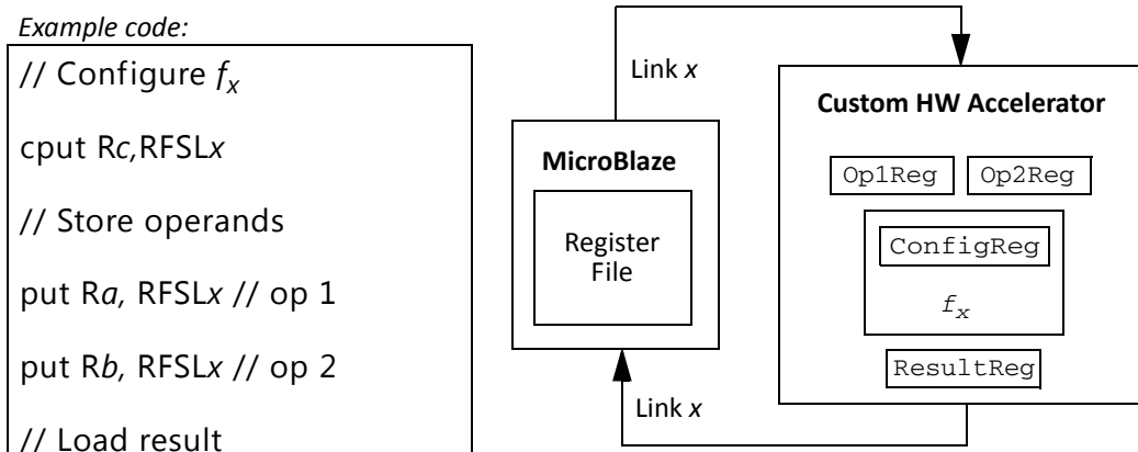
Figure 2-25: Stream Link Used with HW Accelerated Function f_x
