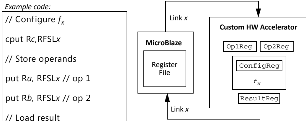
Figure 2-25: Stream Link Used with HW Accelerated Function f_x
