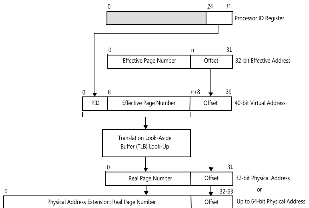
Figure 2-18: Virtual-Mode Address Translation
