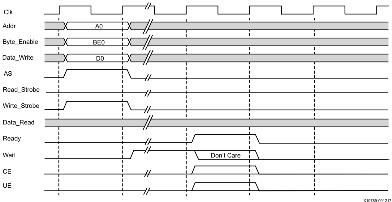
Figure 3-3: LMB Generic Write Operation, N Wait State
