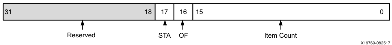
Figure 2-33: Trace Status Register
