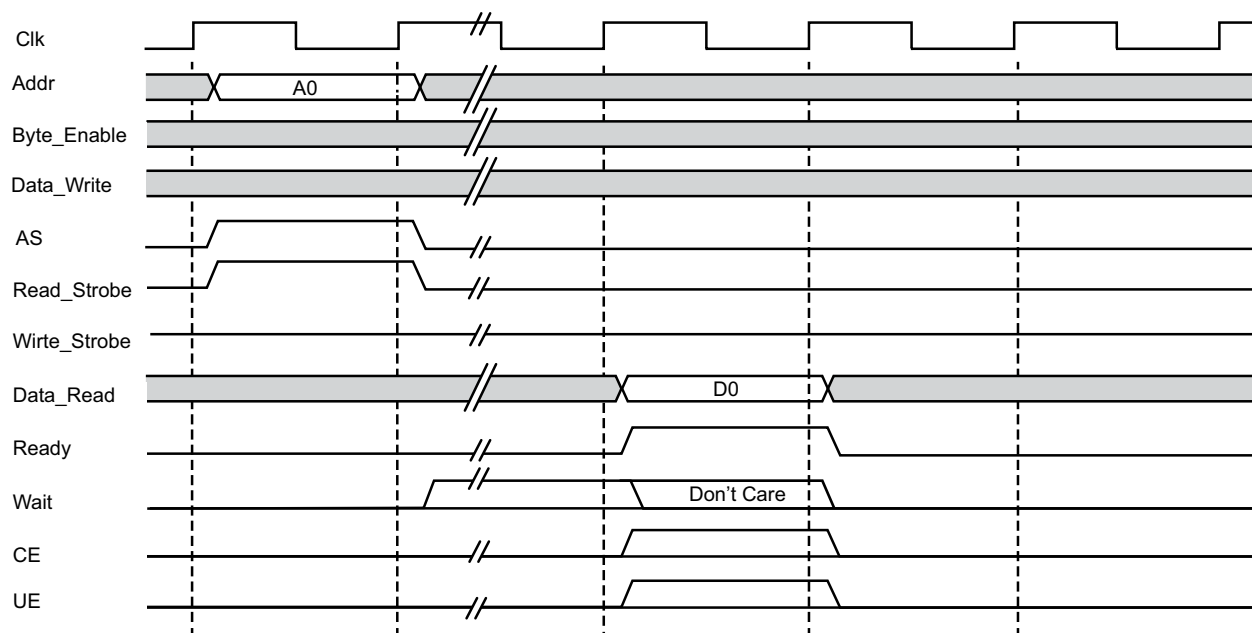
Figure 3-5: LMB Generic Read Operation, N Wait States
