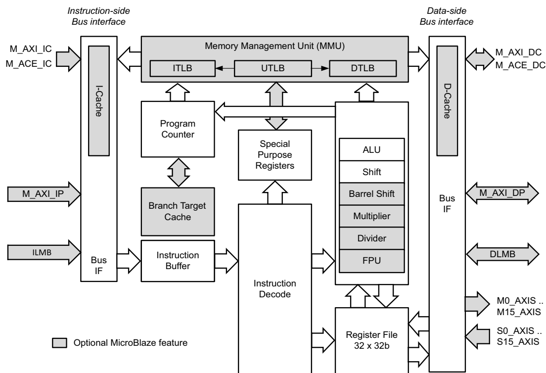
Figure 3-1: MicroBlaze Core Block Diagram
