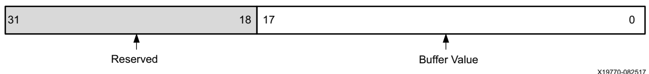
Figure 2-34: Trace Data Read Register
