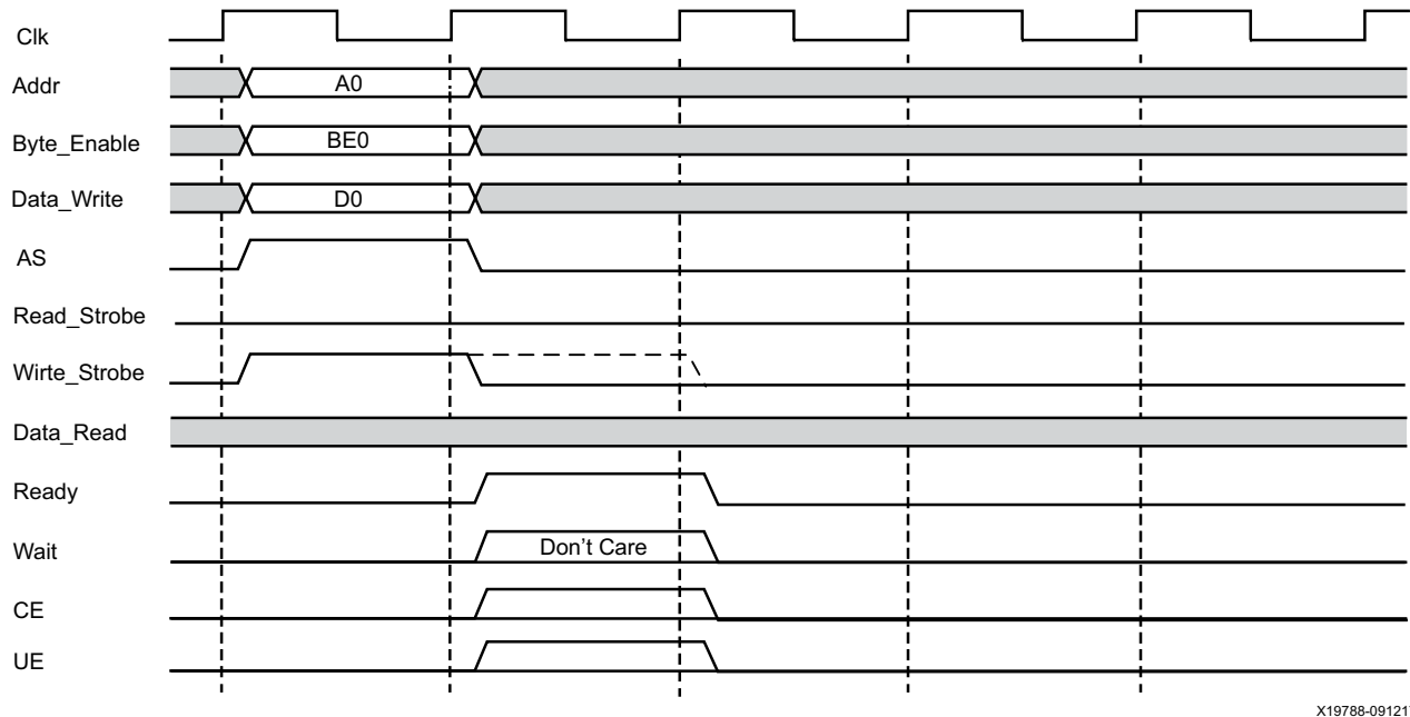
Figure 3-2: LMB Generic Write Operation, 0 Wait States
