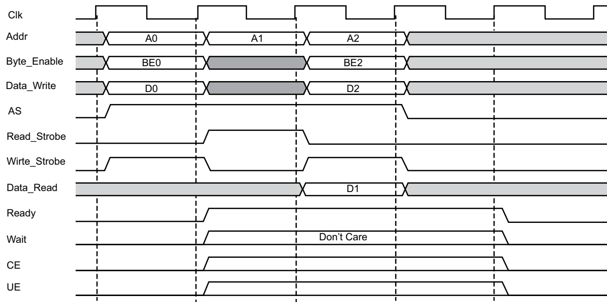
Figure 3-8: Back-to-Back Mixed Write/Read Operation, 0 Wait States
