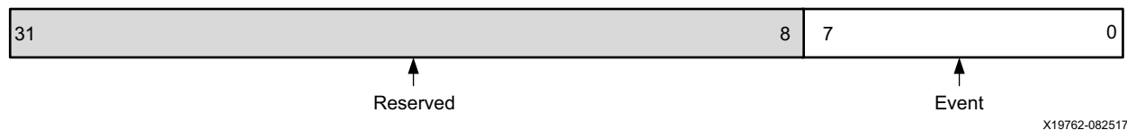
Figure 2-26: Performance Counter Control Register
