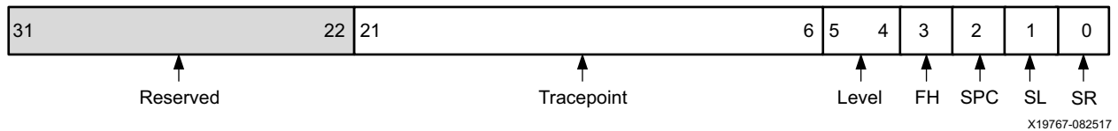
Figure 2-31: Trace Control Register
