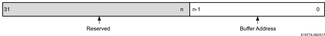
Figure 2-38: Profiling Buffer Address Register
