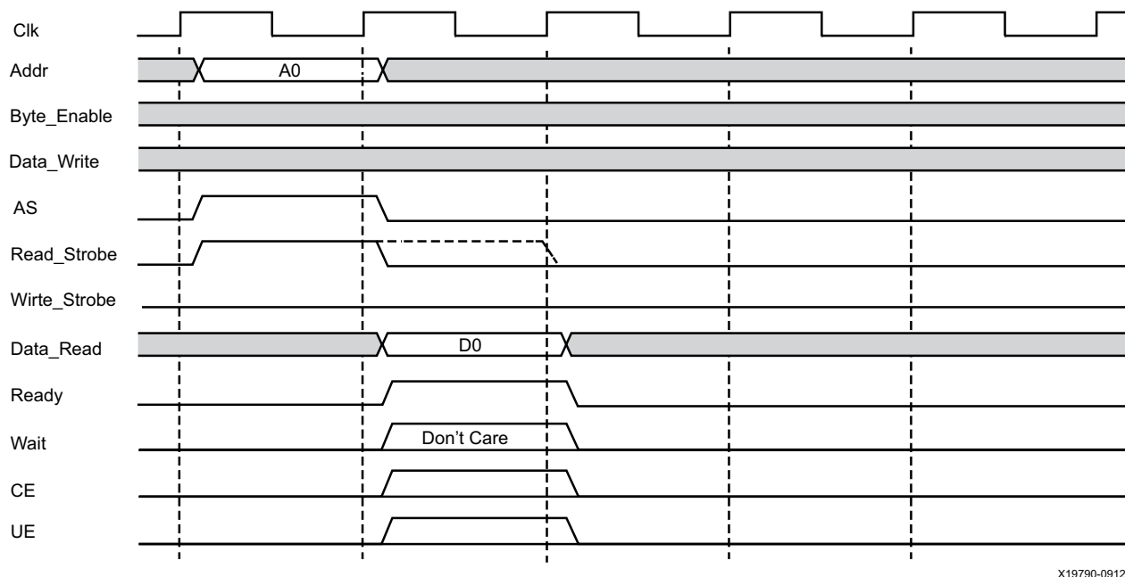
Figure 3-4: LMB Generic Read Operation, 0 Wait States
