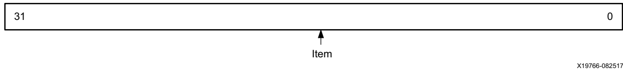
Figure 2-30: Performance Counter Data Write Register
