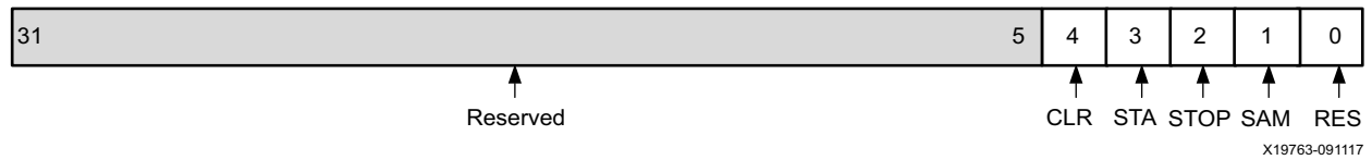
Figure 2-27: Performance Counter Command Register
