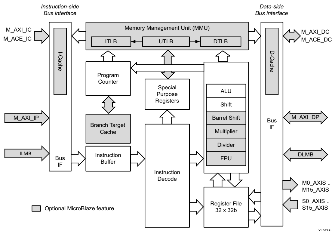
Figure 3-1: MicroBlaze Core Block Diagram
