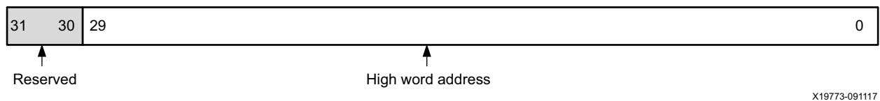
Figure 2-37: Profiling High Address Register
