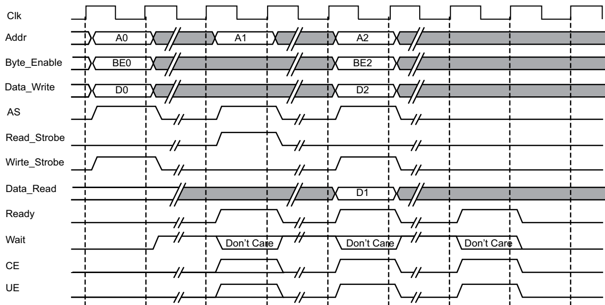
Figure 3-9: Back-to-Back Mixed Write/Read Operation, N Wait States
