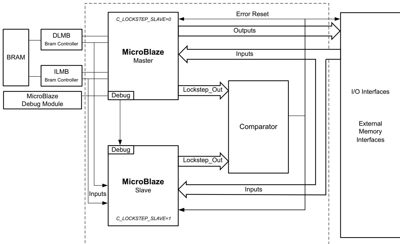
Figure 2-42: Lockstep Error Detection Application
