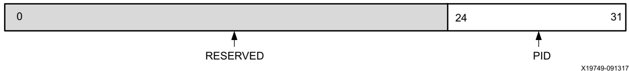
Figure 2-12: PID
