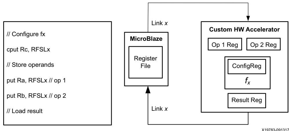
Figure 2-25: Stream Link Used with HW Accelerated Function f_x
