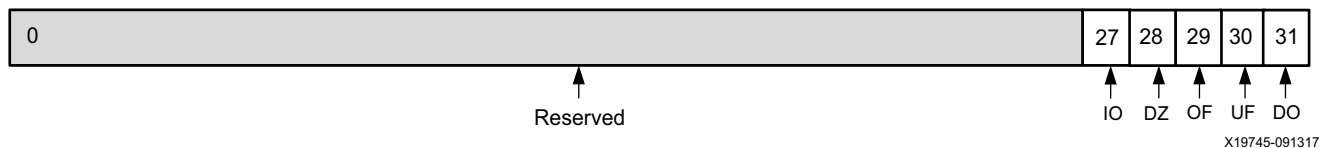
Figure 2-8: FSR
