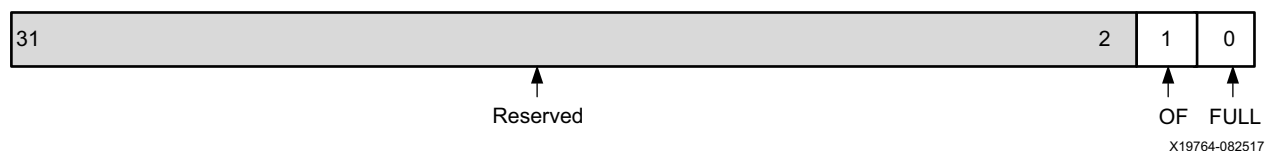
Figure 2-28: Performance Counter Status Register
