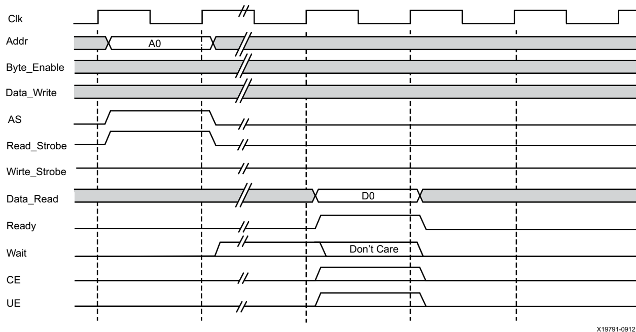
Figure 3-5: LMB Generic Read Operation, N Wait States
