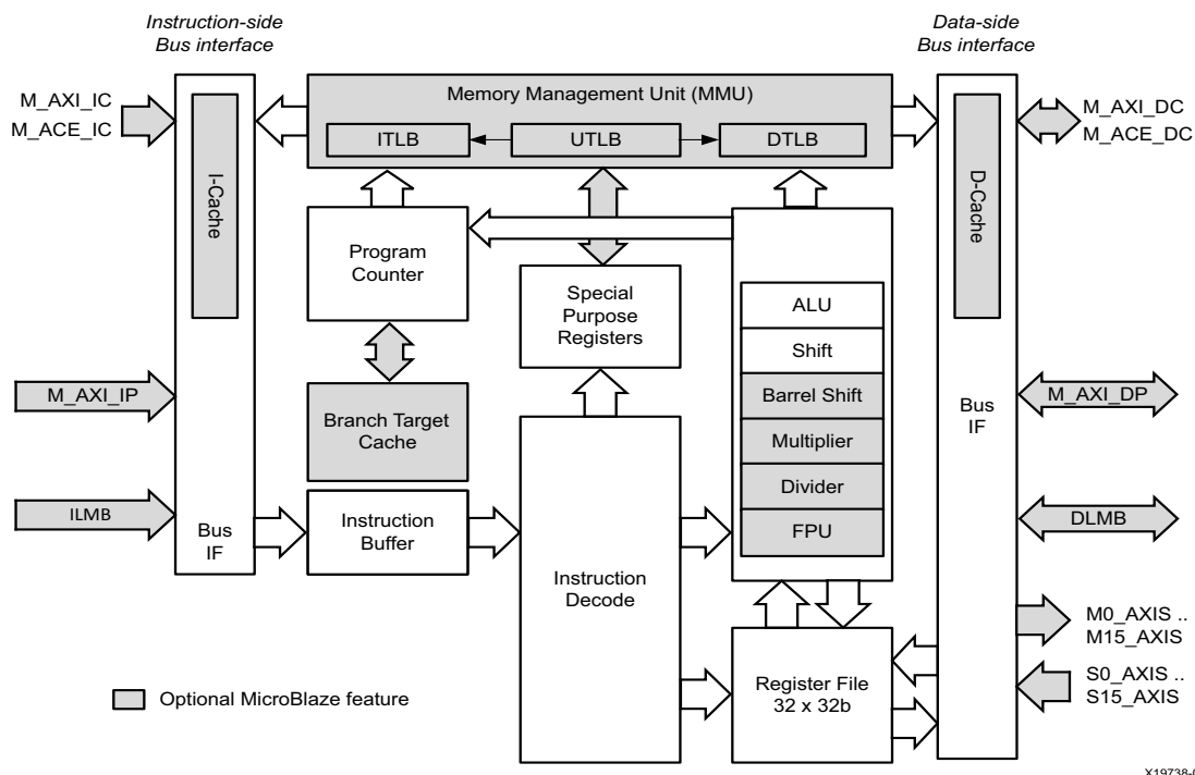
Figure 2-1: MicroBlaze Core Block Diagram
