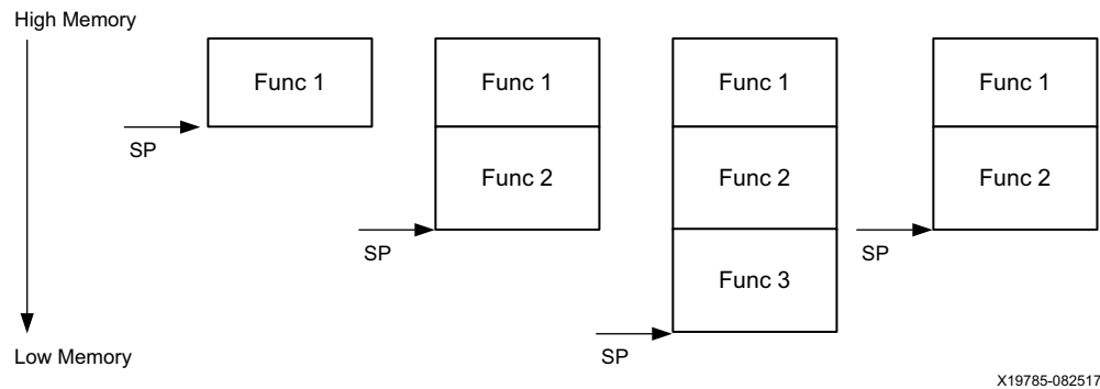
Figure 4-1: Stack Frame
