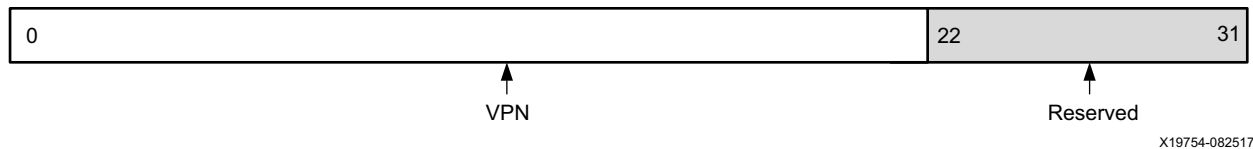
Figure 2-17: TLBSX
