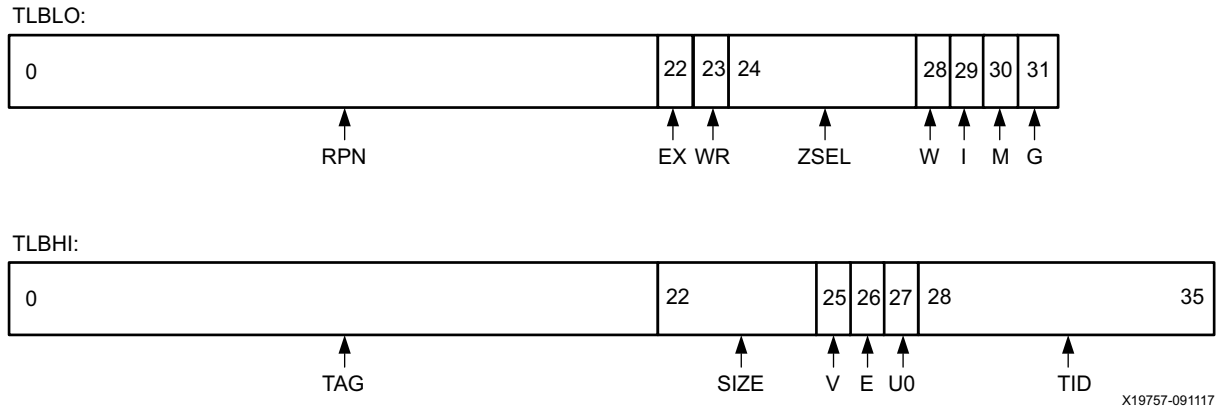
Figure 2-20: TLB Entry Format (PAE Disabled)
