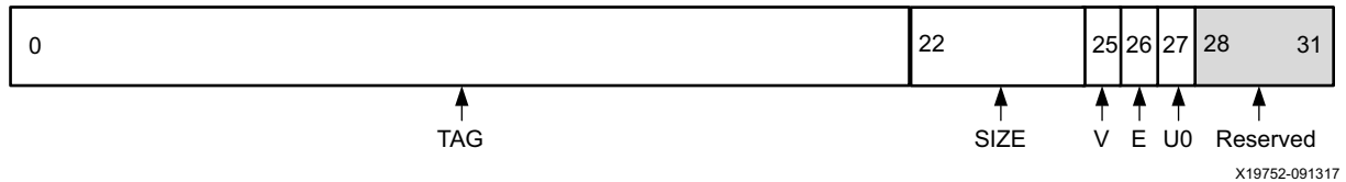
Figure 2-15: TLBHI
