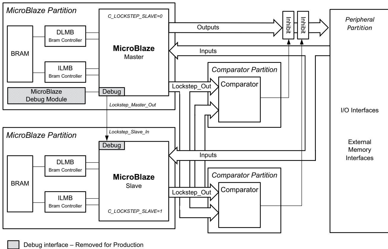
Figure 2-41: Lockstep Tamper Protection Application
