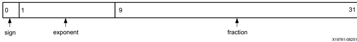
Figure 2-24: IEEE 754 Single Precision Format
