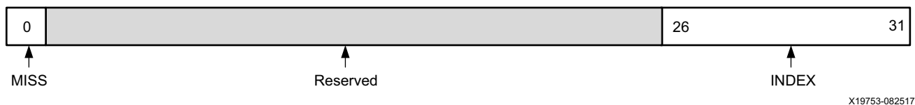
Figure 2-16: TLBX
