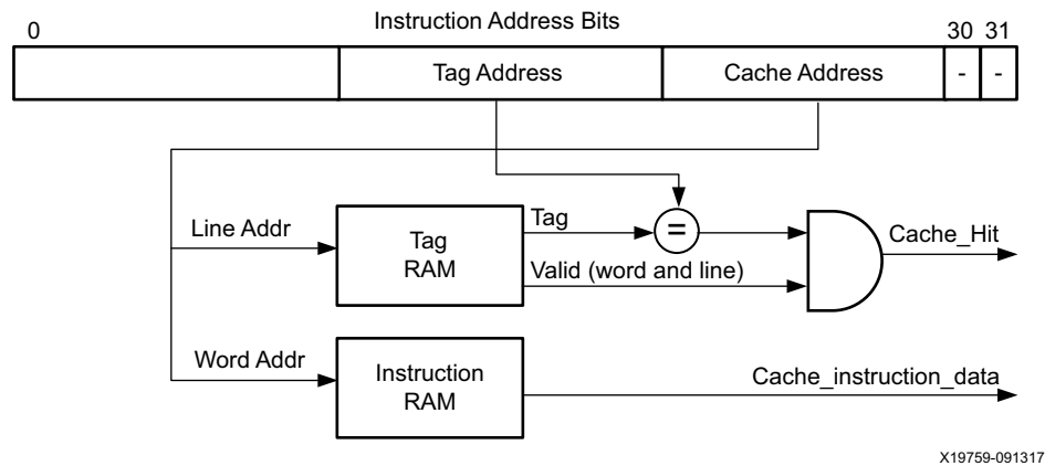
Figure 2-22: Instruction Cache Organization
