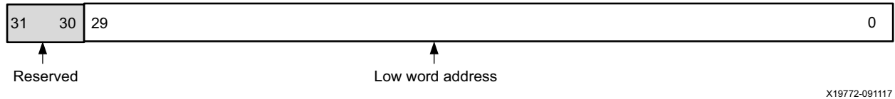
Figure 2-36: Profiling Low Address Register
