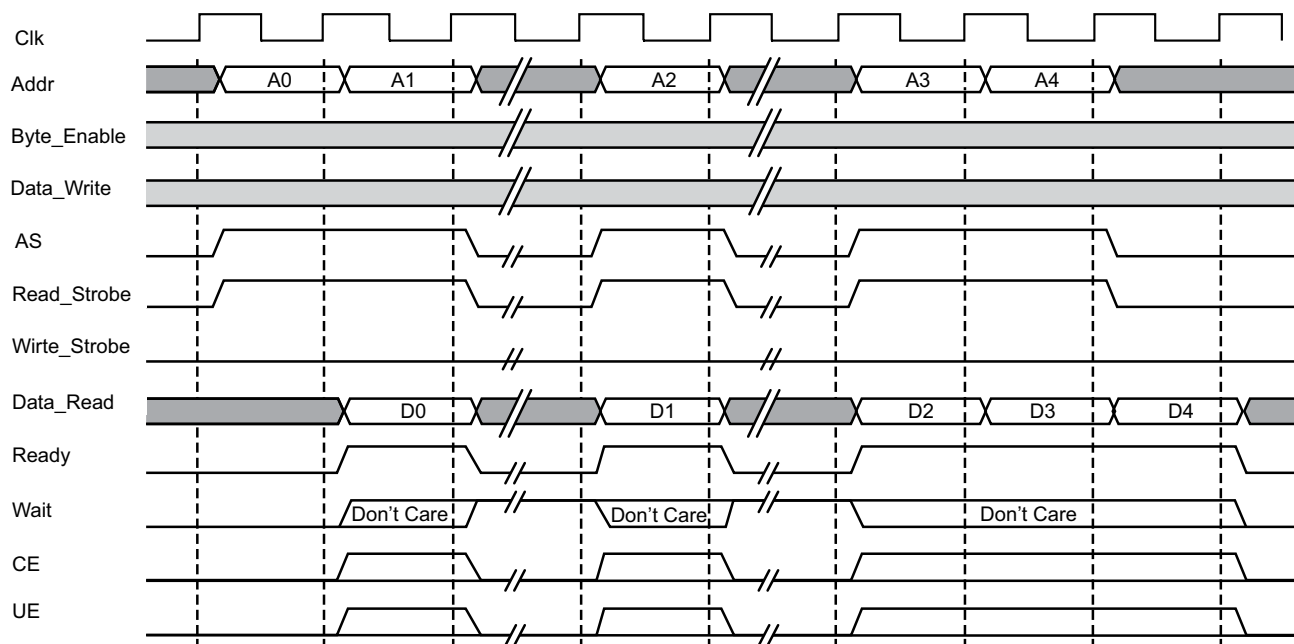
Figure 3-7: LMB Back-to-Back Read Operation
