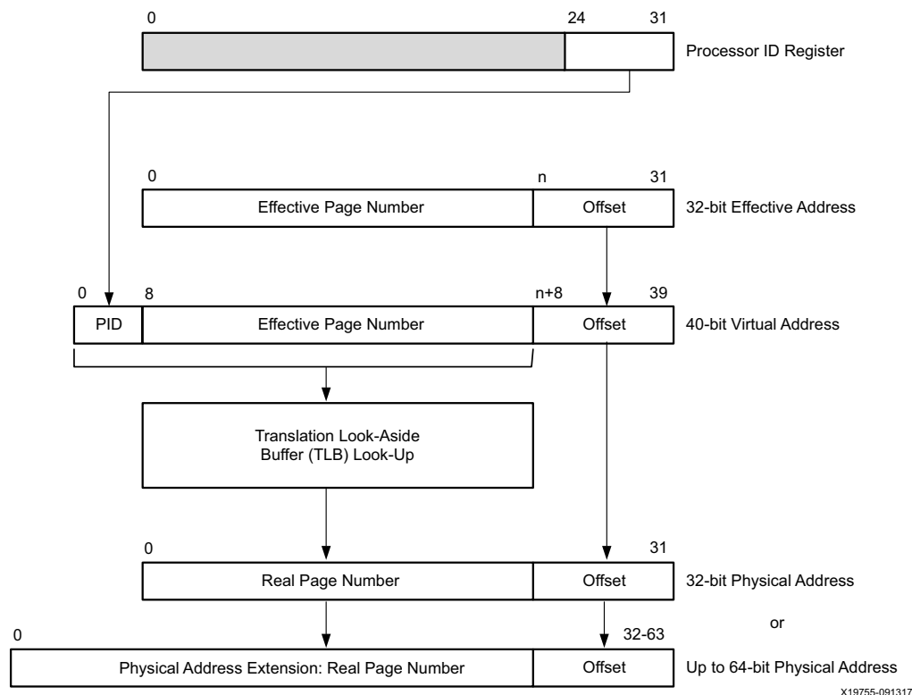
Figure 2-18: Virtual-Mode Address Translation
