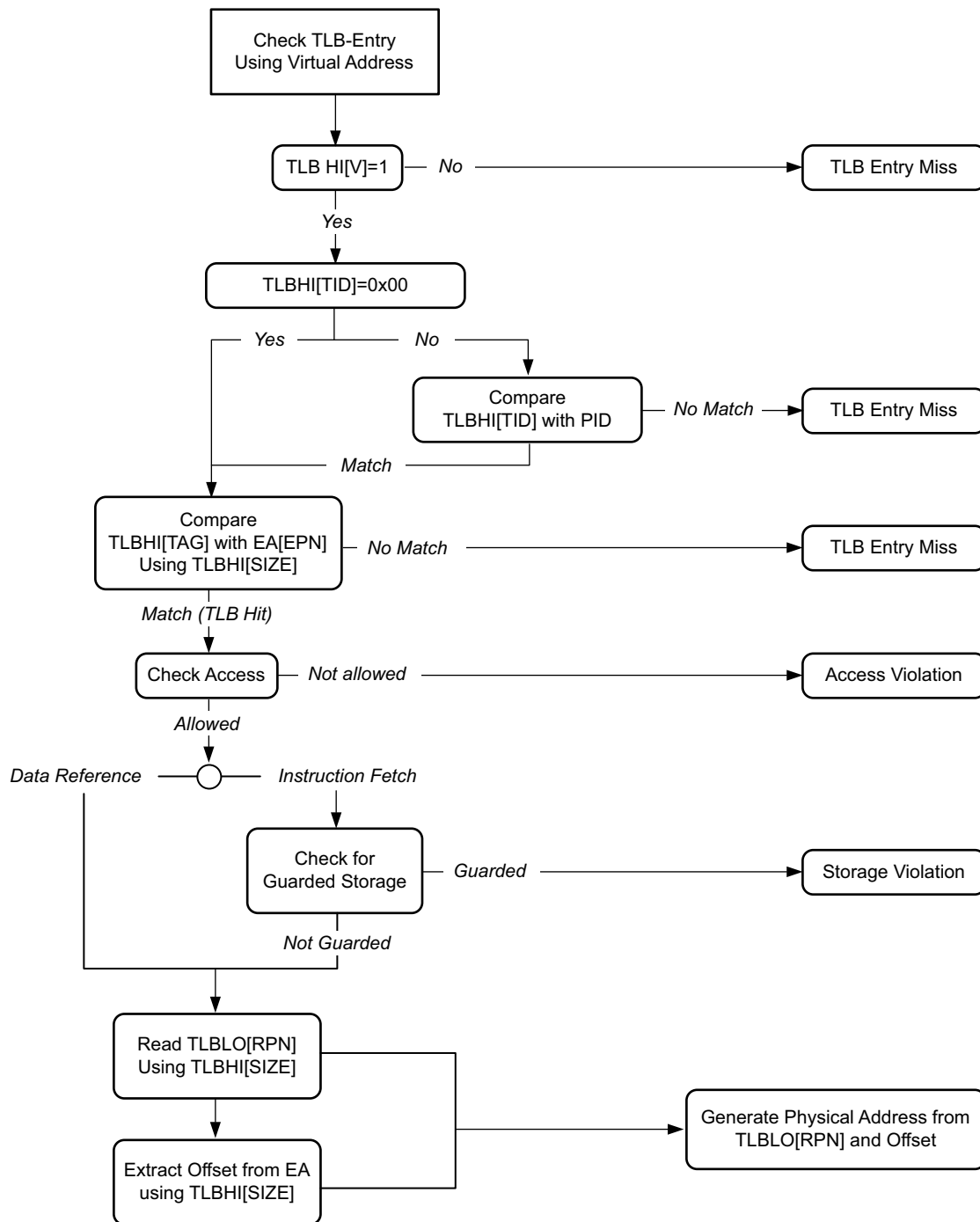
Figure 2-21: General Process for Examining a TLB Entry
