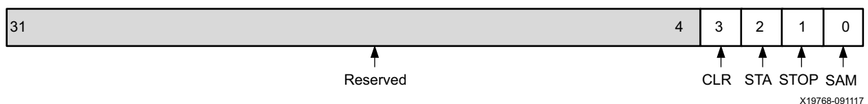
Figure 2-32: Trace Command Register
