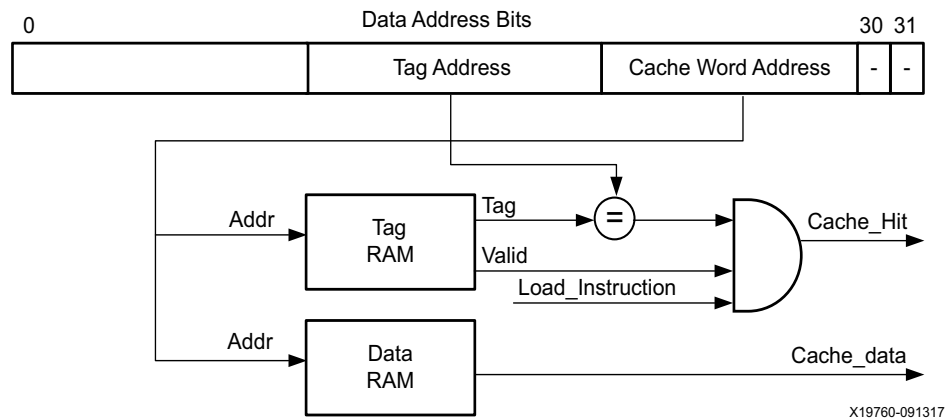
Figure 2-23: Data Cache Organization
