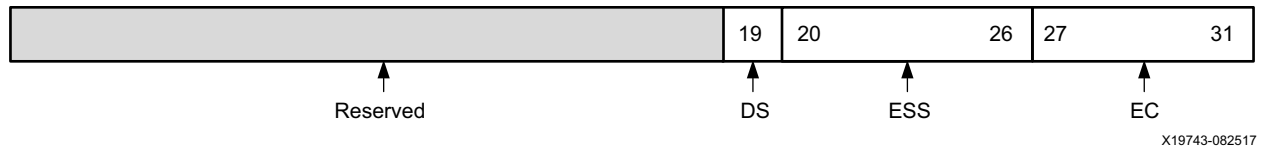
Figure 2-6: ESR
