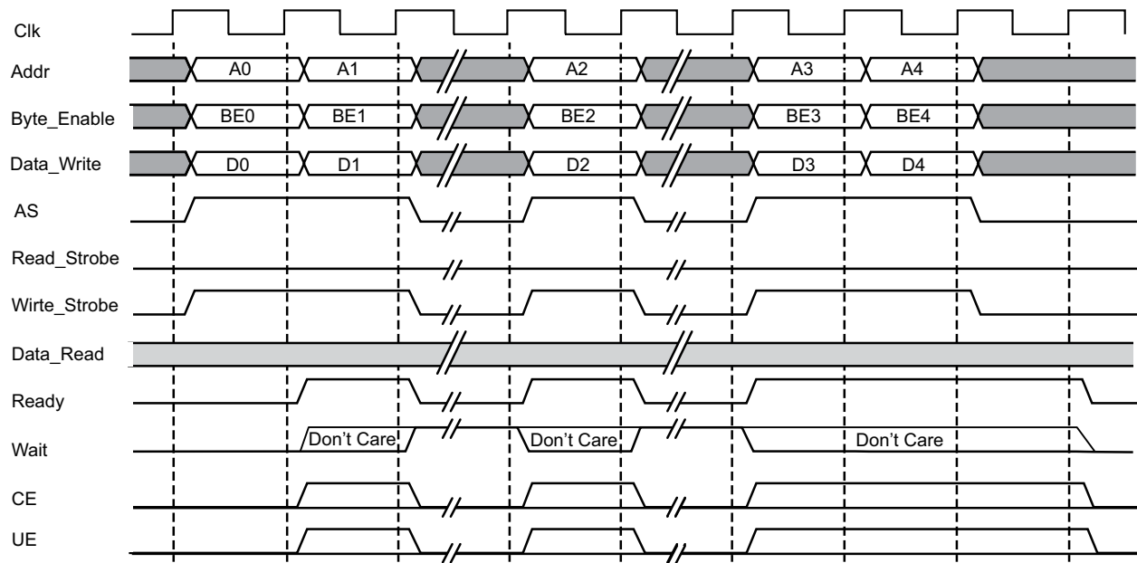
Figure 3-8: LMB Back-to-Back Write Operation
