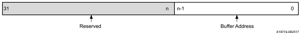
Figure 2-38: Profiling Buffer Address Register
