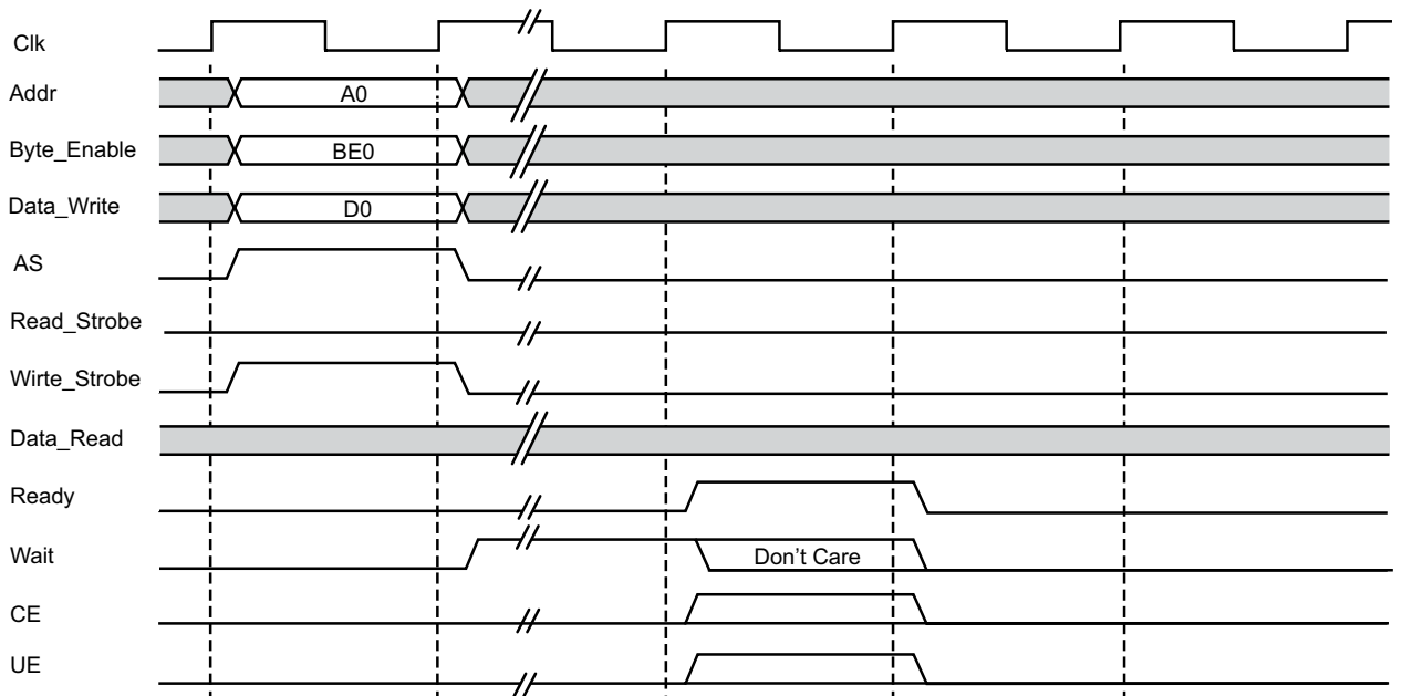
Figure 3-5: LMB Generic Write Operation, N Wait State
