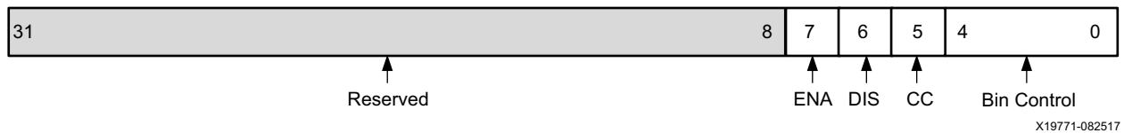
Figure 2-35: Profiling Control Register
