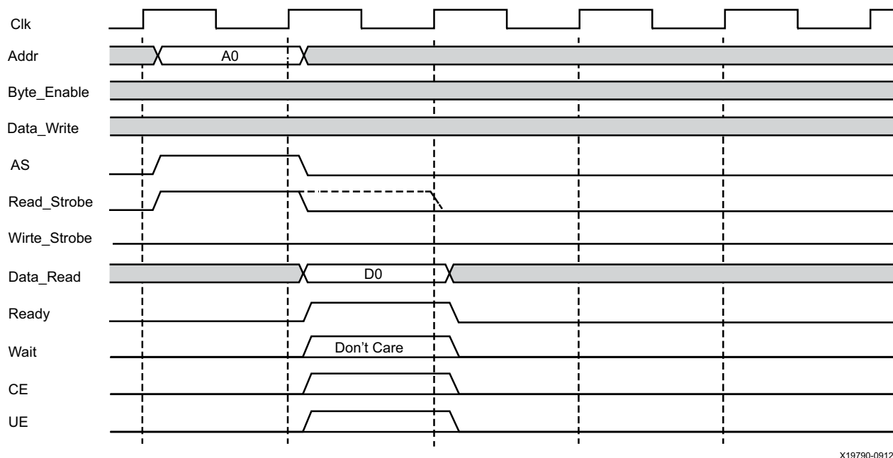
Figure 3-6: LMB Generic Read Operation, 0 Wait States
