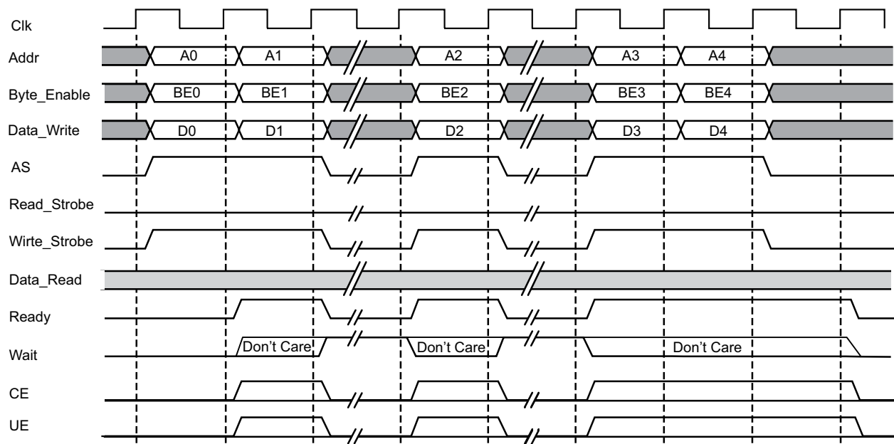
Figure 3-8: LMB Back-to-Back Write Operation
