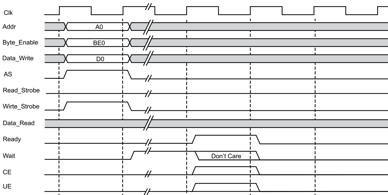
Figure 3-5: LMB Generic Write Operation, N Wait State
