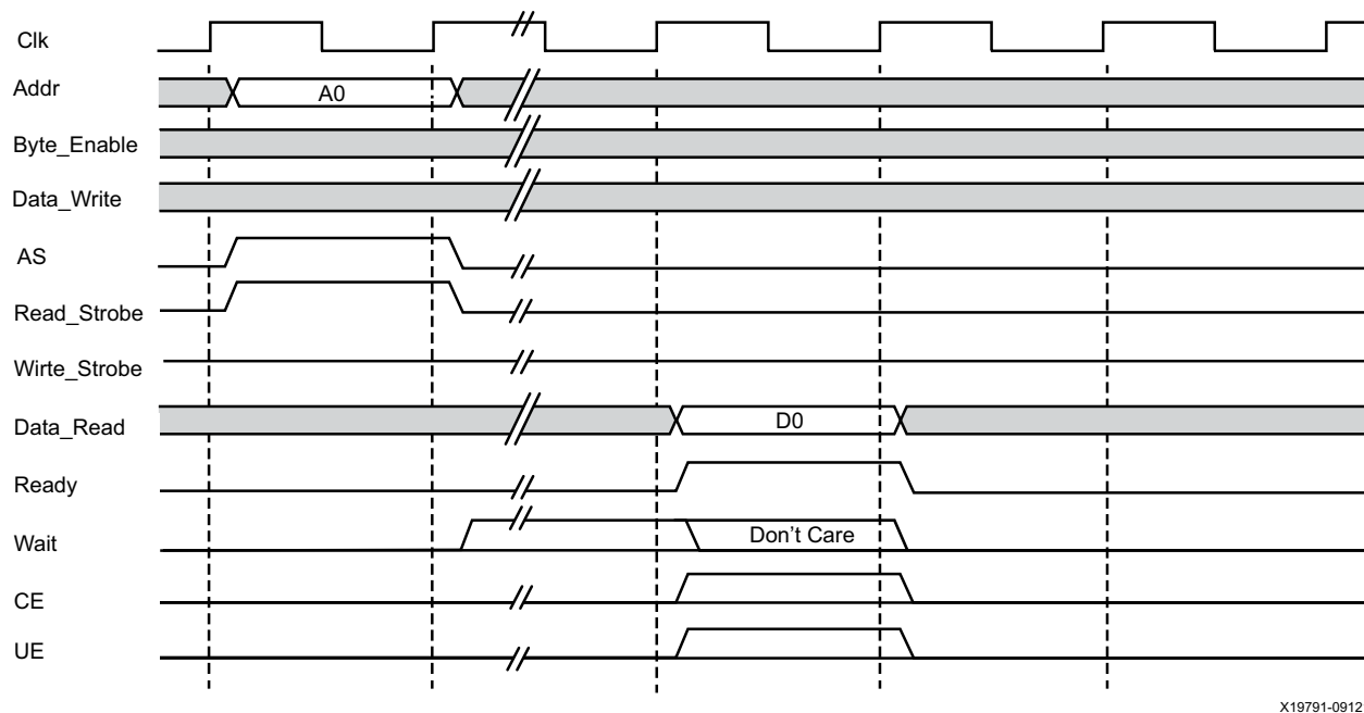
Figure 3-7: LMB Generic Read Operation, N Wait States
