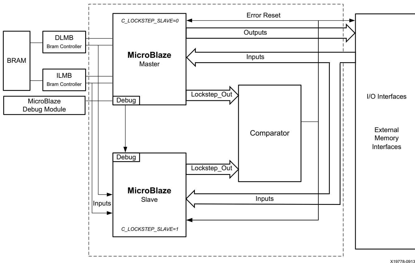
Figure 2-42: Lockstep Error Detection Application
