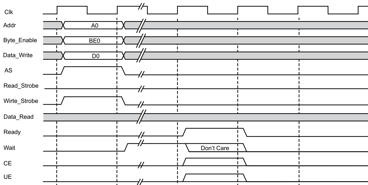
Figure 3-5: LMB Generic Write Operation, N Wait States
