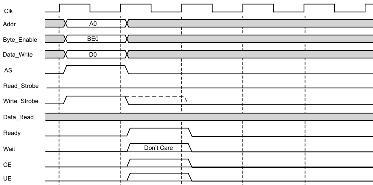
Figure 3-4: LMB Generic Write Operation, 0 Wait States
