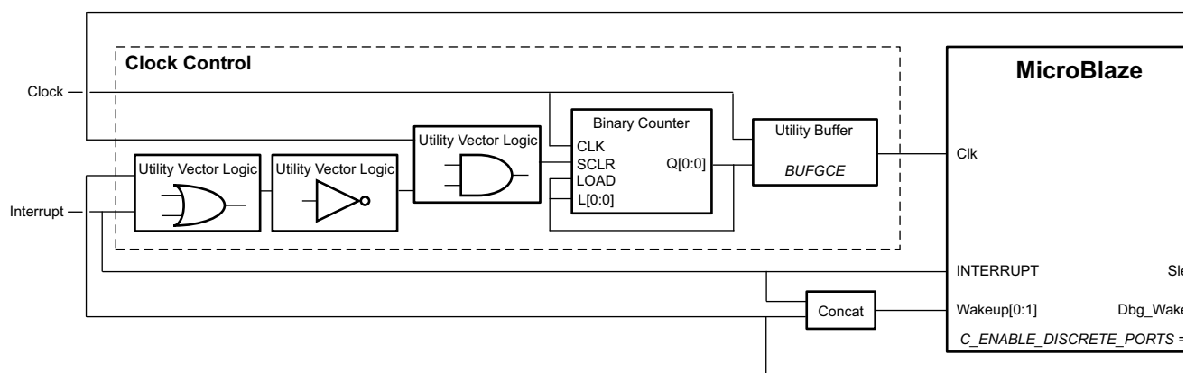
Figure 3-2: Sleep Clock Control Block Diagram
