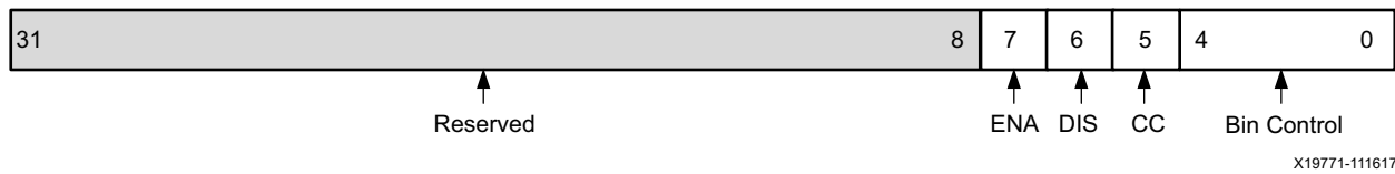
Figure 2-36: Profiling Control Register
