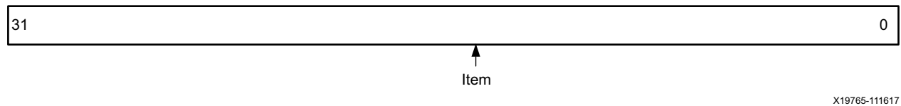
Figure 2-30: Performance Counter Data Read Register
