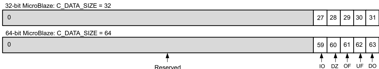
Figure 2-8: FSR
