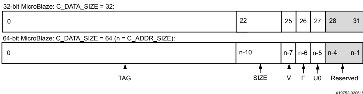
Figure 2-15: TLBHI
