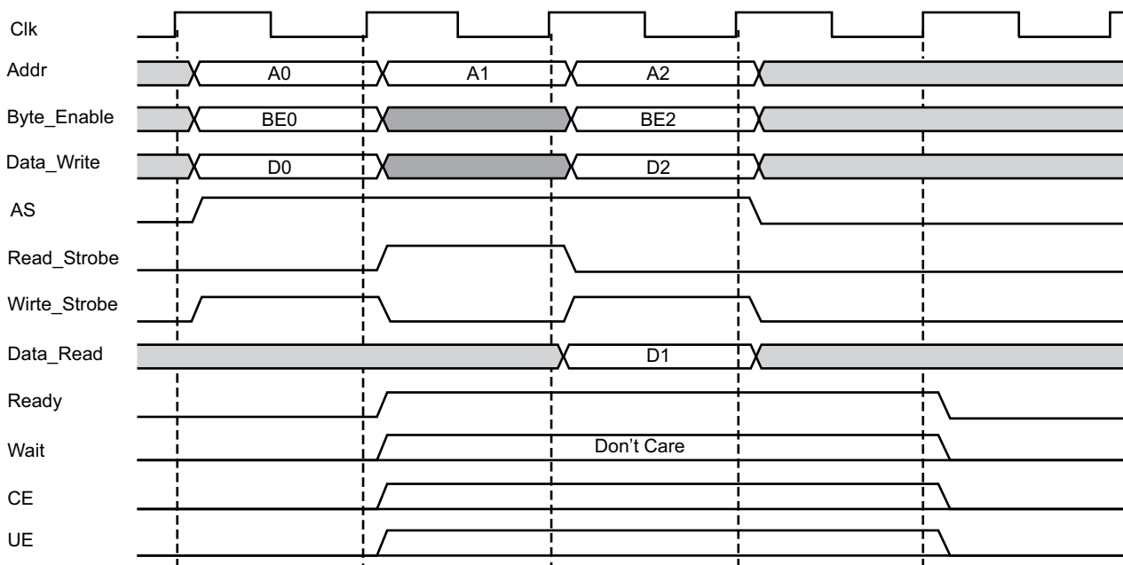
Figure 3-10: Back-to-Back Mixed Write/Read Operation, 0 Wait States
