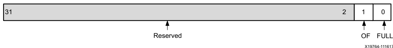
Figure 2-29: Performance Counter Status Register
