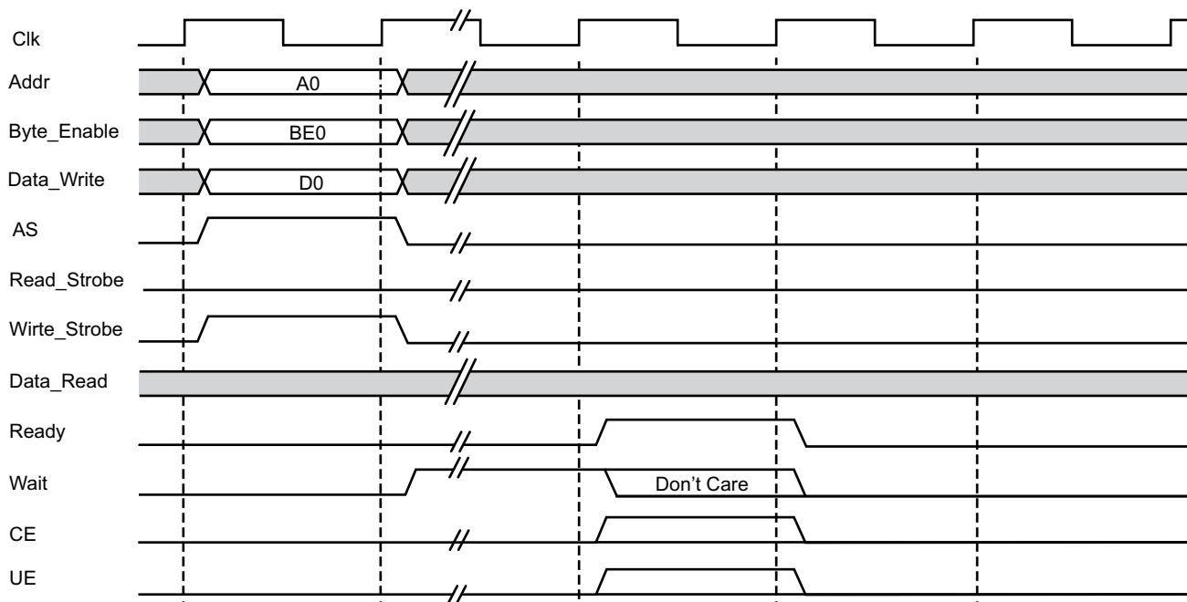
Figure 3-5: LMB Generic Write Operation, N Wait States
