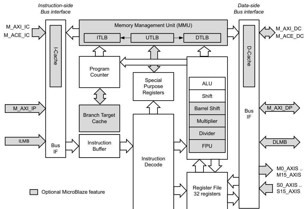
Figure 2-1: MicroBlaze Core Block Diagram
