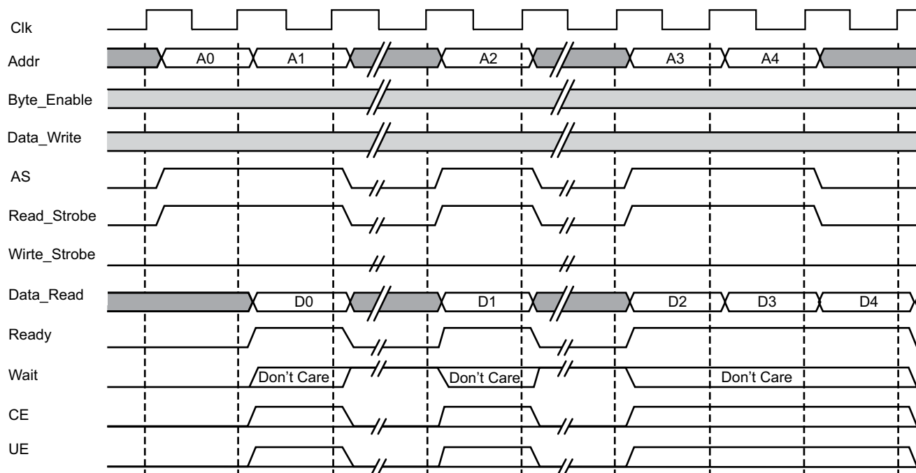
Figure 3-9: LMB Back-to-Back Read Operation
