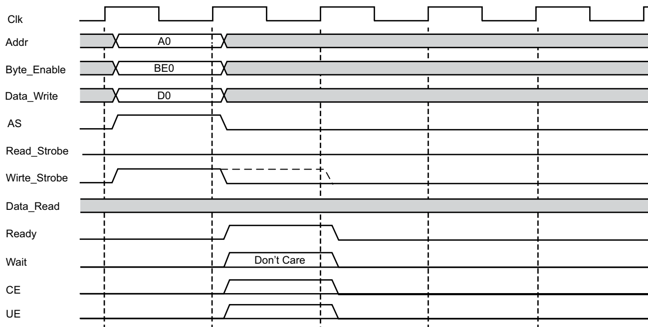
Figure 3-4: LMB Generic Write Operation, 0 Wait States
