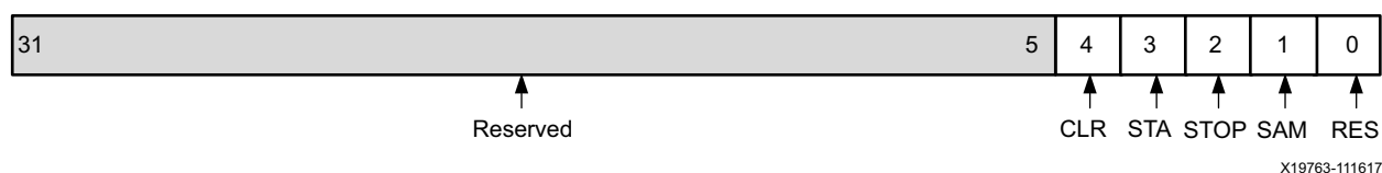
Figure 2-28: Performance Counter Command Register
