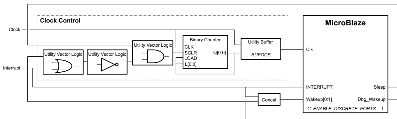
Figure 3-2: Sleep Clock Control Block Diagram
