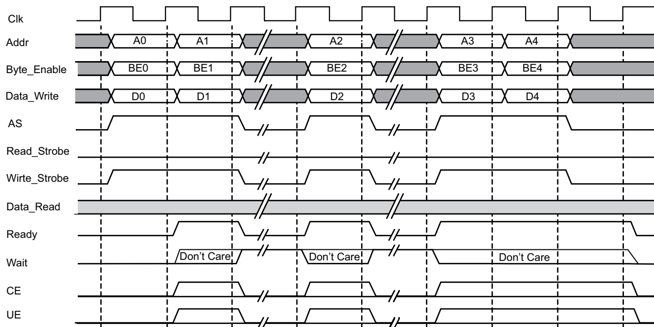
Figure 3-8: LMB Back-to-Back Write Operation
