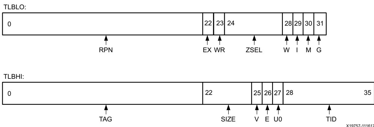
Figure 2-20: TLB Entry Format (PAE Disabled)
