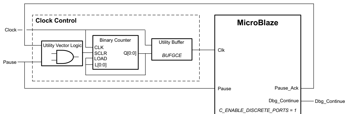
Figure 3-3: Pause Clock Control Block Diagram
