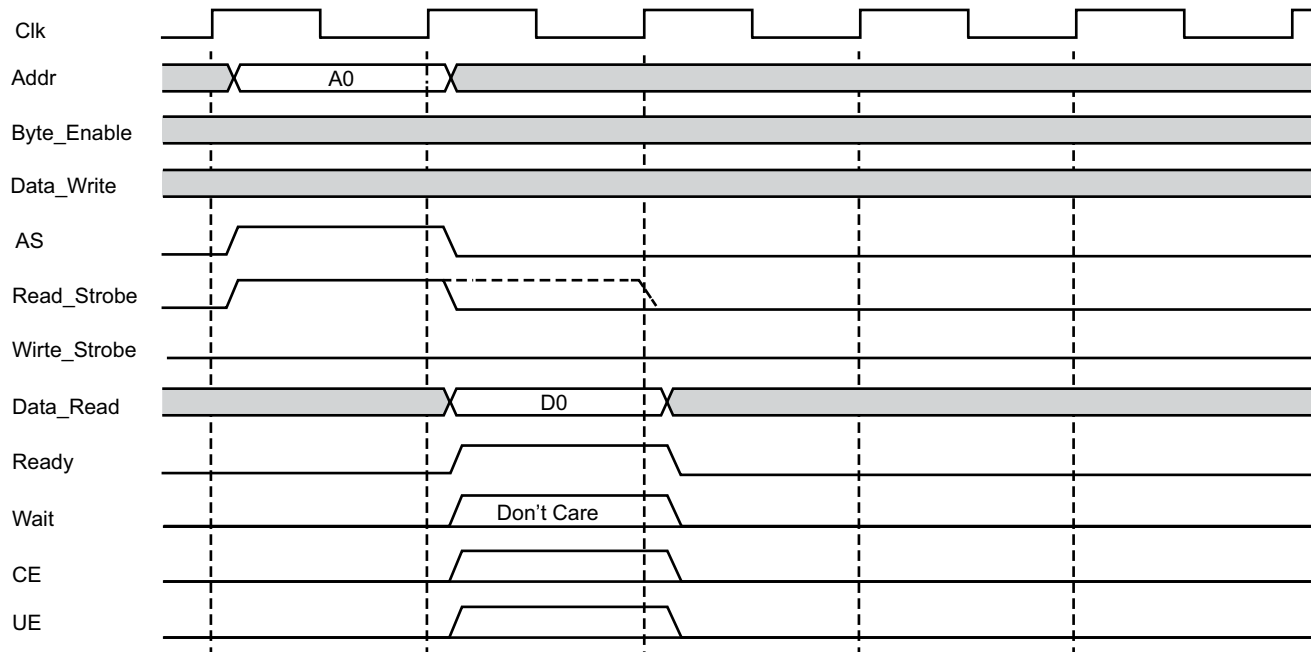
Figure 3-6: LMB Generic Read Operation, 0 Wait States
