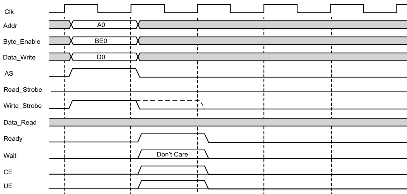
Figure 3-4: LMB Generic Write Operation, 0 Wait States
