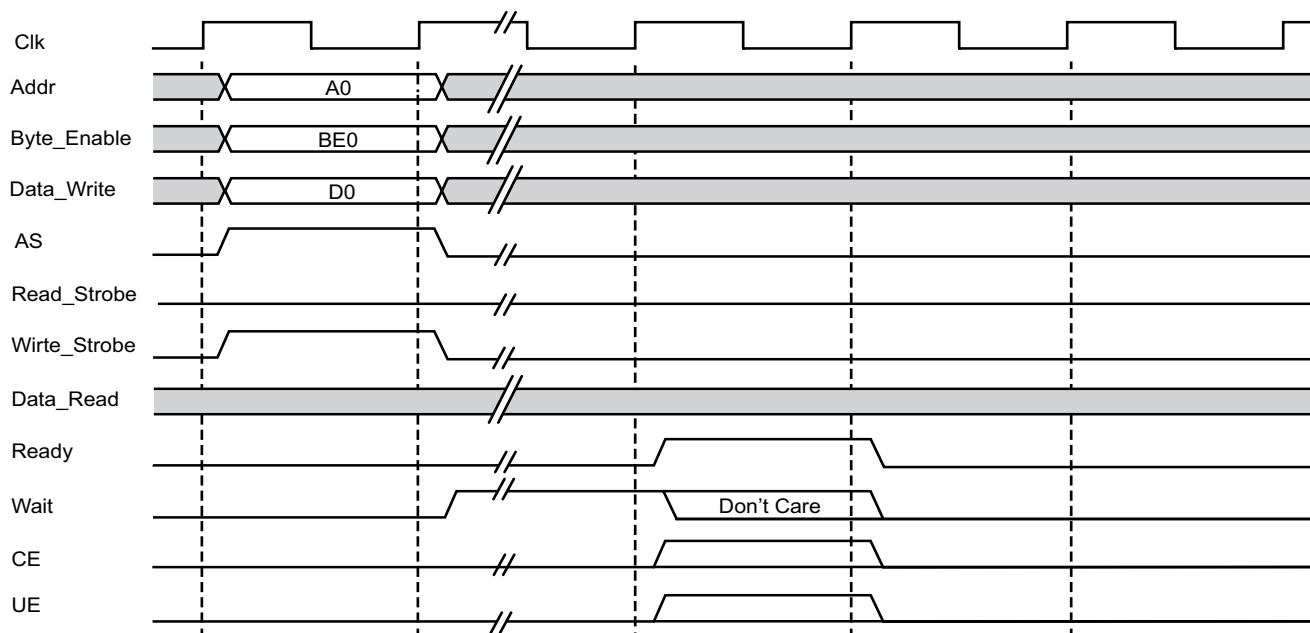
Figure 3-5: LMB Generic Write Operation, N Wait States
