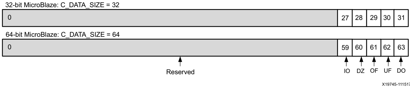
Figure 2-8: FSR
