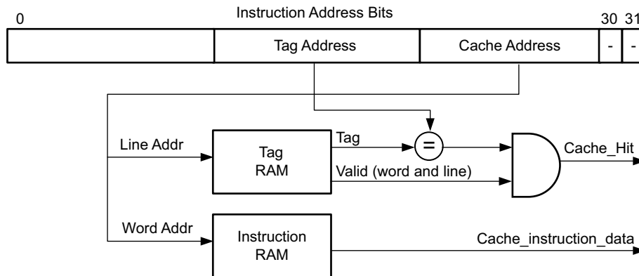
Figure 2-22: Instruction Cache Organization
