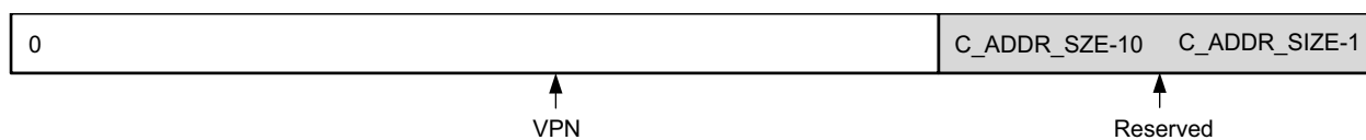
Figure 2-17: TLBSX
