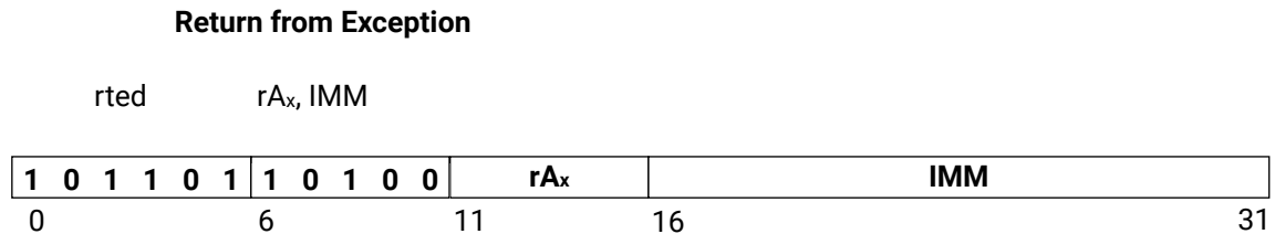
Figure 125: rted
