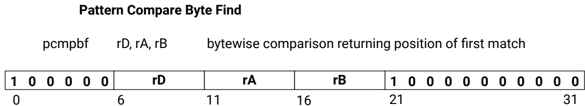
Figure 116: pcmpbf
