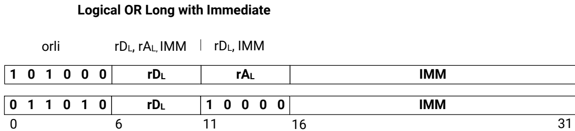
Figure 180: orli
