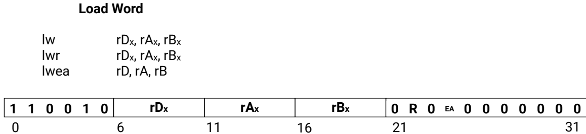
Figure 101: lw
