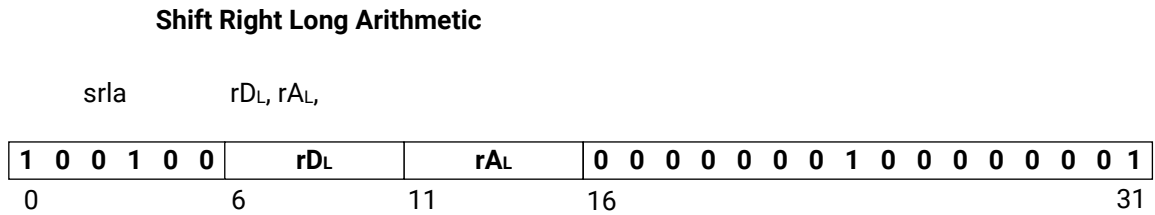
Figure 189: srla
