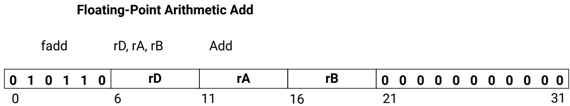
Figure 85: fadd
