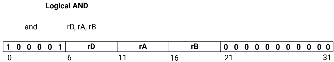
Figure 61: and
