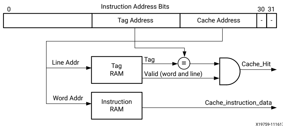
Figure 25: Instruction Cache Organization
