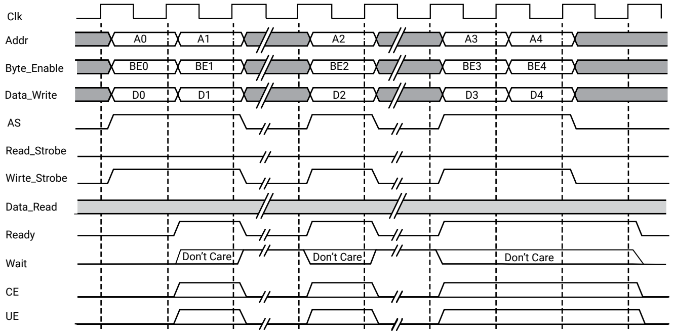
Figure 54: LMB Back-to-Back Write Operation
