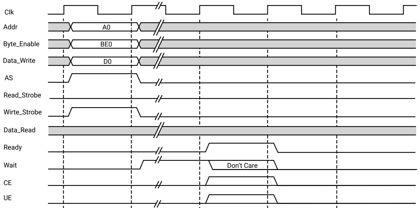
Figure 51: LMB Generic Write Operation, N Wait States
