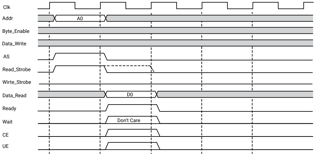
Figure 52: LMB Generic Read Operation, 0 Wait States
