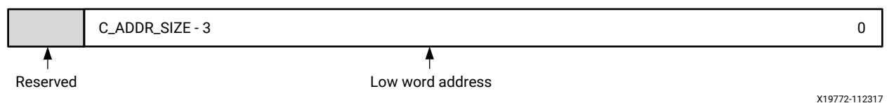
Figure 40: Profiling Low Address Register
