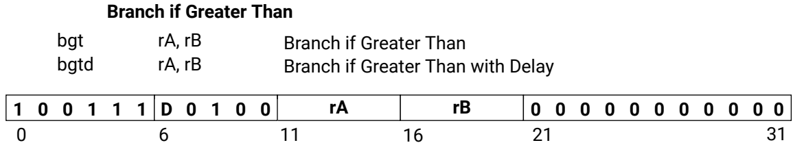
Figure 69: bgt
