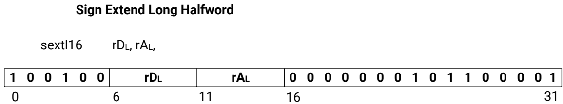
Figure 186: sextl16
