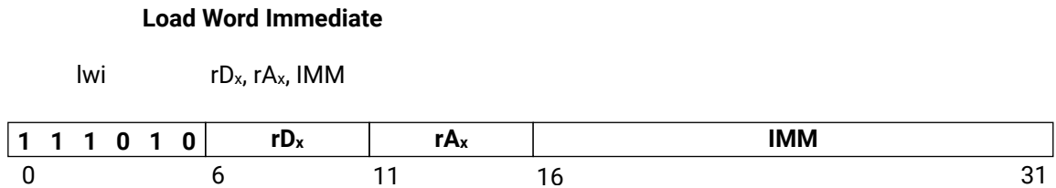
Figure 102: lwi
