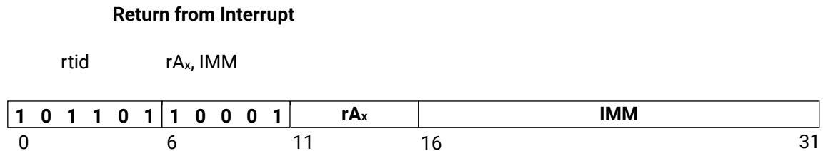
Figure 124: rtid
