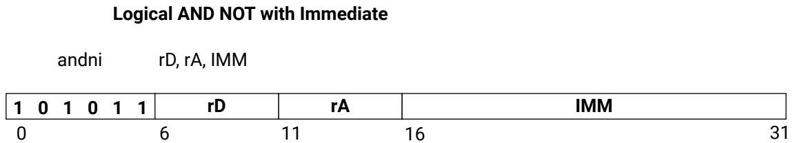
Figure 64: andni
