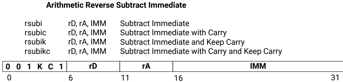
Figure 122: rsubi
