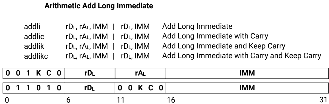
Figure 146: addli
