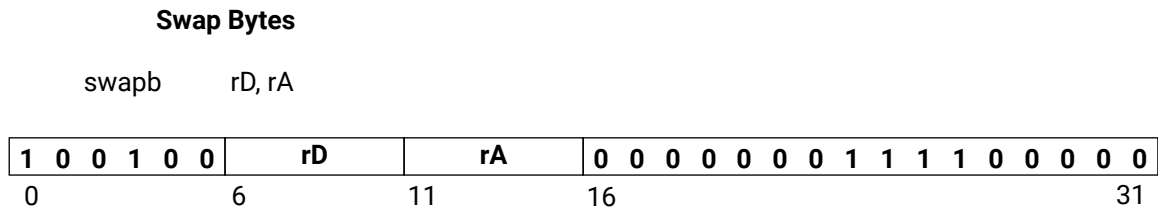
Figure 137: swapb
