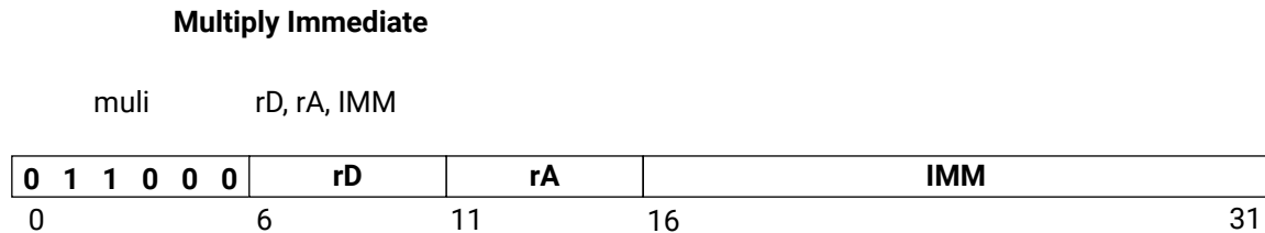
Figure 113: multi
