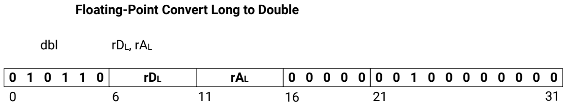
Figure 173: dbl
