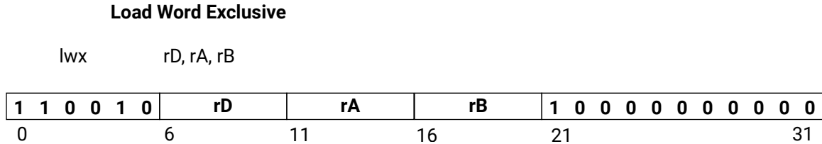
Figure 103: lwx
