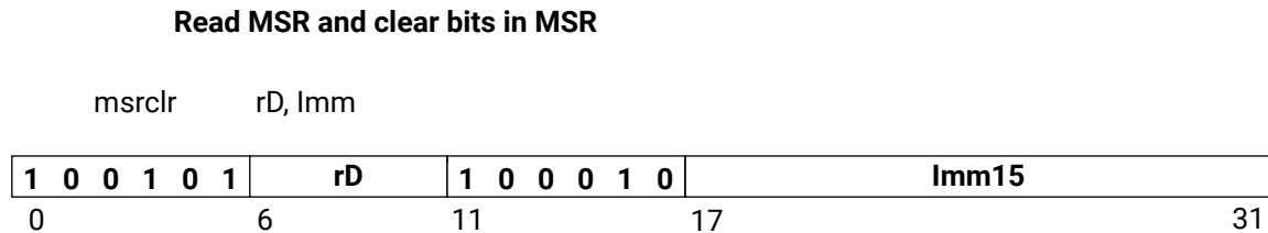
Figure 106: msrclr
