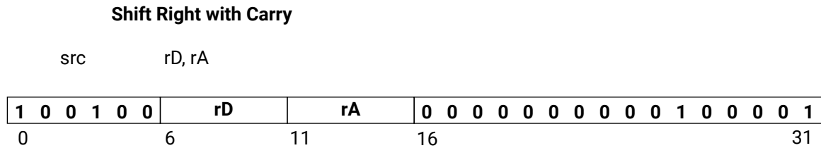
Figure 134: src
