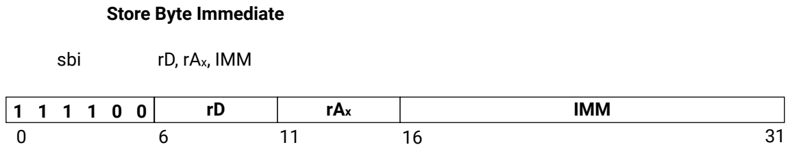
Figure 128: sbi
