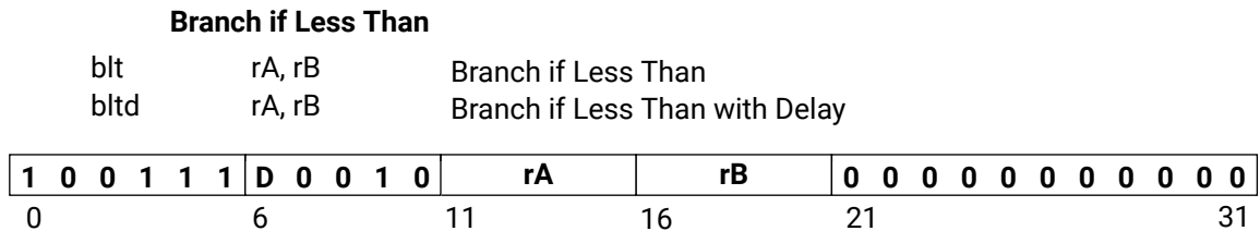
Figure 73: blt
