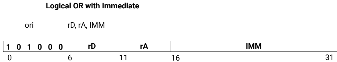
Figure 115: ori
