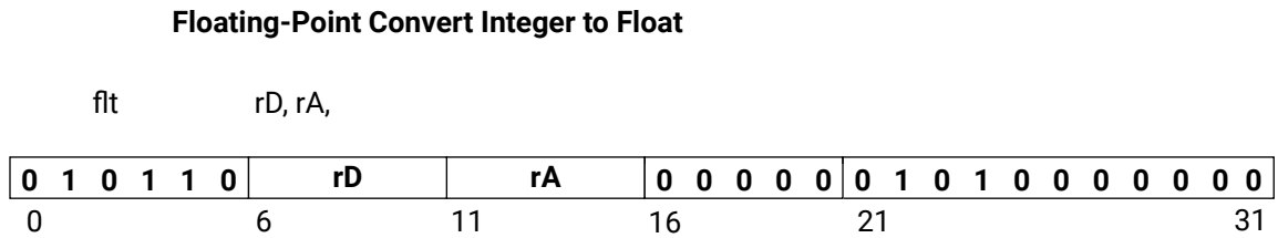
Figure 90: flt
