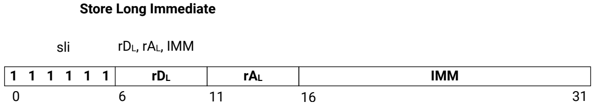
Figure 193: sli
