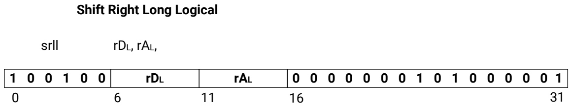
Figure 191: srl
