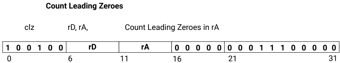
Figure 83: clz
