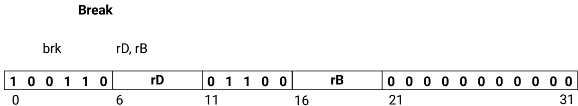
Figure 79: brk
