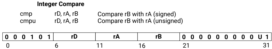
Figure 84: cmp
