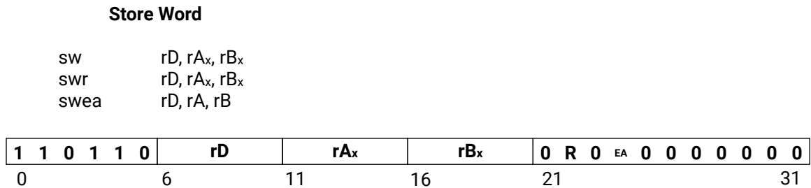
Figure 136: sw
