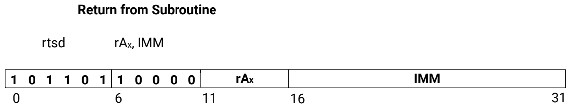
Figure 126: rtsd
