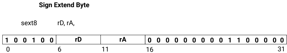
Figure 130: sext8
