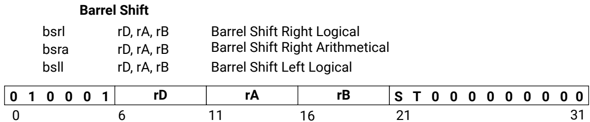
Figure 81: bs
