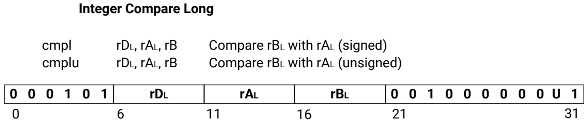
Figure 167: cmpl
