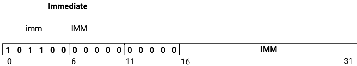
Figure 96: imm
