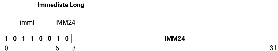
Figure 176: imml
