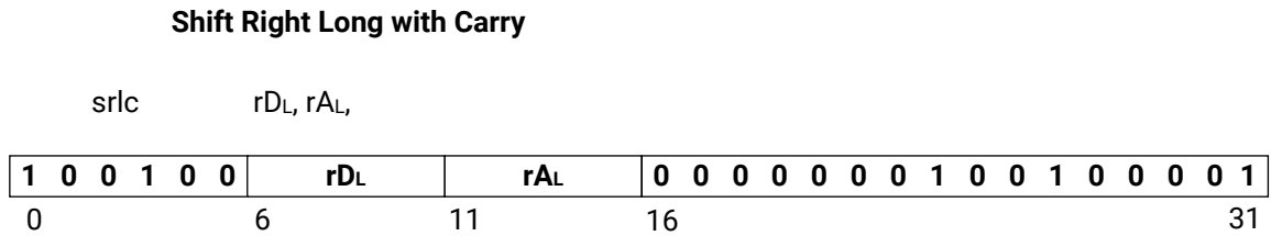
Figure 190: srlc
