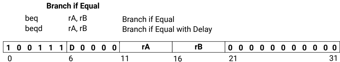
Figure 65: beq
