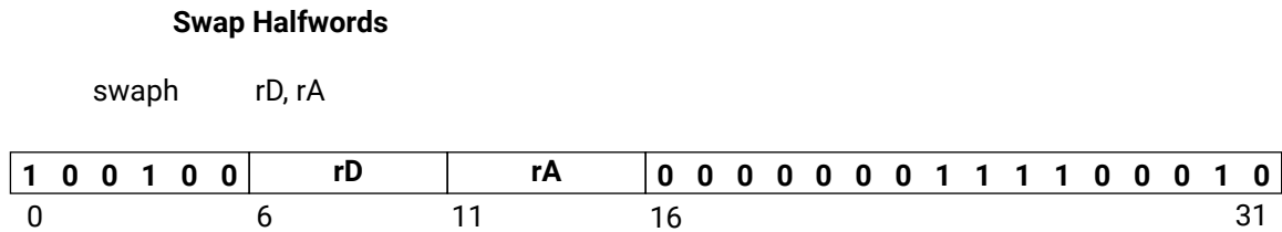
Figure 138: swaph
