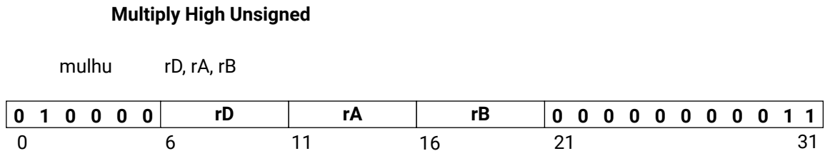
Figure 111: mulhu
