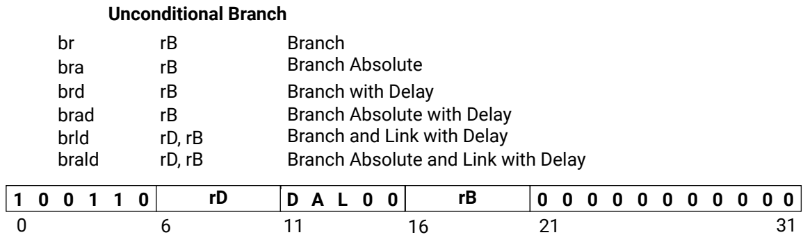
Figure 77: br
