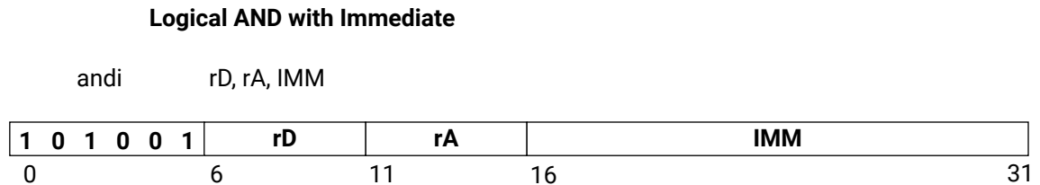
Figure 62: andi
