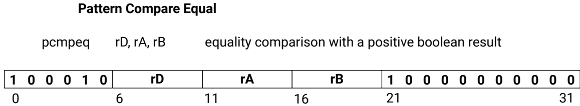
Figure 117: pcmpeq
