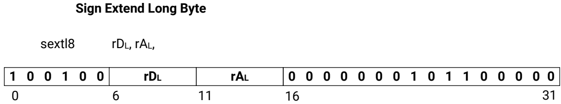
Figure 188: sextl8
