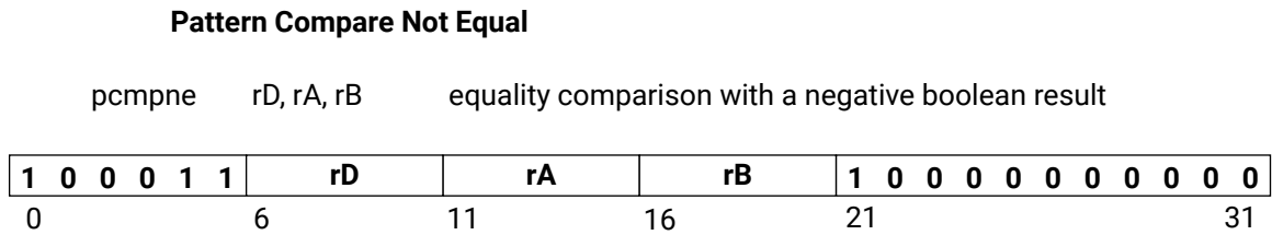
Figure 118: pcmpne
