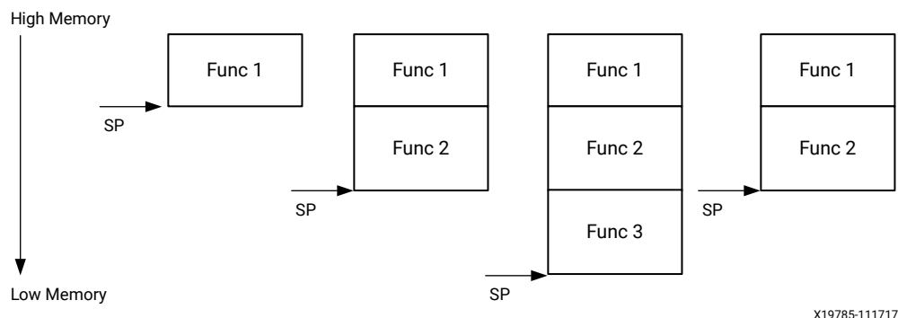
Figure 58: Stack Frame
