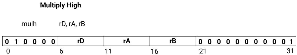
Figure 110: mulh
