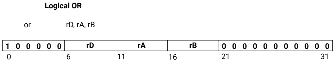
Figure 114: or
