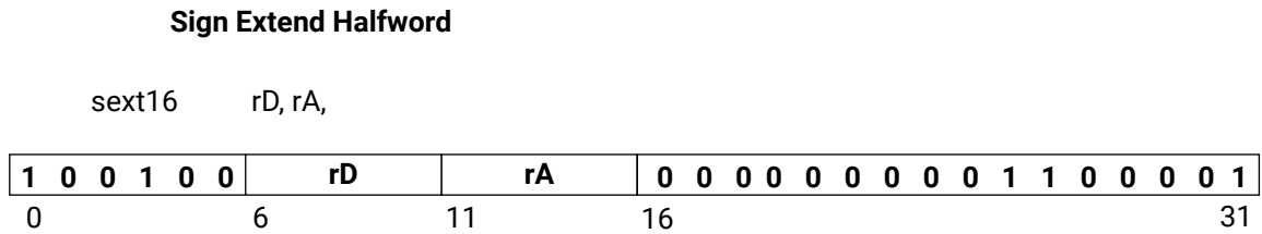
Figure 129: sext16
