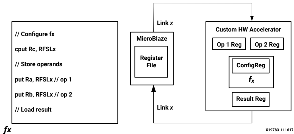
Figure 29: Stream Link Used with HW Accelerated Function
