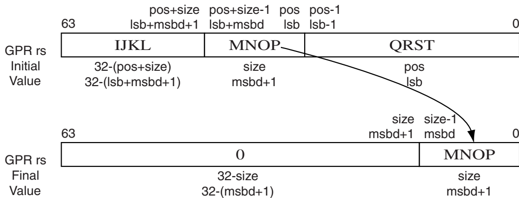
Figure 5.4 Operation of the DEXTM Instruction
