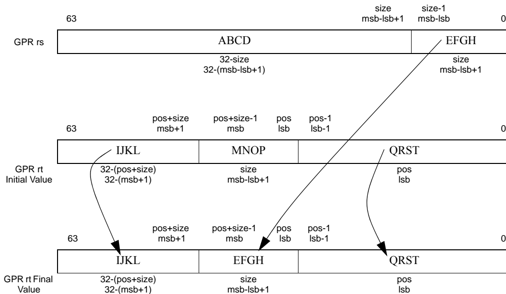
Figure 5.9 Operation of the DINSM Instruction
