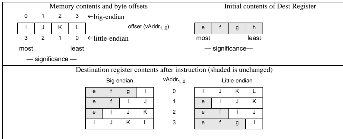
Figure 5.12 Bytes Loaded by LWRE Instruction
