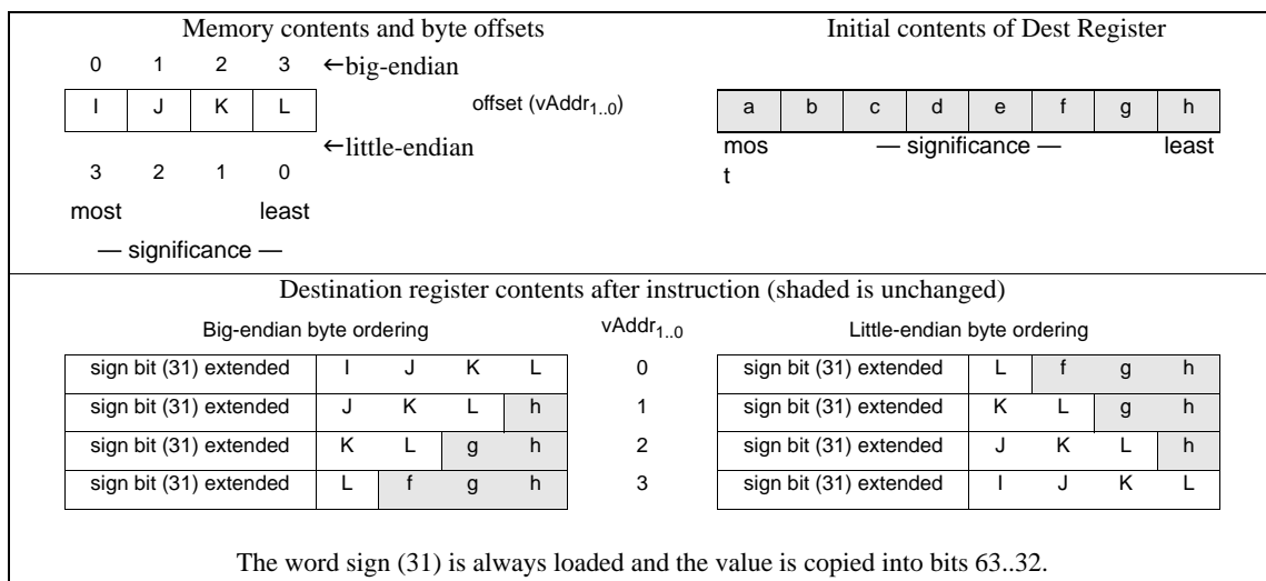
Figure 5.3 Bytes Loaded by LWL Instruction
