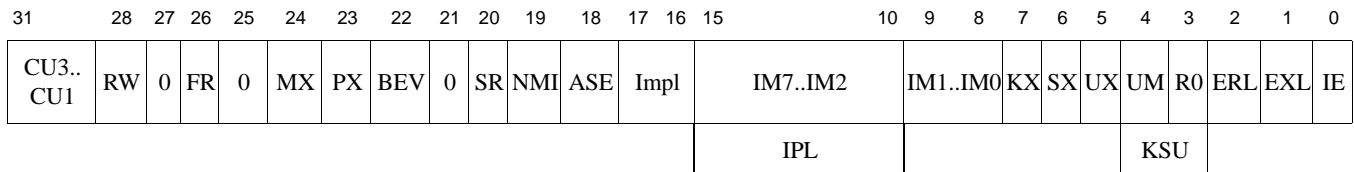
Figure 9.35 Status Register Format for Release 6
