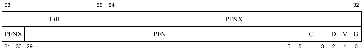
Figure 9-5 EntryLo0, EntryLo1 Register Format in Release 2 of the Architecture
