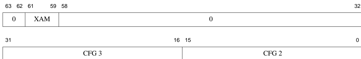
Figure 9.19 SegCtl1 Register Format (CP0 Register 5, Select 3)
