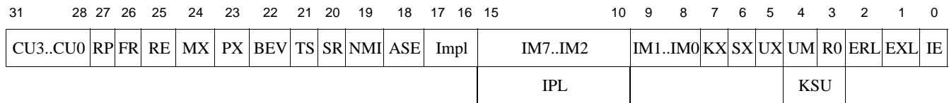
Figure 9.34 Status Register Format for Pre-Release 6
