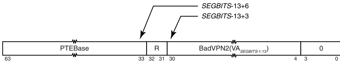
Figure 9.62 XContext Register Format when Config3_{CTXTC} = 0
