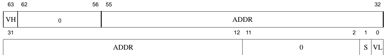
Figure 9-58 MAAR Register Format
