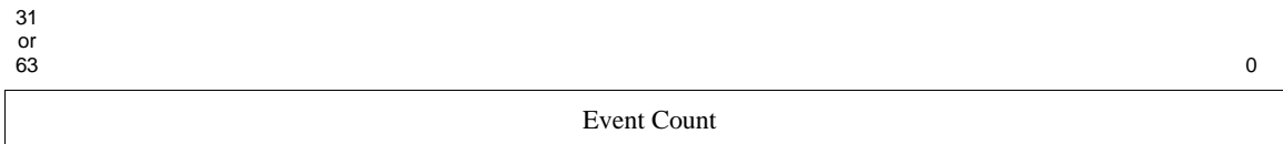
Figure 9.65 Performance Counter Counter Register Format
