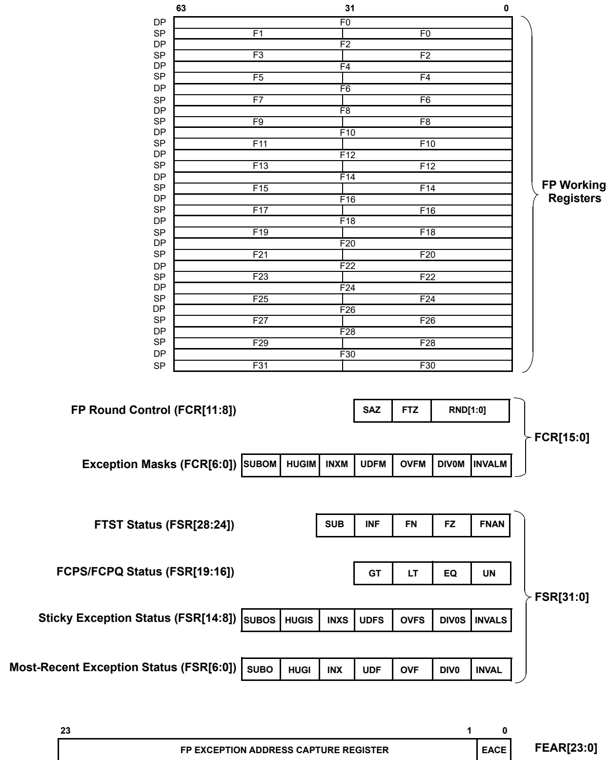
Figure 1-2. FPU Programmer's Model
