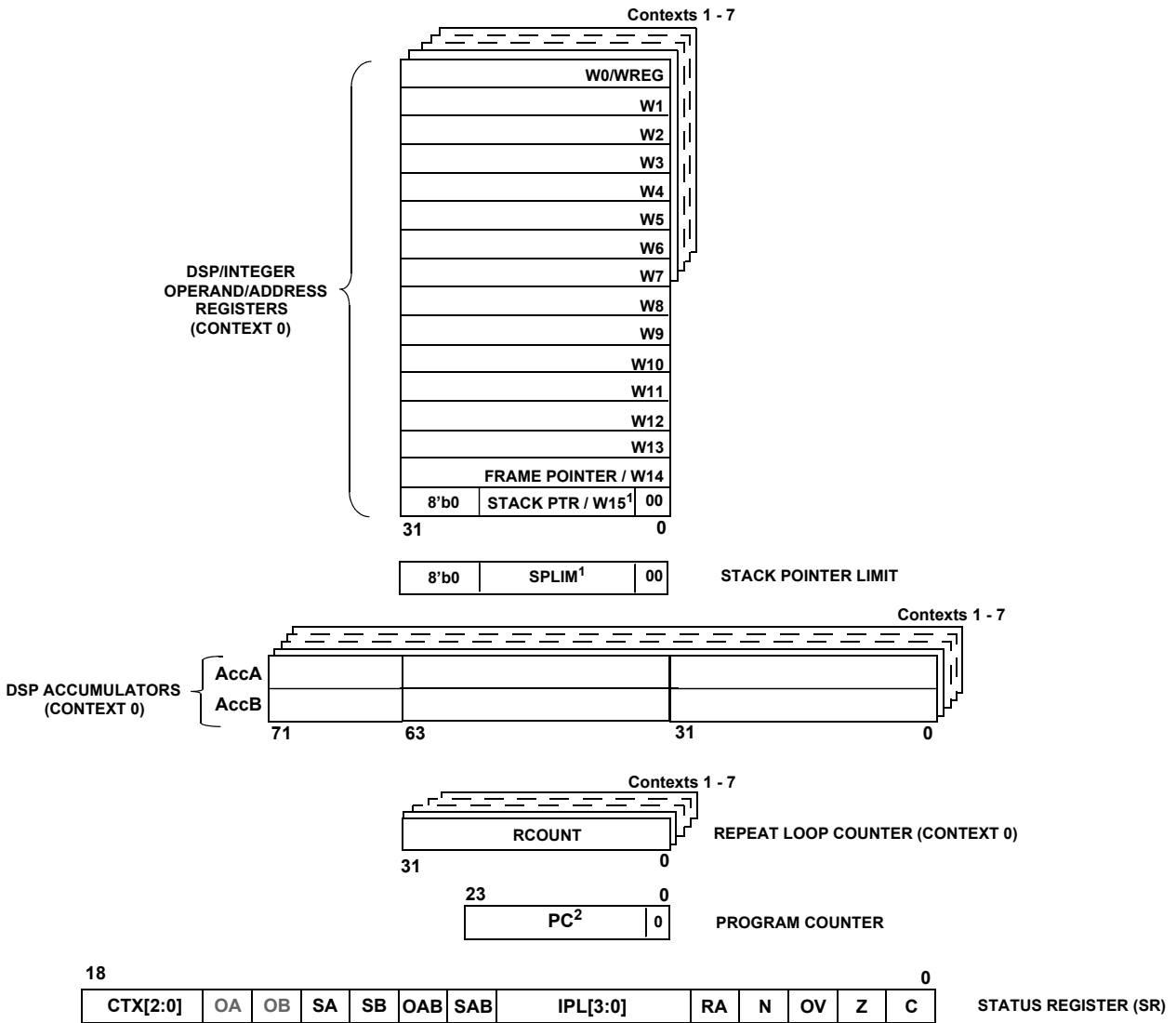
Figure 1-3. dsPIC33A Programmer's Model
