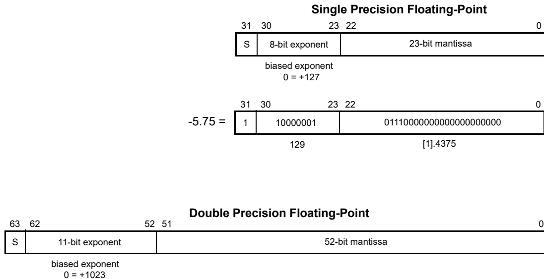
Figure 1-1. IEEE Floating-Point Data Formats and Single Precision Example
