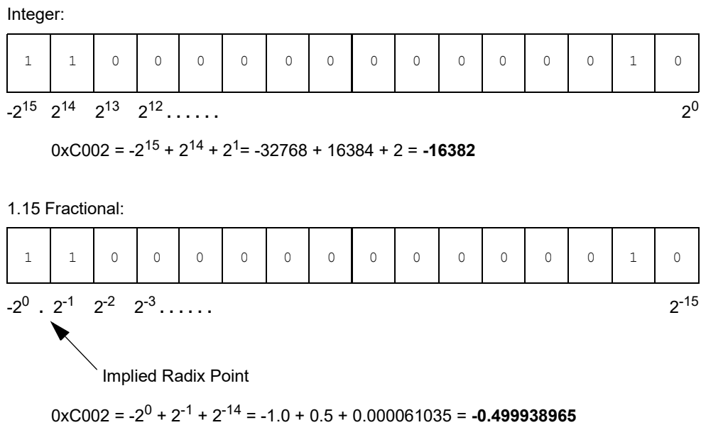
Figure 3-12. Different Representations of 0xC002
