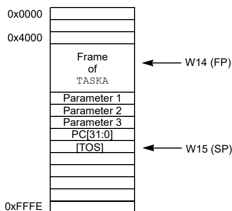
Figure 3-9. Stack After "CALL COMPUTE" Executes
