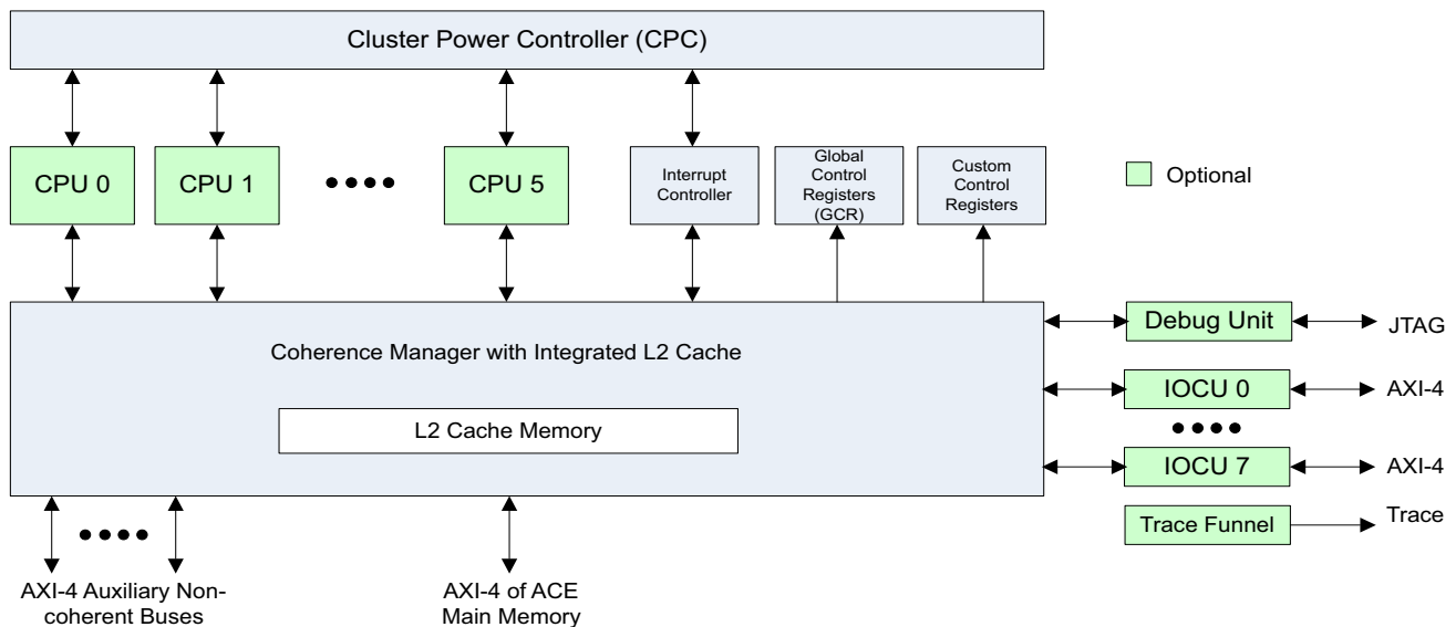
Figure 1.1 Block Diagram of Single Cluster P8700 Multiprocessing System
