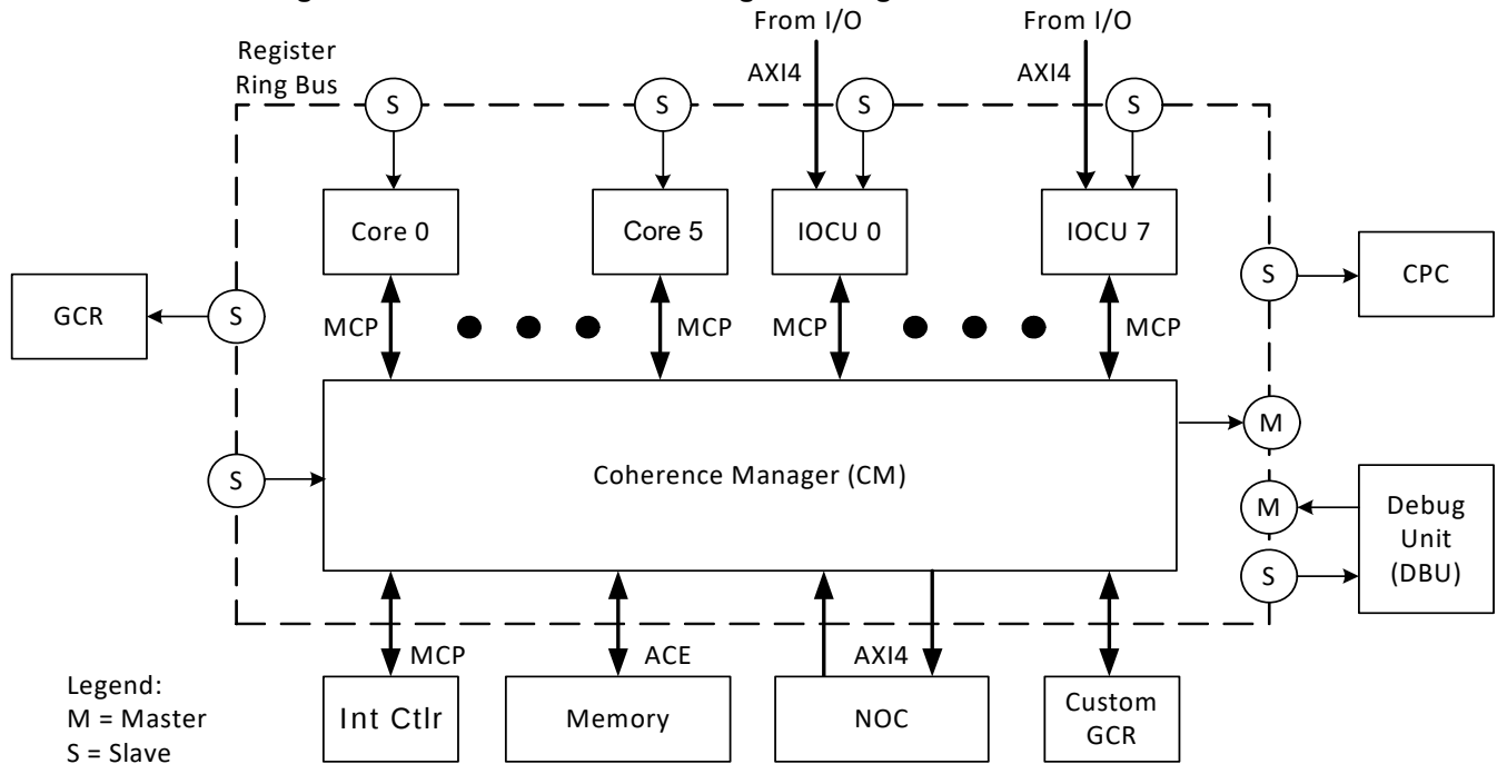
Figure 5.1 Interface Ports and Register Ring Bus Interface to the CM
