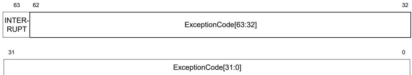
Figure 7.2 Machine Cause Register Bit Assignments — RV64
