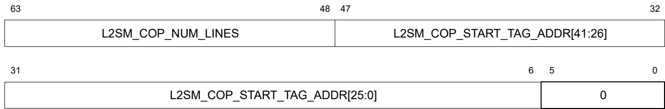
Figure 5.33 Global L2SM Tag Address CacheOp Register Bit Assignments
