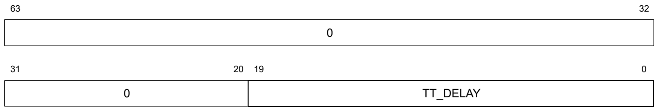
Figure 5.35 Global Timeout Timer Limit Register Bit Assignments
