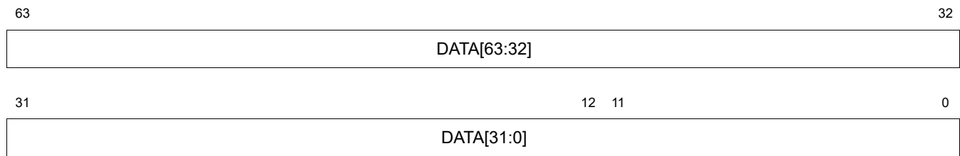
Figure 5.30 Global L2 Data Register Bit Assignments
