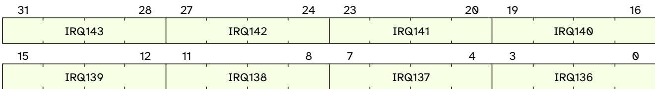
Figure 27. qc.mclcivl17 format
