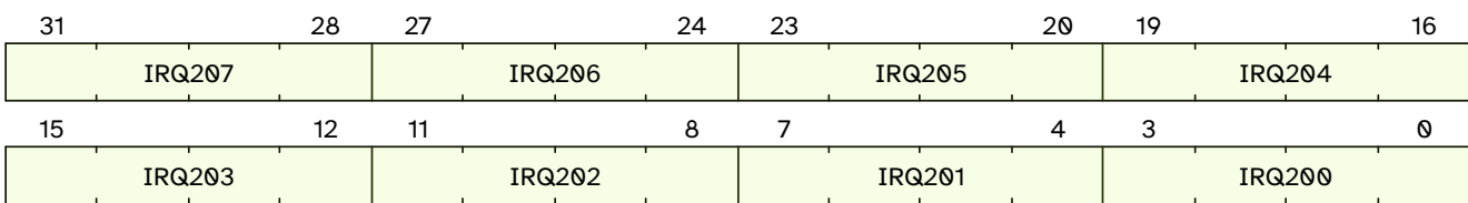
Figure 35. qc.mclivil25 format
