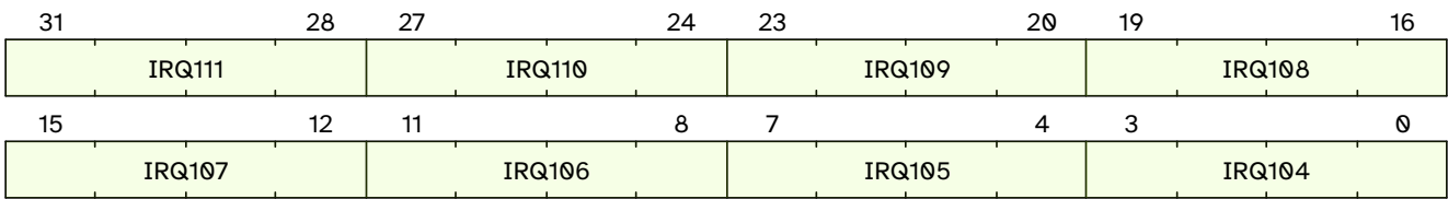
Figure 23. qc.mclcivl13 format
