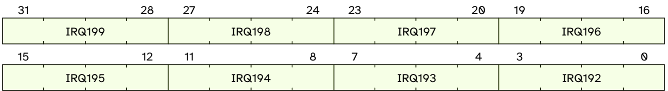
Figure 34. qc.mclivil24 format
