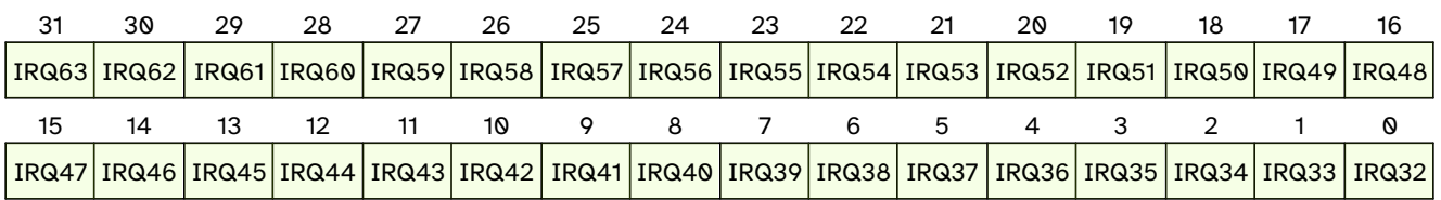
Figure 3. qc.mclicie1 format
