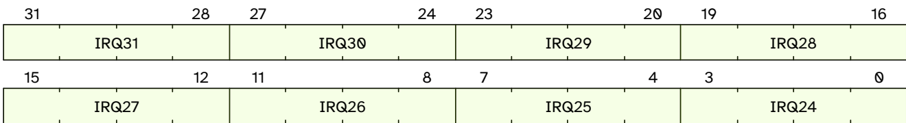
Figure 13. qc.mclcivl03 format
