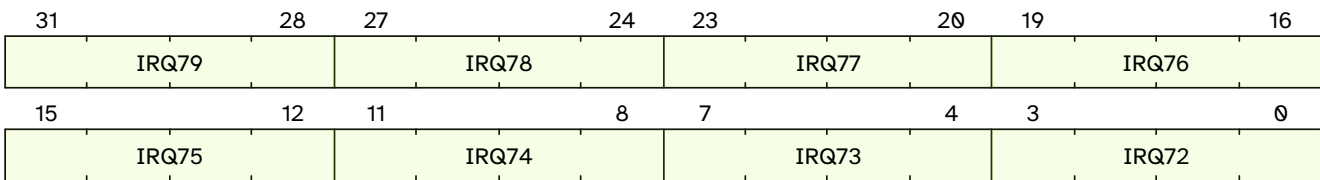
Figure 19. qc.mclcivl09 format
