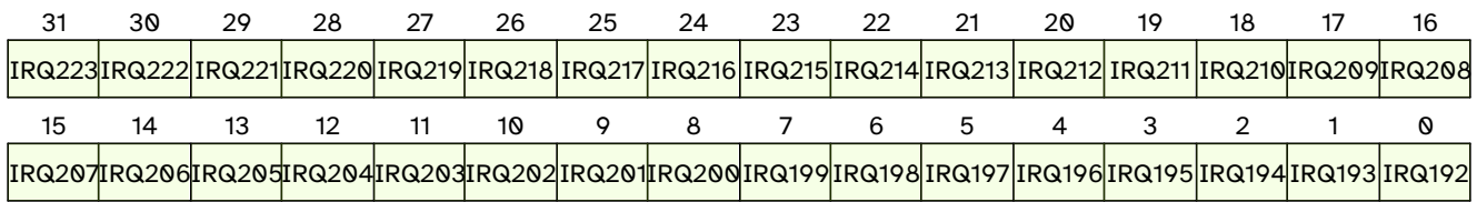
Figure 48. qc.mclicip6 format
