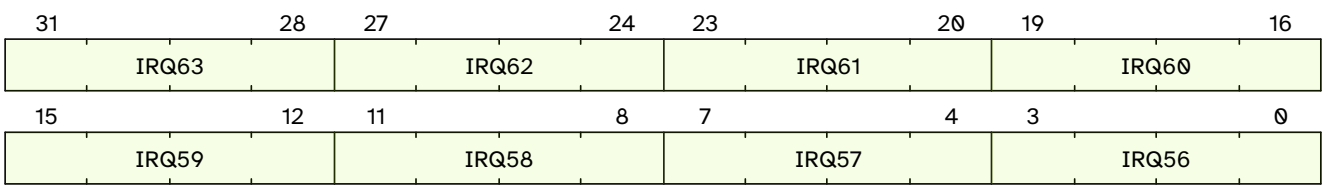
Figure 17. qc.mclcivl07 format
