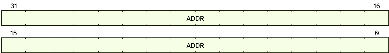
Figure 60. qc.mwpstartaddr1 format
