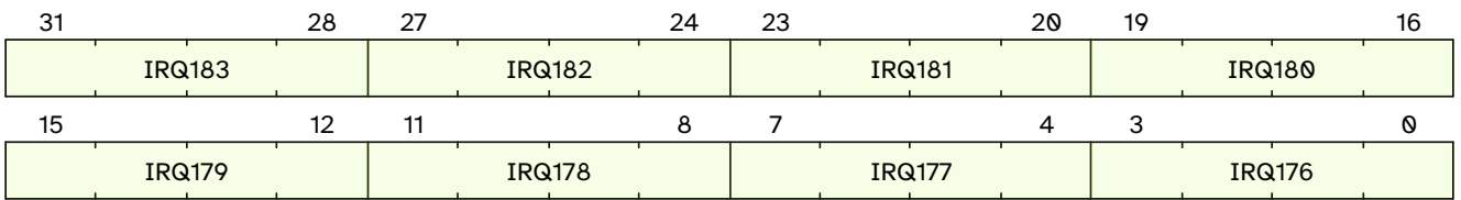
Figure 32. qc.mclcivl22 format
