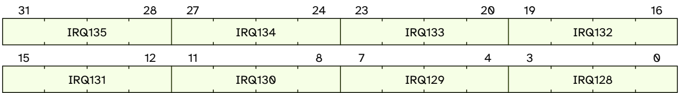
Figure 26. qc.mclcivl16 format
