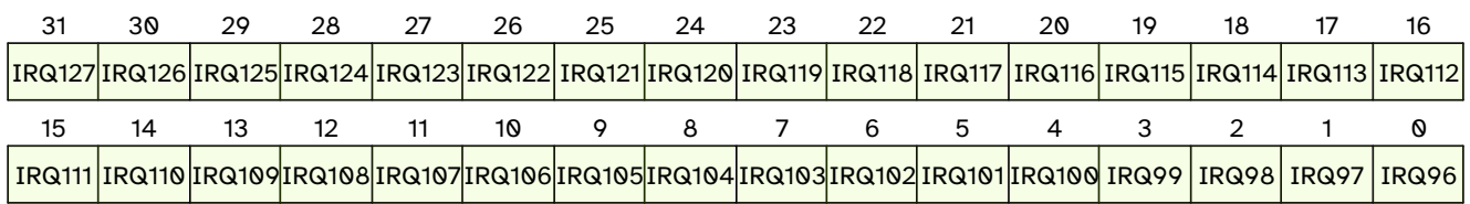
Figure 5. qc.mclcie3 format
