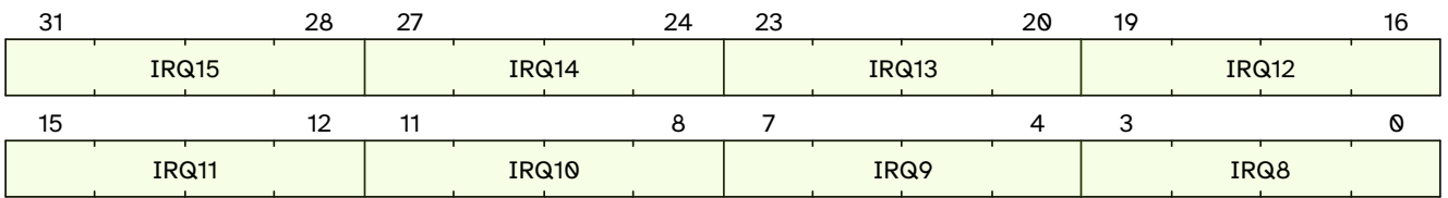
Figure 11. qc.mclcivl01 format
