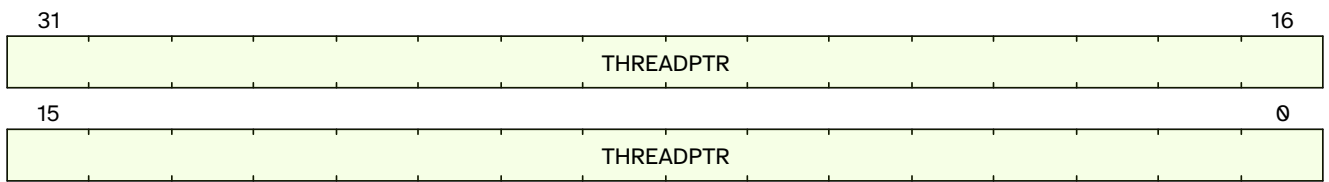
Figure 54. qc.mthreadptr format
