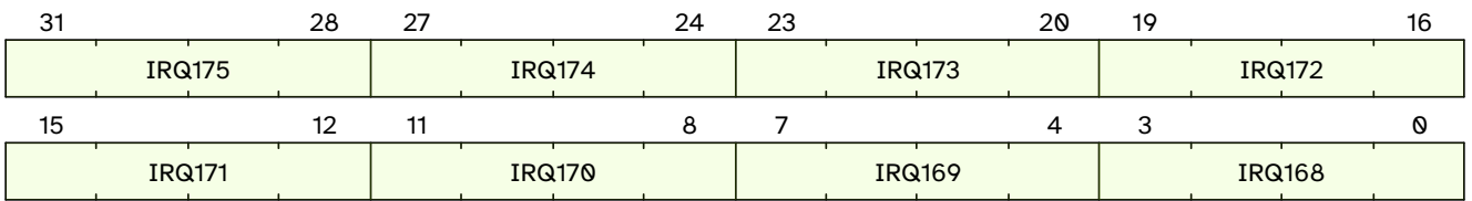
Figure 31. qc.mclcivl21 format
