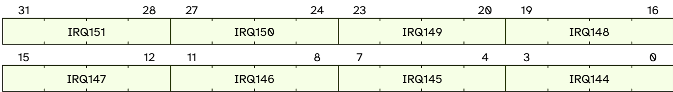
Figure 28. qc.mclcivl18 format
