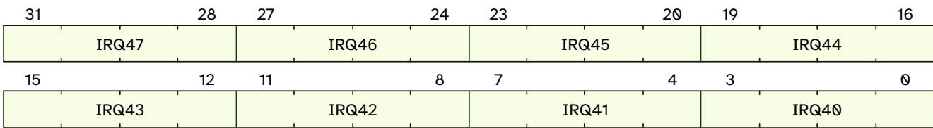
Figure 15. qc.mclivil05 format
