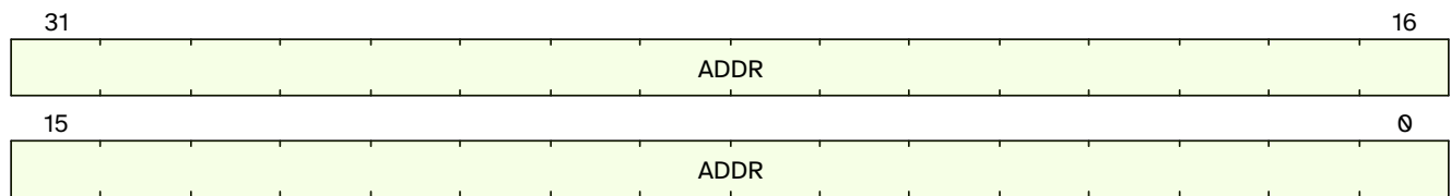
Figure 61. qc.mwpstartaddr2 format
