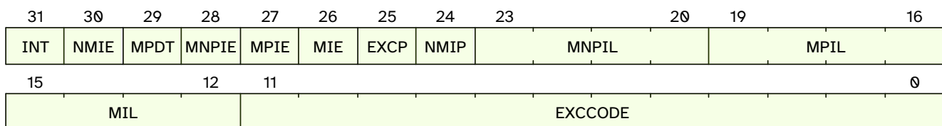
Figure 1. qc.mcause format
