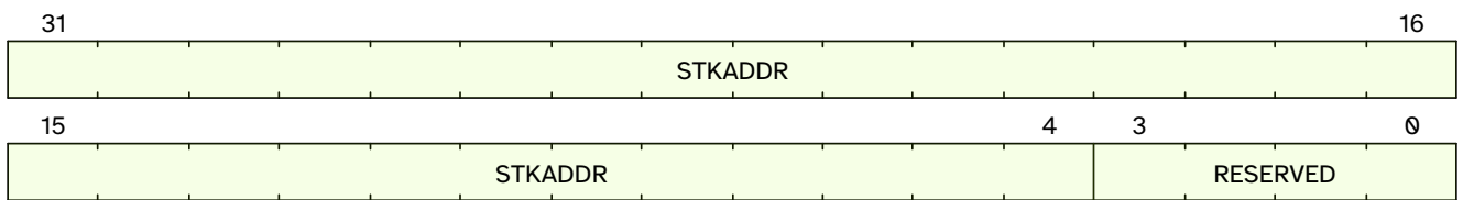
Figure 52. qc.mstkbottomaddr format
