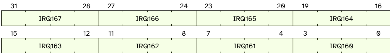
Figure 30. qc.mclcivl20 format
