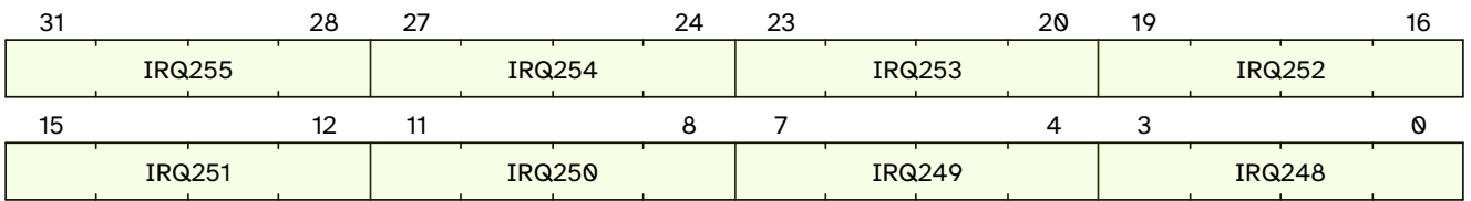
Figure 41. qc.mclcivl31 format
