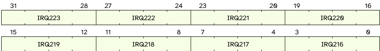
Figure 37. qc.mclcivl27 format
