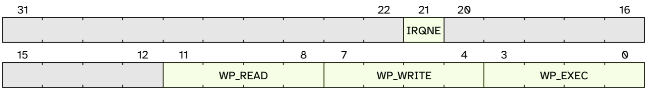
Figure 50. qc.mmcr format
