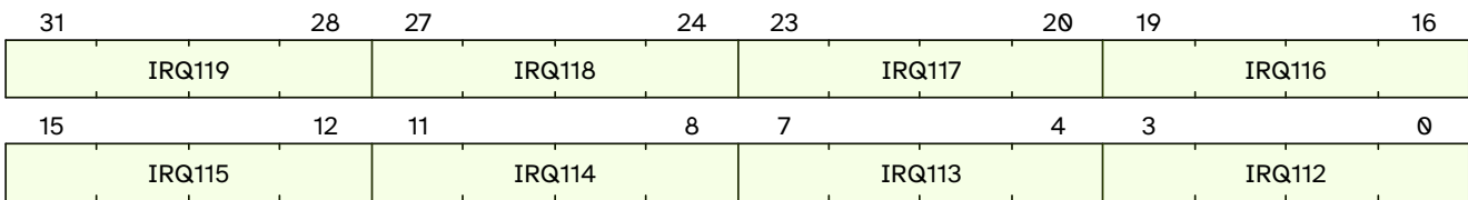
Figure 24. qc.mclcivl14 format
