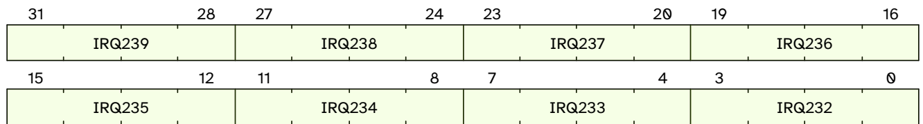
Figure 39. qc.mclivil29 format
