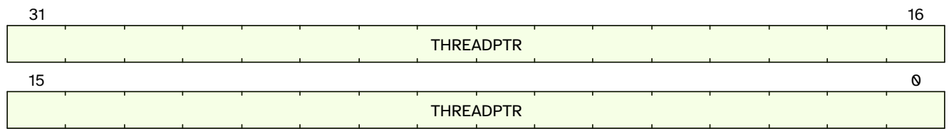
Figure 54. qc.mthreadptr format
