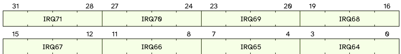
Figure 18. qc.mclcivl08 format
