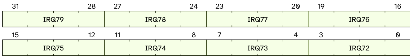
Figure 19. qc.mclcivl09 format
