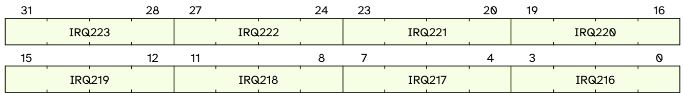
Figure 37. qc.mclcivl27 format
