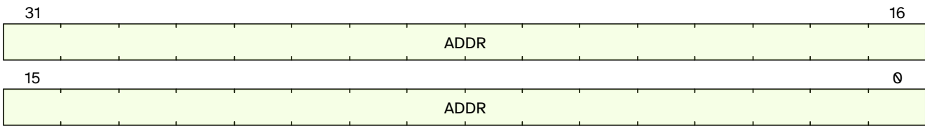
Figure 55. qc.mwpendaddr0 format
