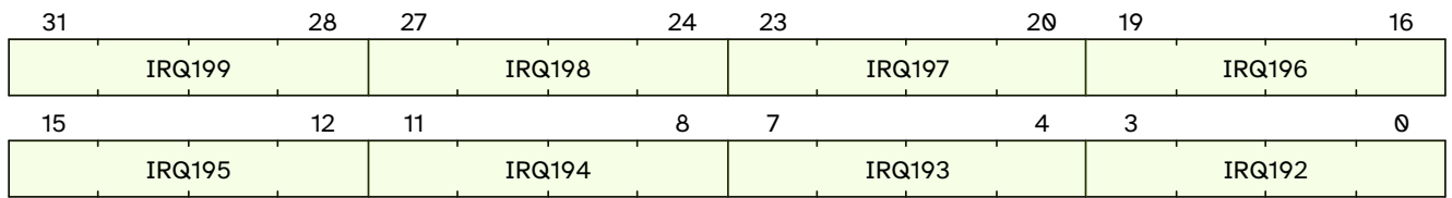
Figure 34. qc.mclcivl24 format
