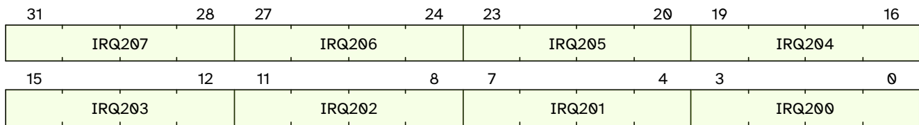
Figure 35. qc.mclivil25 format
