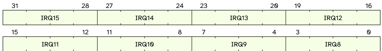
Figure 11. qc.mclcivl01 format
