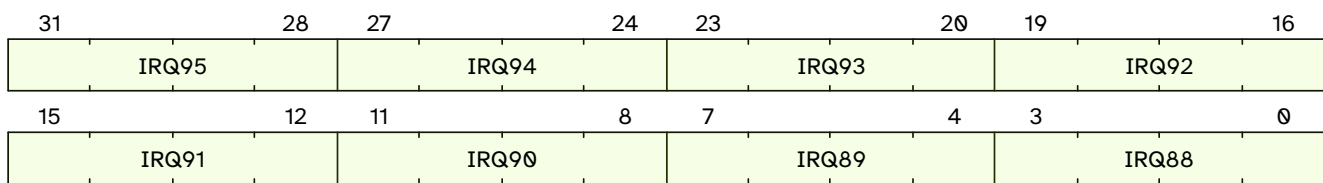
Figure 21. qc.mclivil11 format
