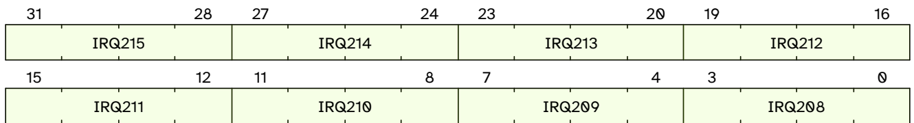
Figure 36. qc.mclcivl26 format
