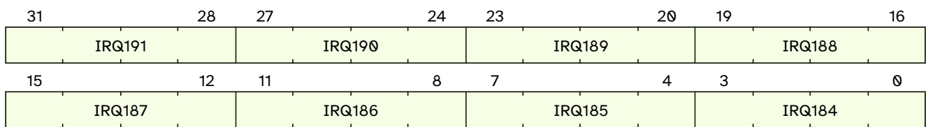
Figure 33. qc.mclivil23 format
