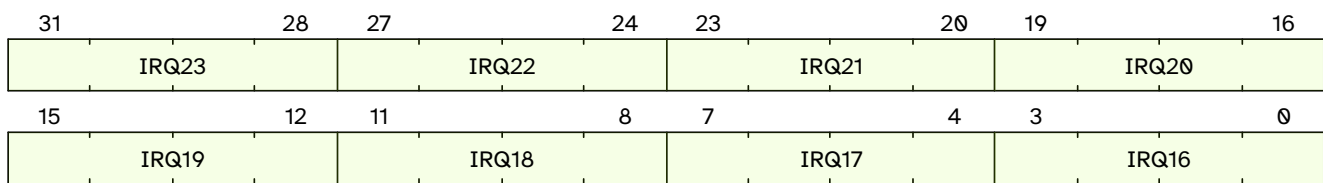
Figure 12. qc.mclivil02 format
