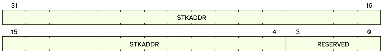
Figure 52. qc.mstkbottomaddr format
