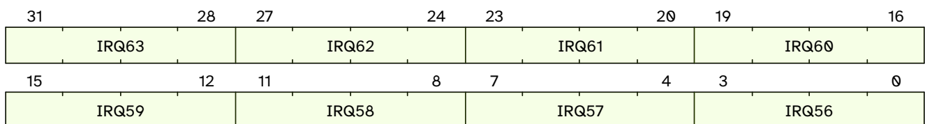
Figure 17. qc.mclcivl07 format
