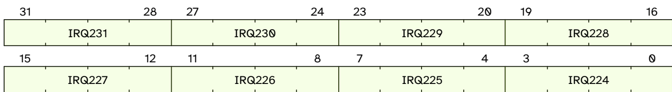
Figure 38. qc.mclivil28 format
