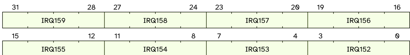
Figure 29. qc.mclivil19 format
