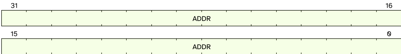
Figure 59. qc.mwpstartaddr0 format
