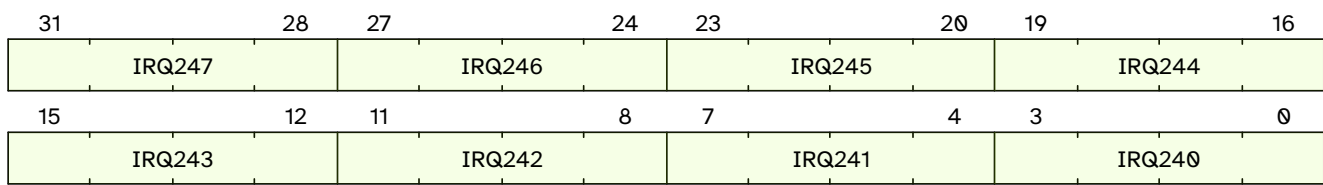
Figure 40. qc.mclivil30 format
