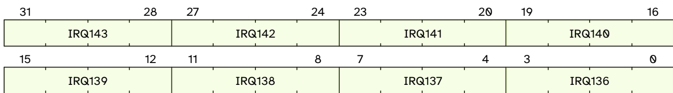
Figure 27. qc.mclivil17 format
