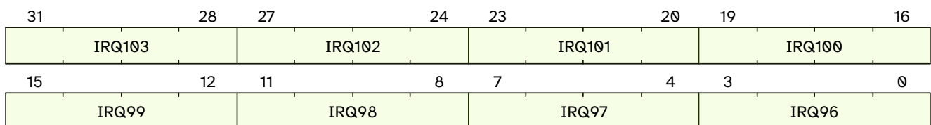
Figure 22. qc.mclcivl12 format
