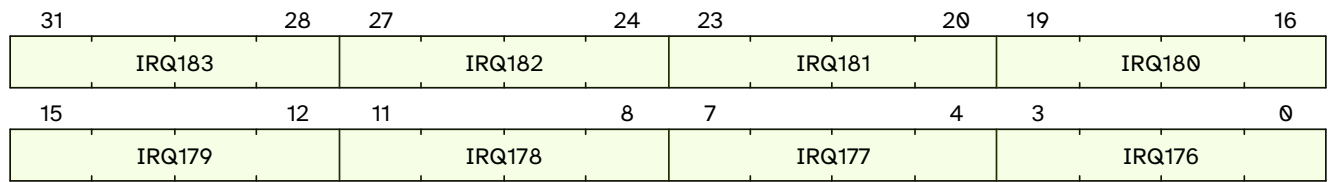
Figure 32. qc.mclivil22 format
