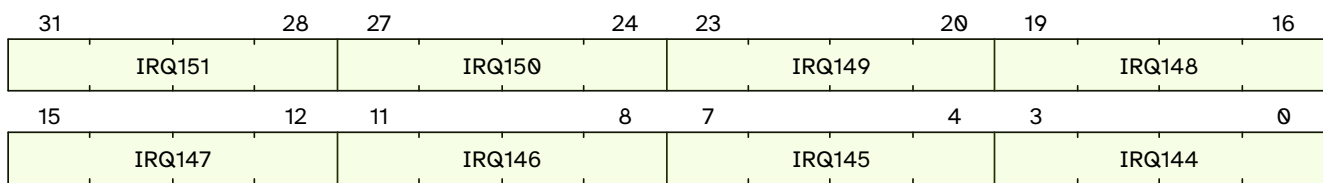
Figure 28. qc.mclivil18 format
