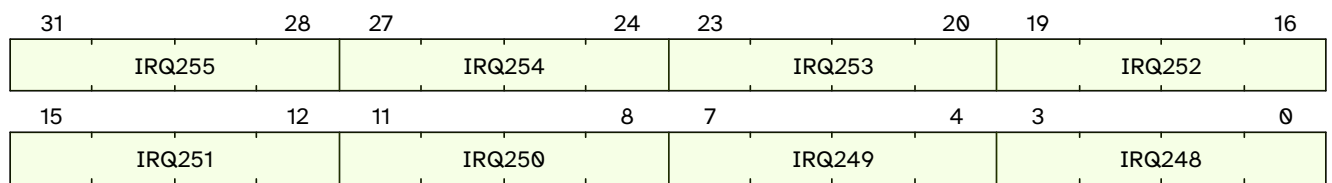
Figure 41. qc.mclivil31 format
