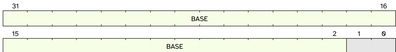
Figure 51. qc.mntvec format
