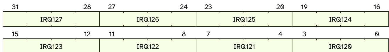
Figure 25. qc.mclivil15 format
