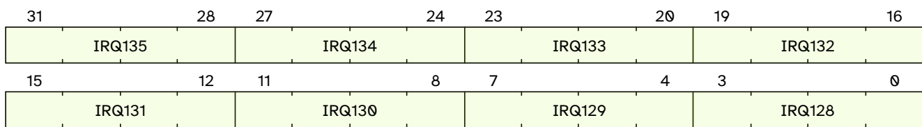
Figure 26. qc.mclivil16 format
