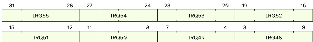
Figure 16. qc.mclivil06 format
