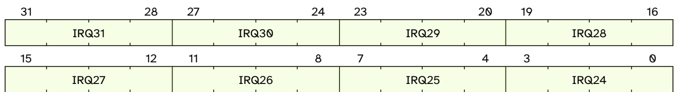
Figure 13. qc.mclivil03 format
