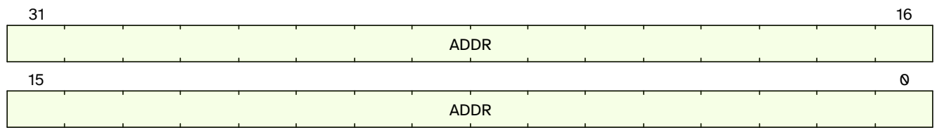
Figure 60. qc.mwpstartaddr1 format
