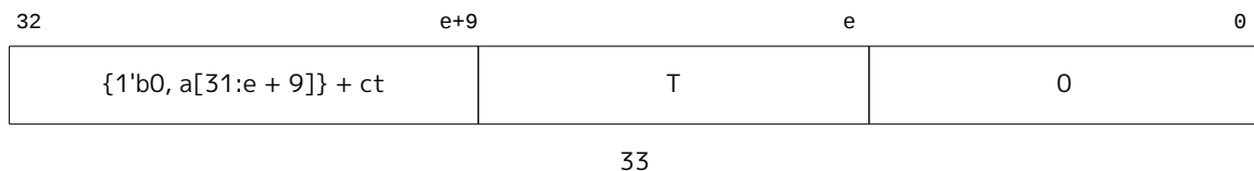
Figure 16. Decoding of the XLEN+1 wide top (t) bound
