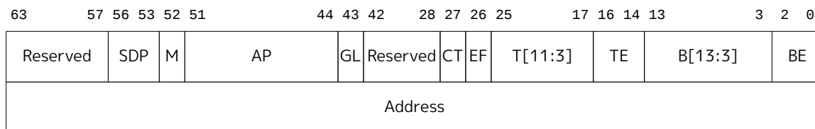
Figure 8. Capability encoding for RV64LYmw14rc1ps
