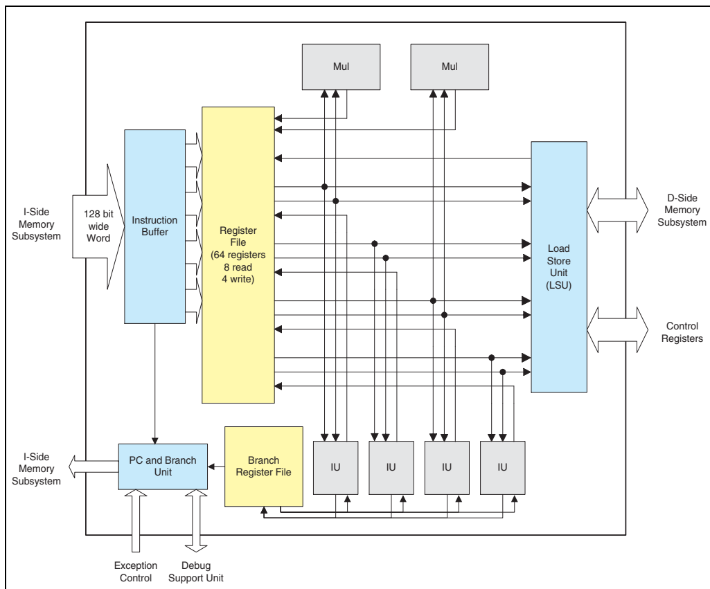
Figure 2: ST220 cluster
