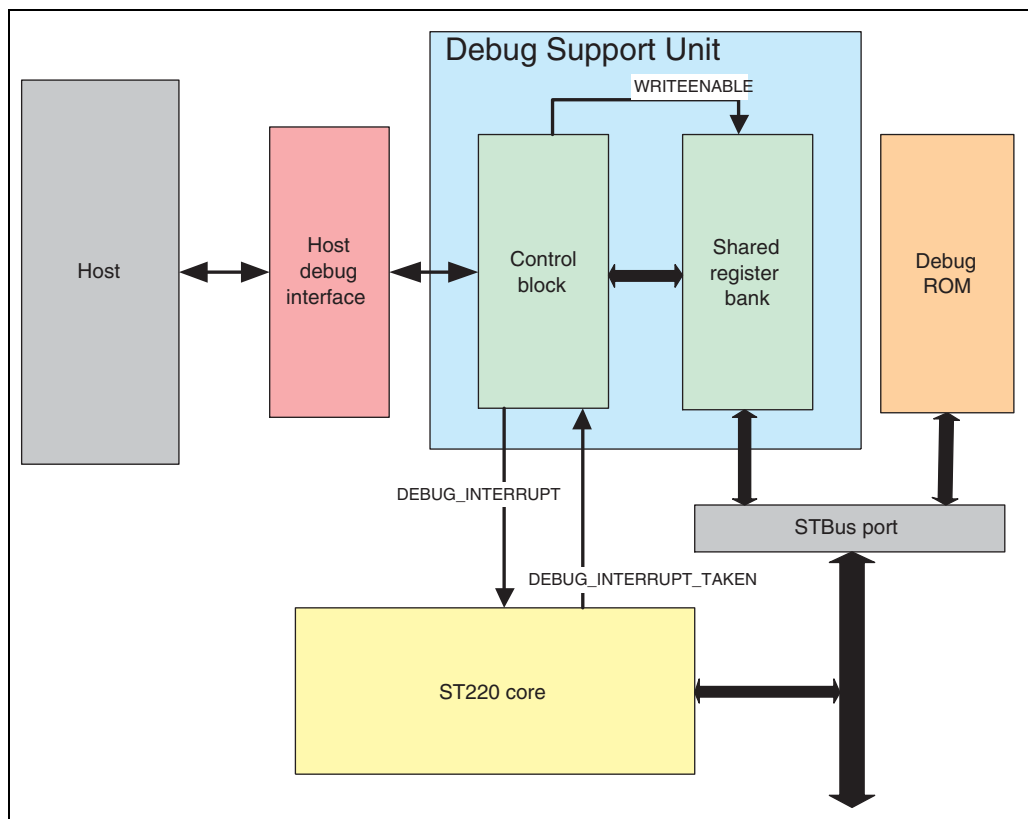
Figure 9: DSU architecture
