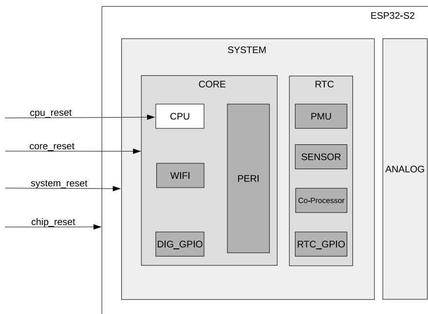
Figure 6-1. System Reset
