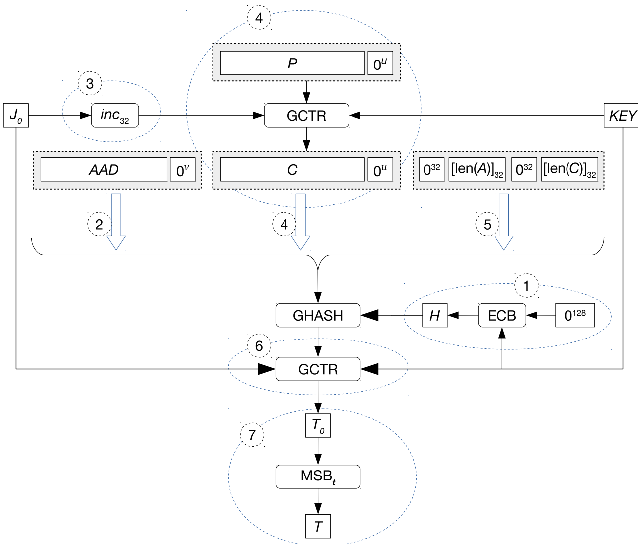
Figure 17-1. GCM Encryption Process
