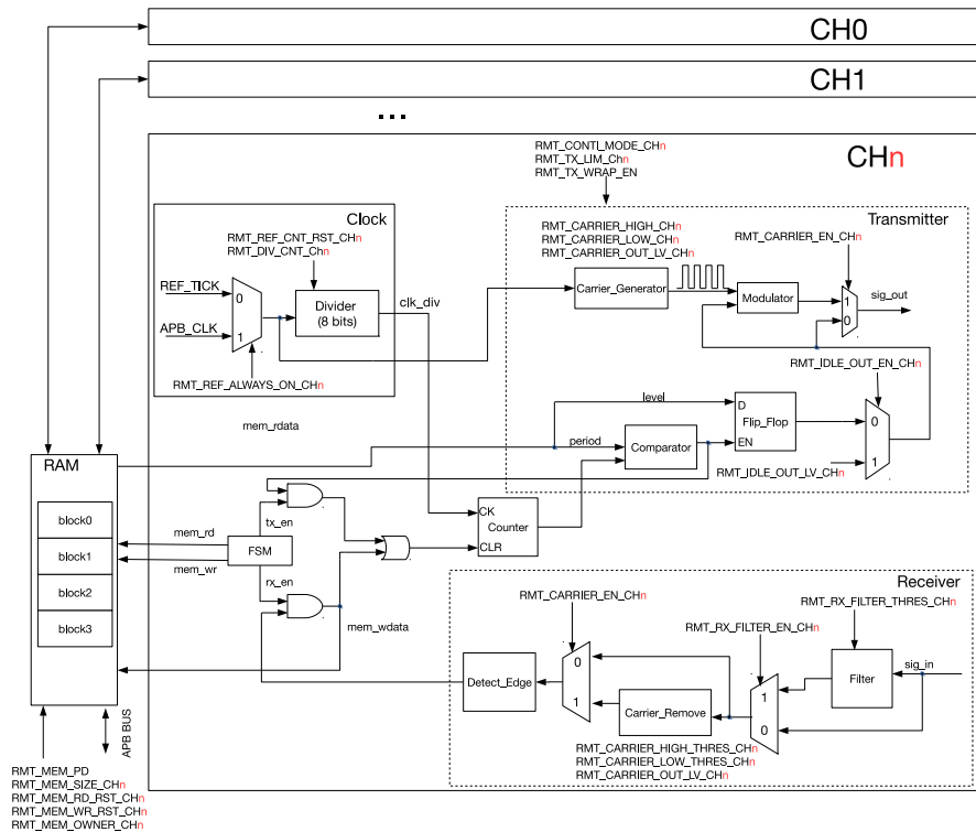
Figure 31-1. RMT Architecture
