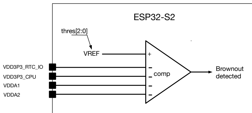
Figure 9-9. Brown-out detector
