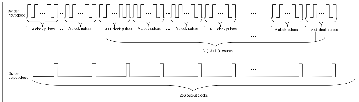
Figure 30-3. LED_PWM Divider
