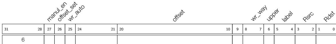
Figure 1-10. Instruction Type - ST
