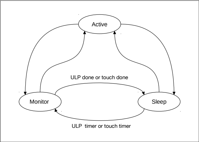
Figure 9-10. RTC States Transition
