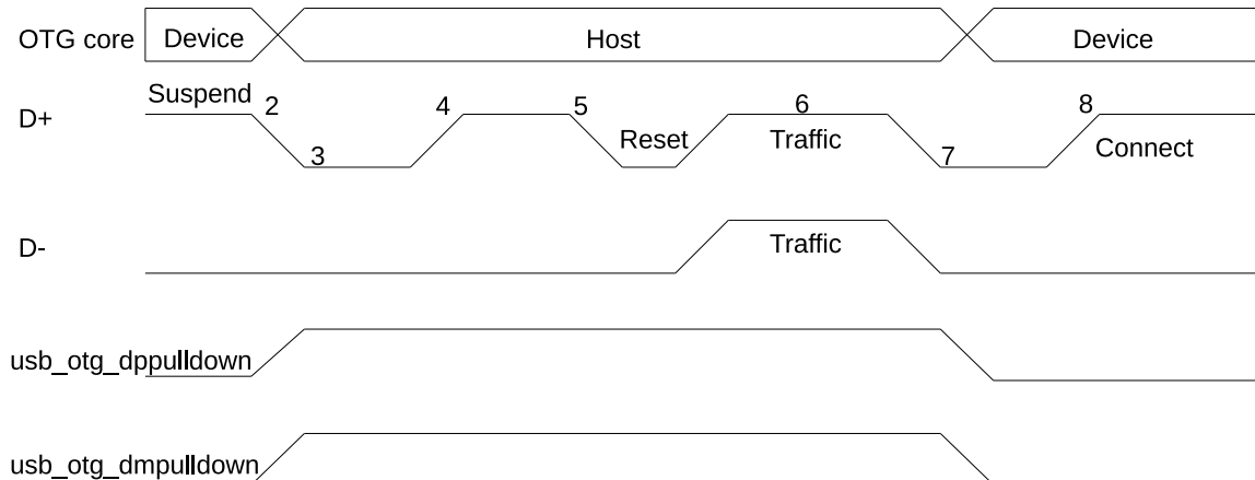
Figure 28-10. B-Device HNP
