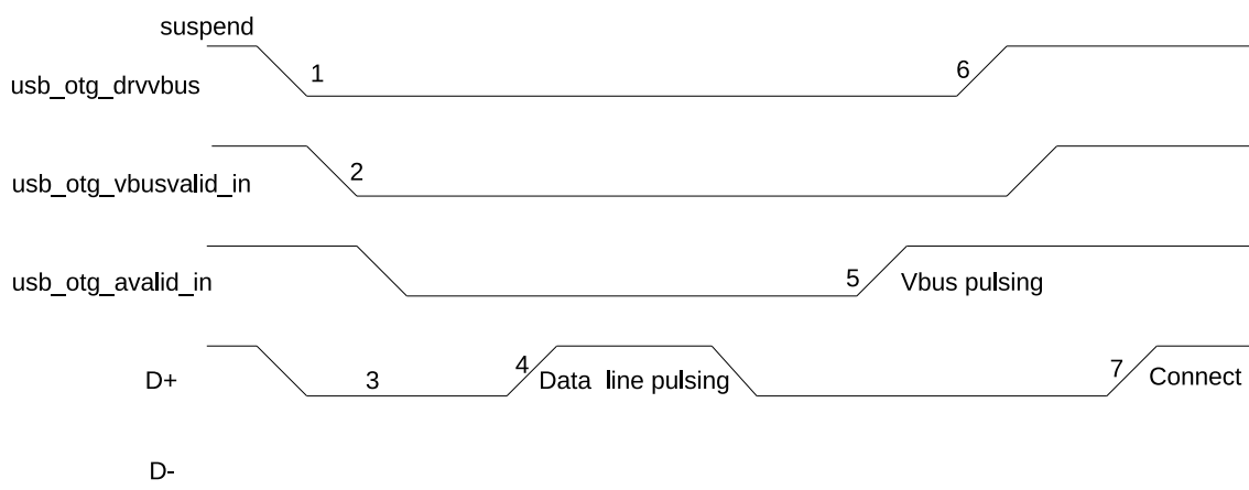
Figure 28-7. A-Device SRP
