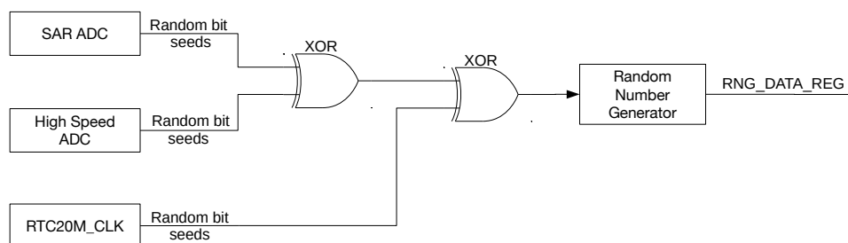
Figure 22-1. Noise Source
