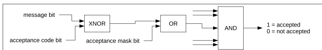
Figure 29-7. Acceptance Filter
