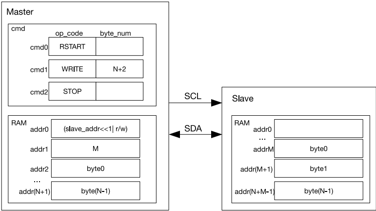
Figure 25-7. An I2C Master Writing Address M in the RAM to an I2C Slave with a 7-bit Address
