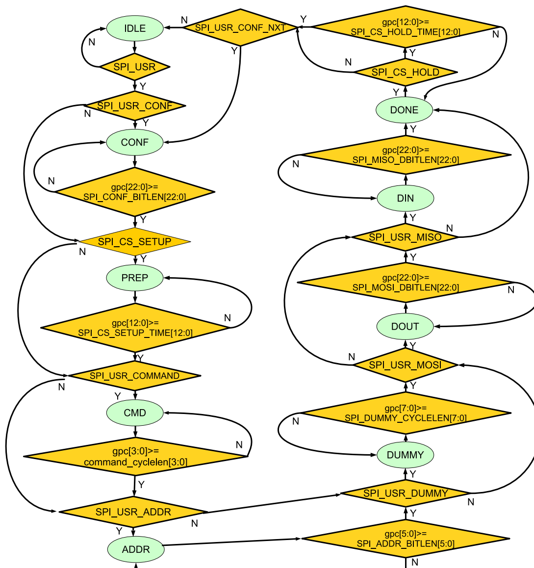
Figure 24-3. GP-SPI2 State Flow in Master Mode
