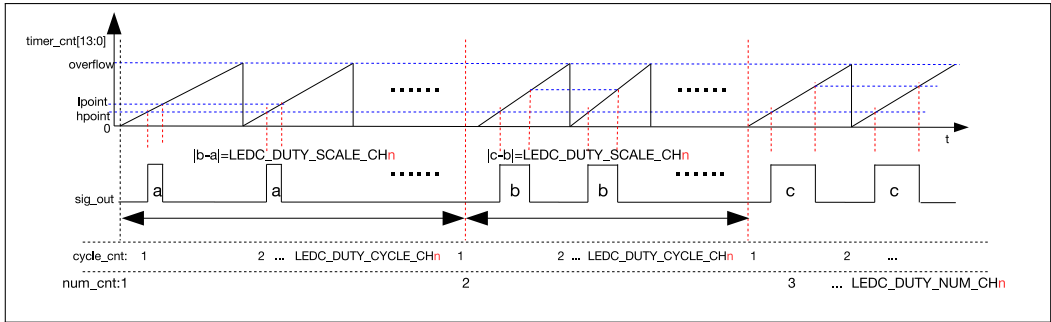
Figure 30-5. Output Signal Diagram of Fading Duty Cycle
