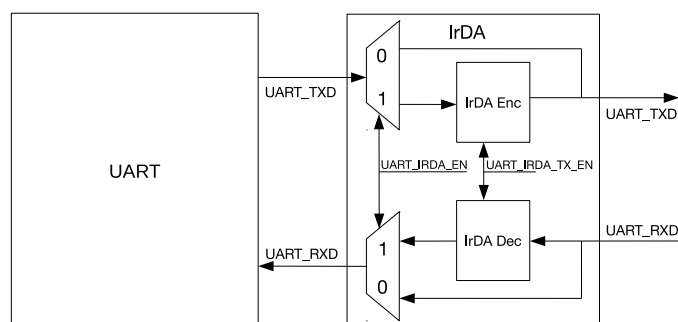
Figure 23-9. IrDA Encoding and Decoding Diagram
