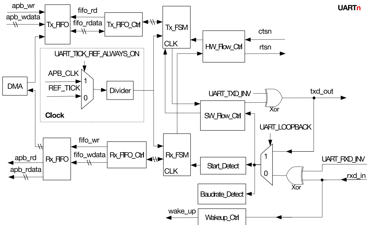
Figure 23-1. UART Structure
